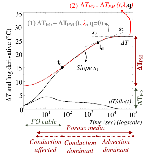
Figure 1. Principle of the interpretation of thermal response curves (represented by the black line) collected during ADTS measurements (following Simon et al. 2021). The black dotted line corresponds to the log-derivative of temperature. First, the temperature rise \Delta T_{PM} during the conduction-dominant period, for t_c < t < t_d , can be reproduced using the Moving Instantaneous Line Source (MILS) model considering q = 0 m/s (gray line). Then, \Delta T_{PM} during both conduction-dominant and the advection-dominant periods can be reproduced using the MILS model considering the groundwater flow (red line).
