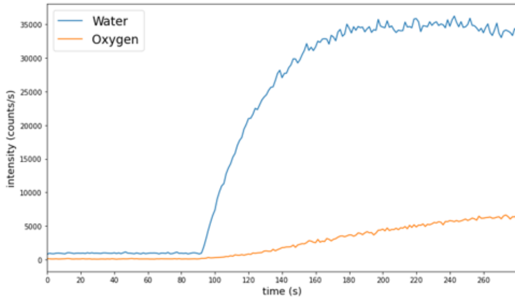
Fig. 2. Temporal evolution of the intensity (in counts/s) measured by the mass spectrometer for water (blue curve) and oxygen (orange curve). This second scenario is associated with 5% of molecular hydrogen in the mixture.
