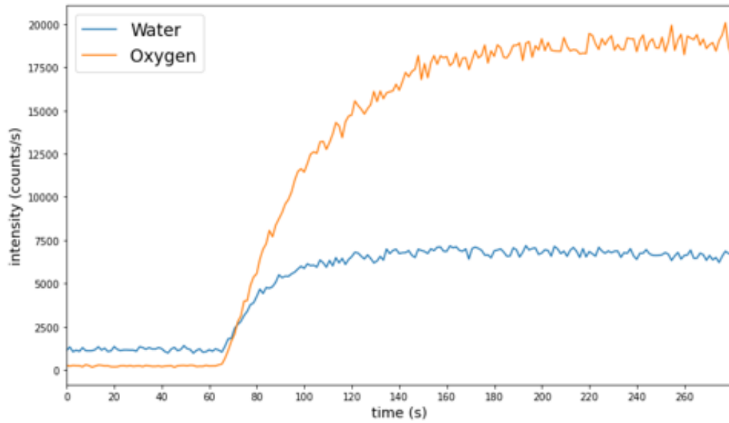
Fig. 1. Temporal evolution of the intensity (in counts/s) measured by the mass spectrometer for water (blue curve) and oxygen (orange curve). This first scenario is associated with 0.5% of molecular hydrogen in the mixture.
