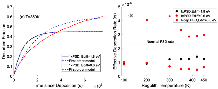
Fig. 26 Simulated desorption of alkali adsorbates from a porous soil. (a) Desorbed versus initially adsorbed particles as a function of time for soil temperature T = 350\text{ K} . Adsorbates that are not on illuminated grains are trapped unless high mobility is considered; (b) Effective photodesorption rate for constant and temperature-dependent yield and different mobilities. Mobility in these simulations is defined by a barrier for surface diffusion ( E_{\text{diff}} ). Figure from Sarantos and Tsavachidis (2020)
