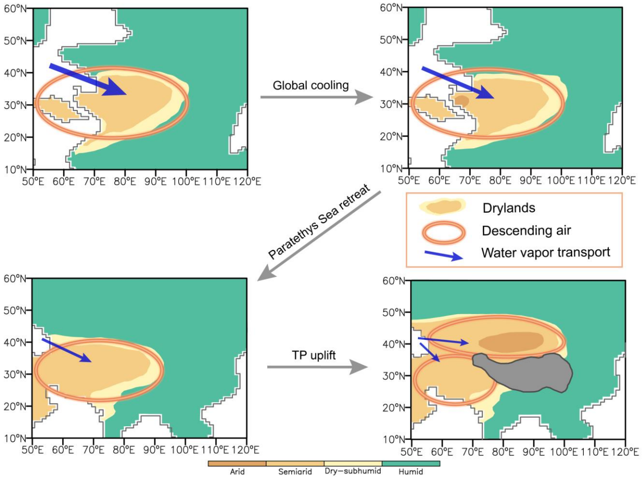
Figure 4. Cartoon illustrating the impacts from global cooling, Paratethys Sea retreat and Tibetan Plateau (TP) uplift on Asian drylands. The decreased atmospheric CO 2 concentration and the retreated Paratethys Sea weaken the water vapor transport and promote aridification in inland Asia, but they only slightly change the latitudinal position of dryland. The uplift of the TP makes Asian drylands move northward, concentrate in narrow latitudinal bands and increase in intensity mainly through intensification of descending air in the north of the TP. Note that the water vapor transport from the Indian and Pacific Oceans is not shown.
