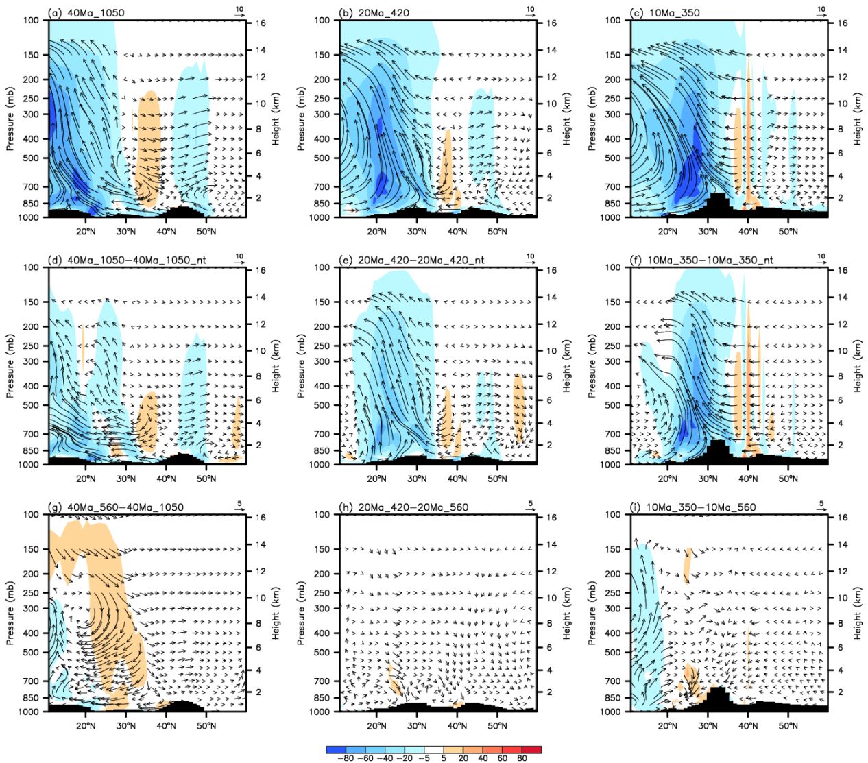
Figure 3. Differences in simulated summer (May to September) meridionally averaged ( 70\text{--}90^\circ\text{E} ) vertical velocity (shaded, units: \text{hPa day}^{-1} ) and wind circulation due to the uplifted Asian topography (d-f) and decreased atmospheric \text{CO}_2 concentration (g-i) under late Eocene, early Miocene and late Miocene boundary conditions. Upward motion is negative and downward motion is positive. Vectors are vertical velocity (units: \text{hPa day}^{-1} ) versus meridional wind (units: \text{m s}^{-1} ). The black shaded regions denote the topography.
