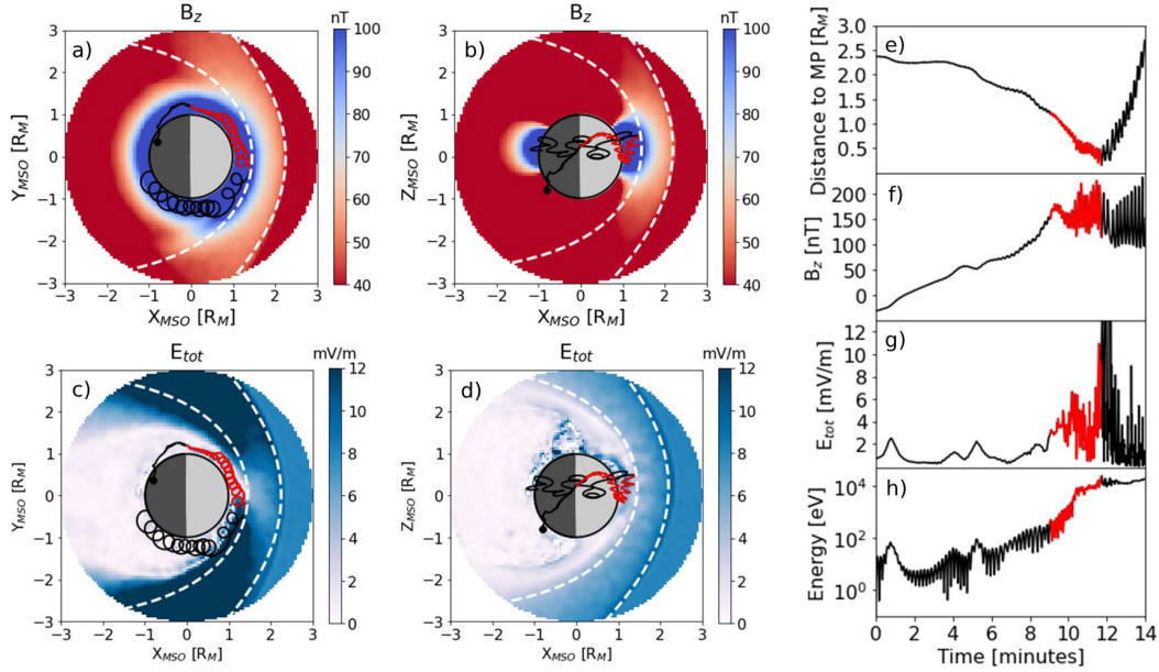
Figure 3. Example test-particle trajectory of a Mg^+ ion from the LIZE model in the (a,c) MSO XY-plane and the (b,d) XZ-plane. Also shown is the magnetic field component B_z (a,b) and the total electric field E_{tot} (c,d) from the LathyS simulation. (e) shows the distance of the Mg^+ ion from the planet, (f) the time-evolution of B_z experienced by the Mg^+ ion, (f) the total electric field and (h) the ion energy. The part of the test-particle trajectory highlighted in red indicates a short time period when the ion energy increases from \sim 100 eV to >10 keV. The white dashed curves in (a-d) show the approximate location of the magnetopause and bow shock calculated from Winslow et al. (2013).
