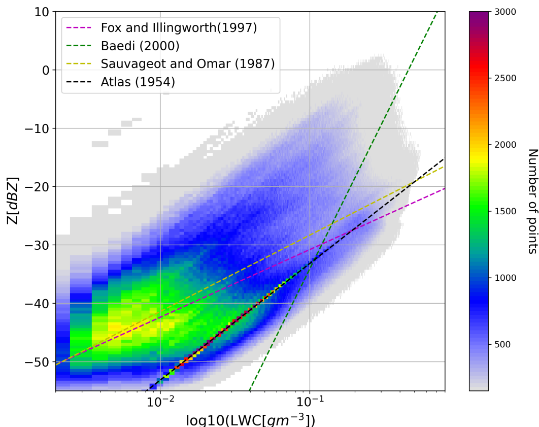
Figure 13. Retrieved LWC as a function of radar reflectivity Z for 39 cloudy days, with reference plot of various empirical relation for different cloud types.
