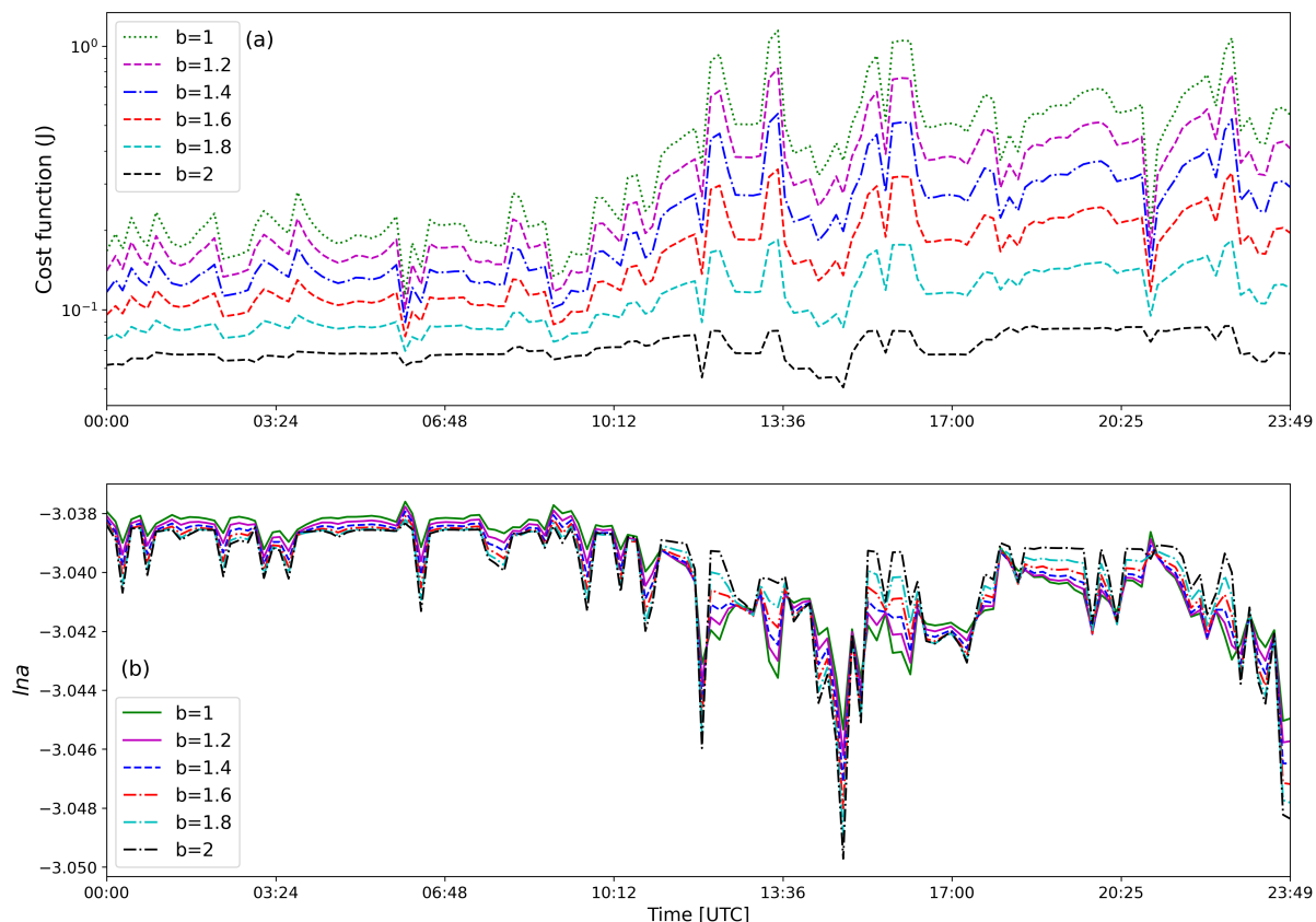
Figure 6. (a) Cost function and (b) Retrieved \ln a for different b values
