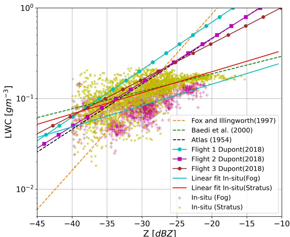
Figure 11. Scatter plot for relation between LWC measured from CDP with radar reflectivity from cloud radar, compared with available literature
