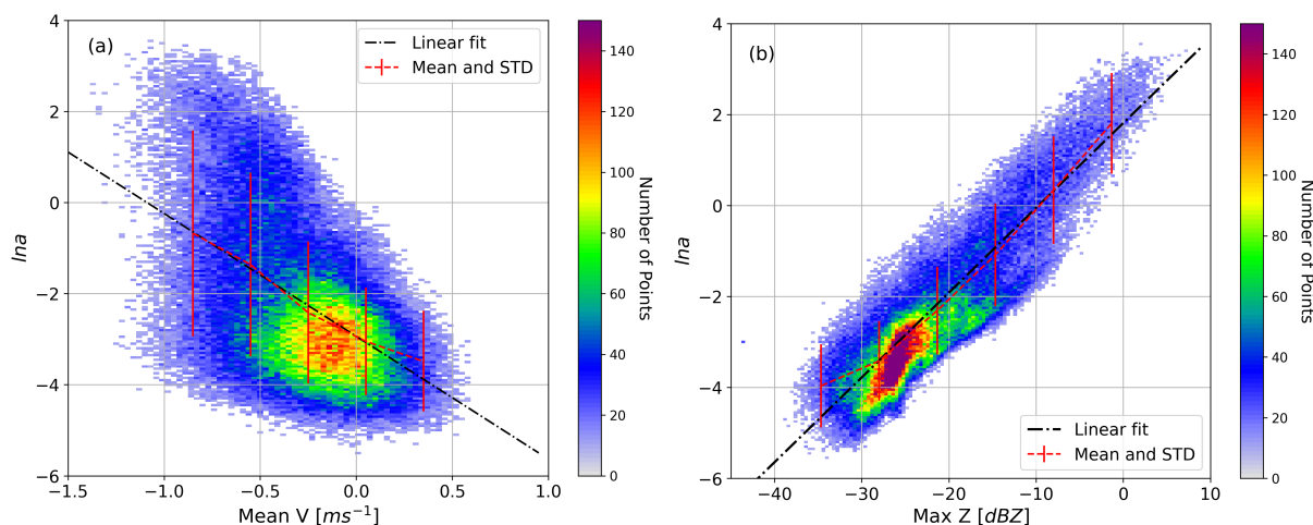
Figure 14. Correlation of (a) Mean velocity versus lna and (b) Maximum reflectivity versus lna for cloud profiles, where color bar indicates the number of profiles
