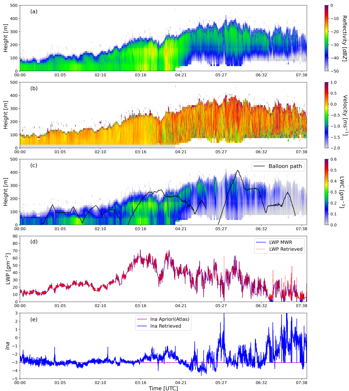
Figure 7. (a) Radar reflectivity Z (b) Vertical velocity (c) Retrieved LWC, (d) LWP and (e) Retrieved \ln a for 09 February 2020 case at SOFOG-3D super-site. Tethered balloon trajectory over retrieved LWC is shown in black line.
