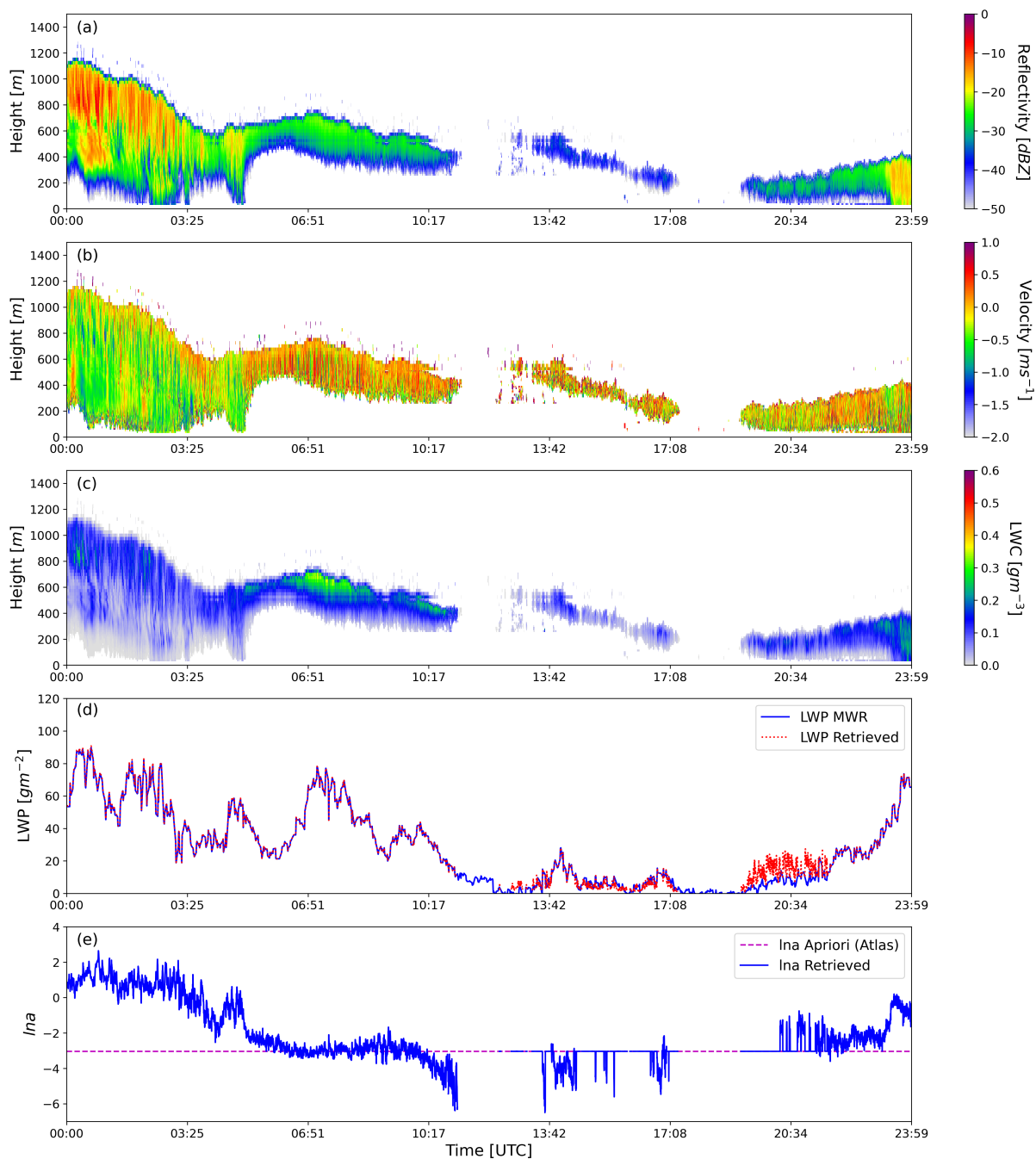
Figure 2. (a) Radar reflectivity (b) Vertical velocity (c) Retrieved LWC, (d) LWP and (e) Retrieved lna for 05 February 2019 case at SIRTa.
