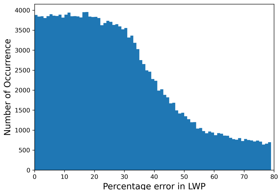
Figure 16. Percentage error in retrieved LWP with respect to LWP measured by MWR at SIRT A.
