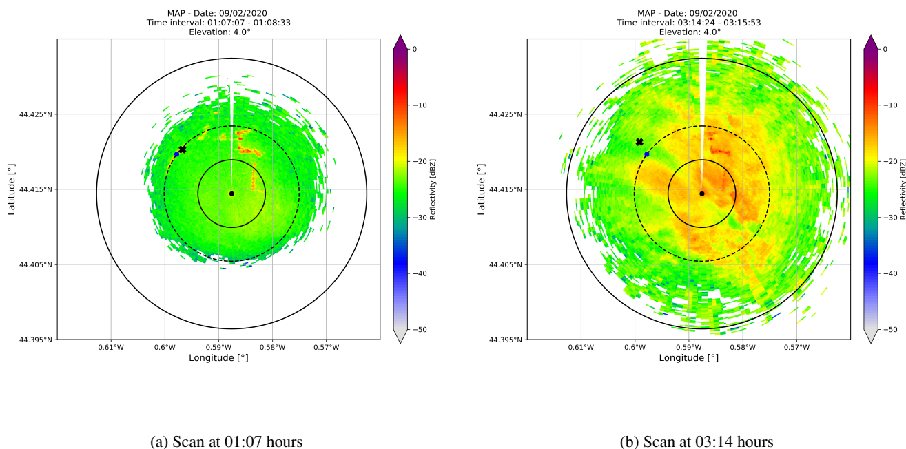
Figure 9. Scans of BASTA-mini collected for fog at 4° elevation angle. The vertically pointing radar shown as blue dot was located 1 km away from the scanning radar and cross represents the location of balloon.
