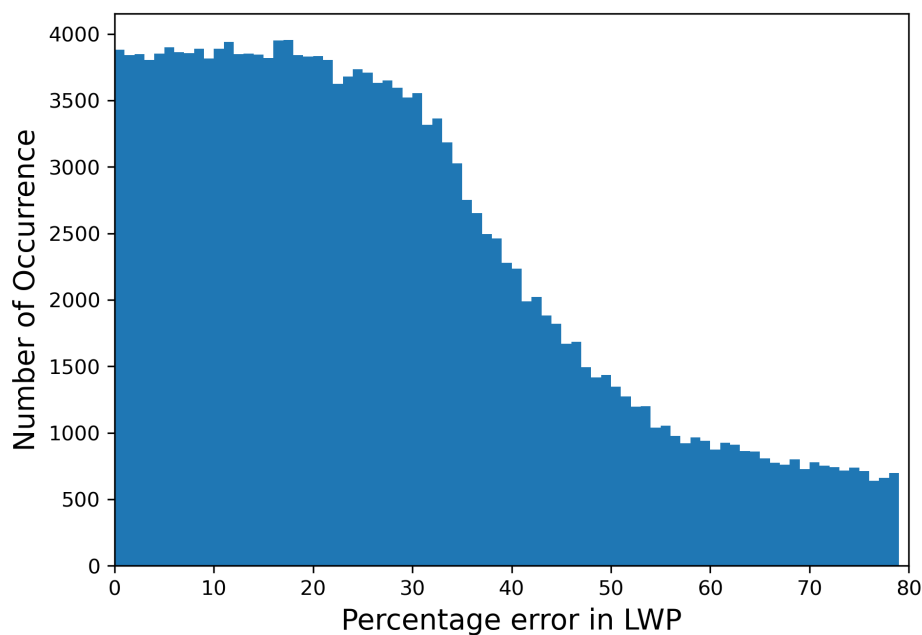
Figure 16. Percentage error in retrieved LWP with respect to LWP measured by MWR at SIRT A.
