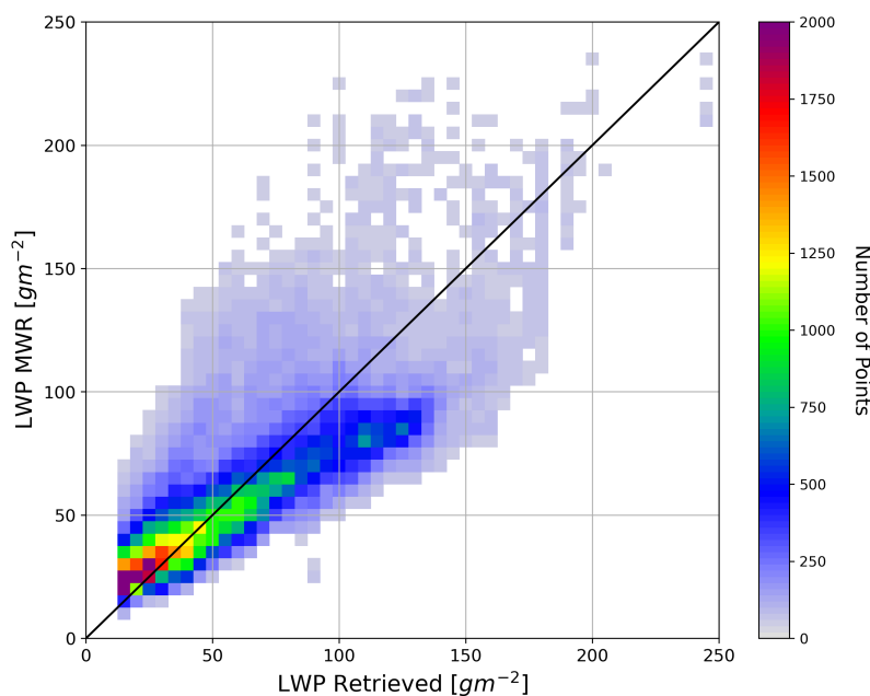
Figure 15. Comparison of retrieved LWP with LWP retrieved by HATPRO, where the black line represents the exact match of LWP for given profile.
