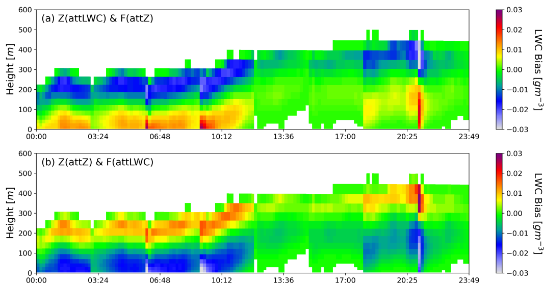
Figure 5. Bias in retrieved LWC with respect to true LWC for different attenuation consideration in the retrieval algorithm
