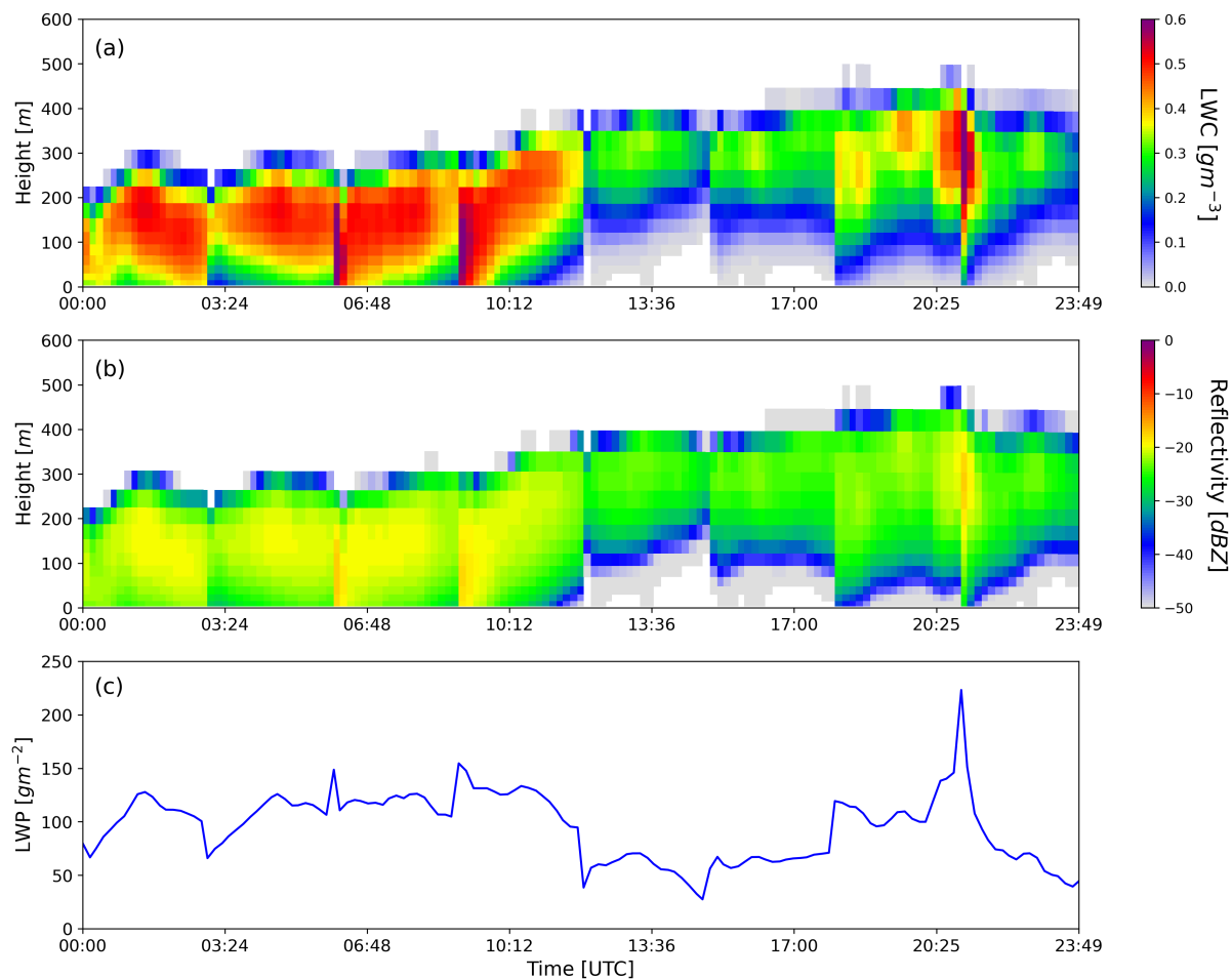
Figure 4. Simulations from AROME model for 16 November 2018 showing (a) True LWC in gm^{-3} , (b) Synthetic reflectivity and (c) LWP.
