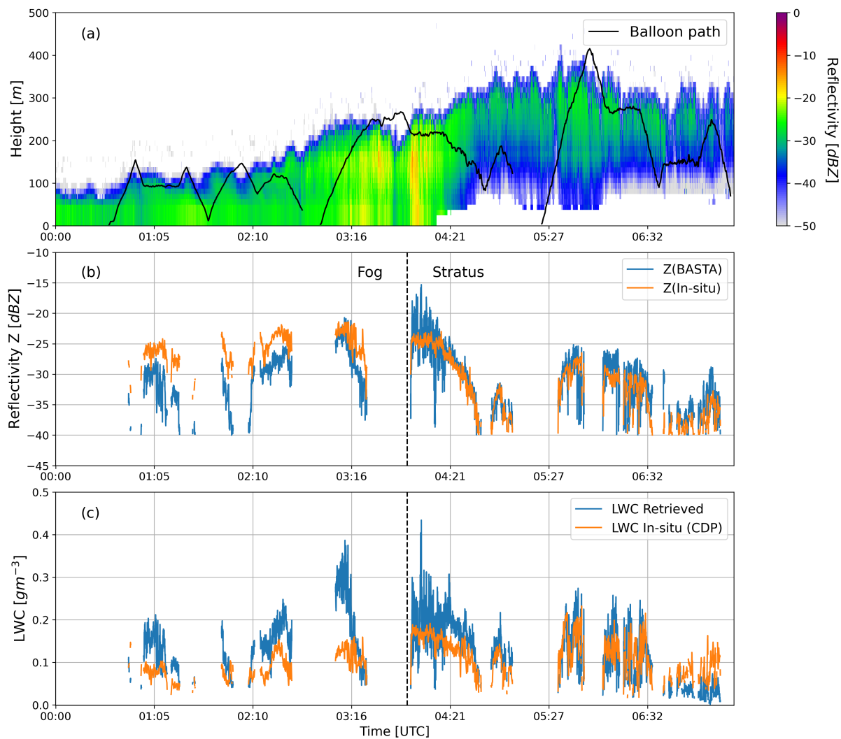
Figure 8. (a) Radar reflectivity and balloon path (b) Comparison of radar reflectivity with reflectivity calculated from CDP using DSD (c) Comparison of retrieved LWC with in-situ LWC
