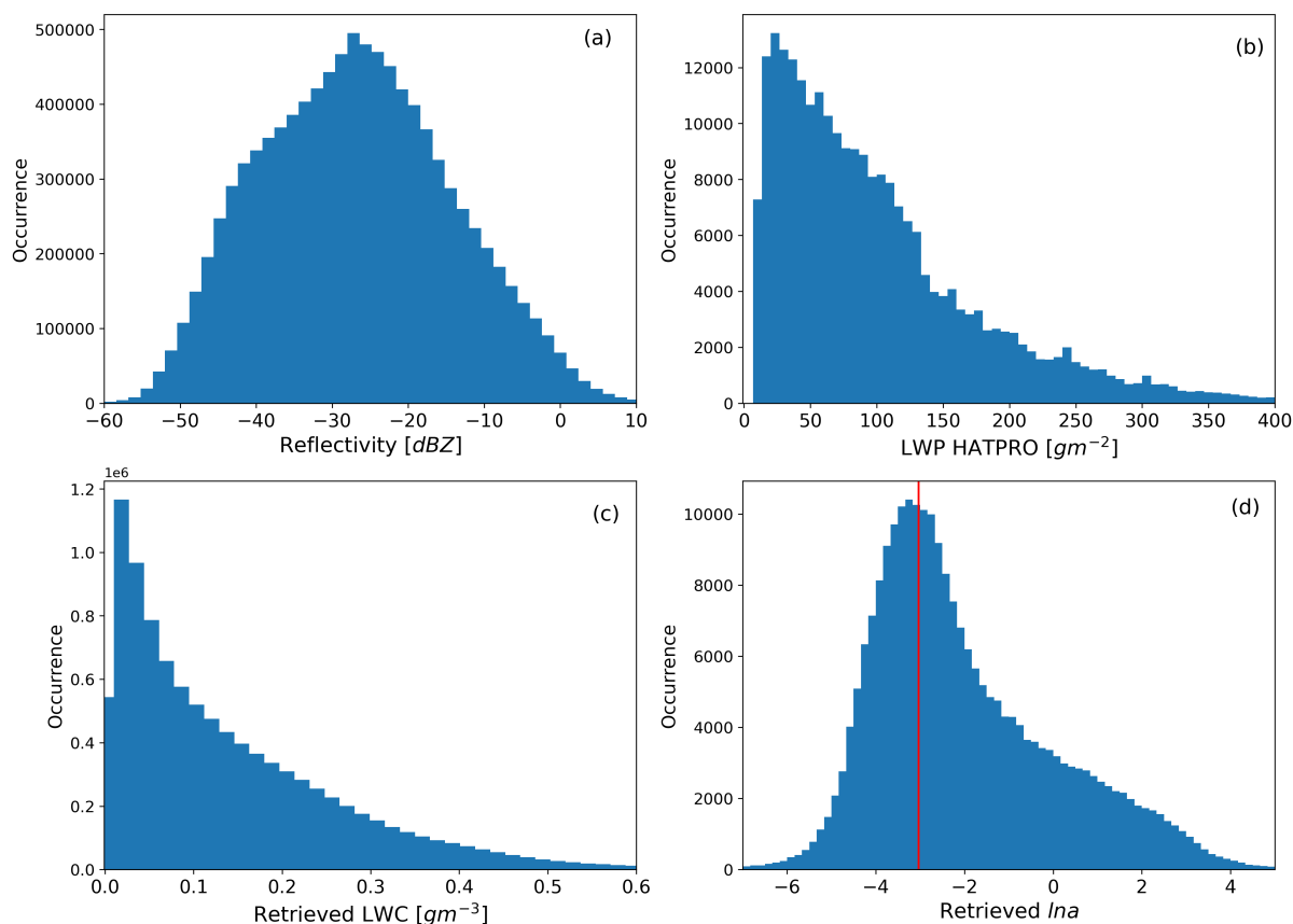
Figure 12. Histogram of (a) Radar reflectivity(Z) (b) LWP from MWR (c) Retrieved LWC (d) Retrieved lna for 39 cloudy days, and the red line in lna histogram indicates the a priori of lna from table 1
