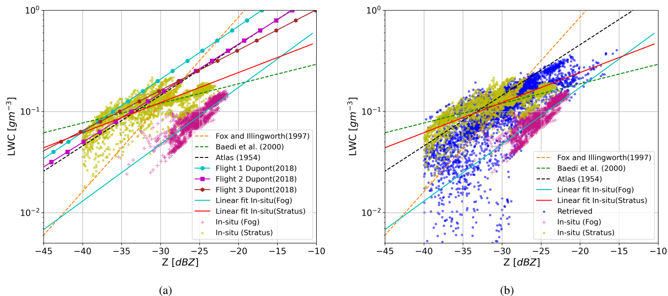
Figure 10. Comparison of in-situ LWC and radar reflectivity relation with (a) available literature for fog and clouds, (b) retrieved LWC and BASTA radar reflectivity relation.
