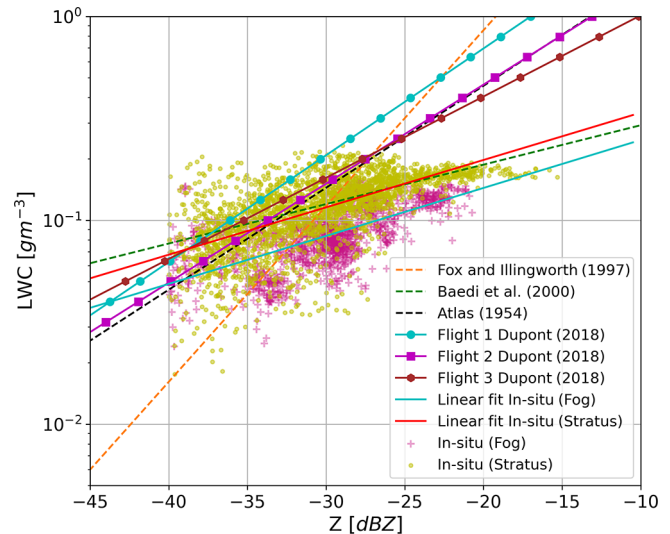
Figure 10. Scatterplot for the relation between LWC measured from CDP with radar reflectivity from cloud radar, compared with the available literature. In situ measurements are separated for fog and stratus clouds where magenta denotes fog, yellow–green (chartreuse) denotes the stratus cloud, and the respective linear fits are also plotted.
