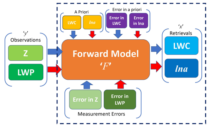
Figure 1. Schematic of LWC retrieval algorithm.
