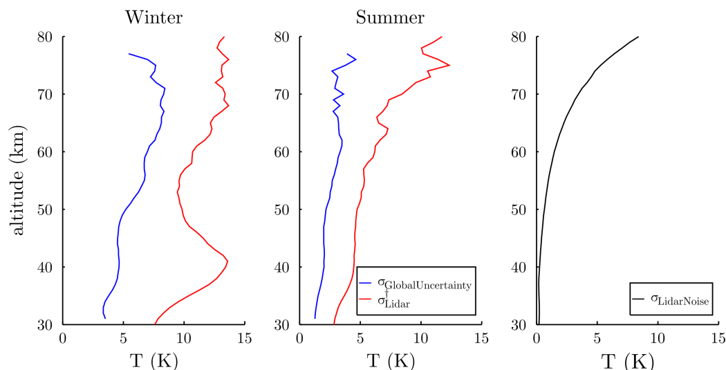
Figure 5. Model uncertainty estimates (blue solid lines) and atmospheric variability observed with the LiDAR (red solid lines) profiles corrected by the LiDAR noise during winter and summer in the 30–80 km altitude range. The median of the LiDAR instrumental errors \sigma_{LiDARNoise} (black solid line) over the altitude is shown as well.
