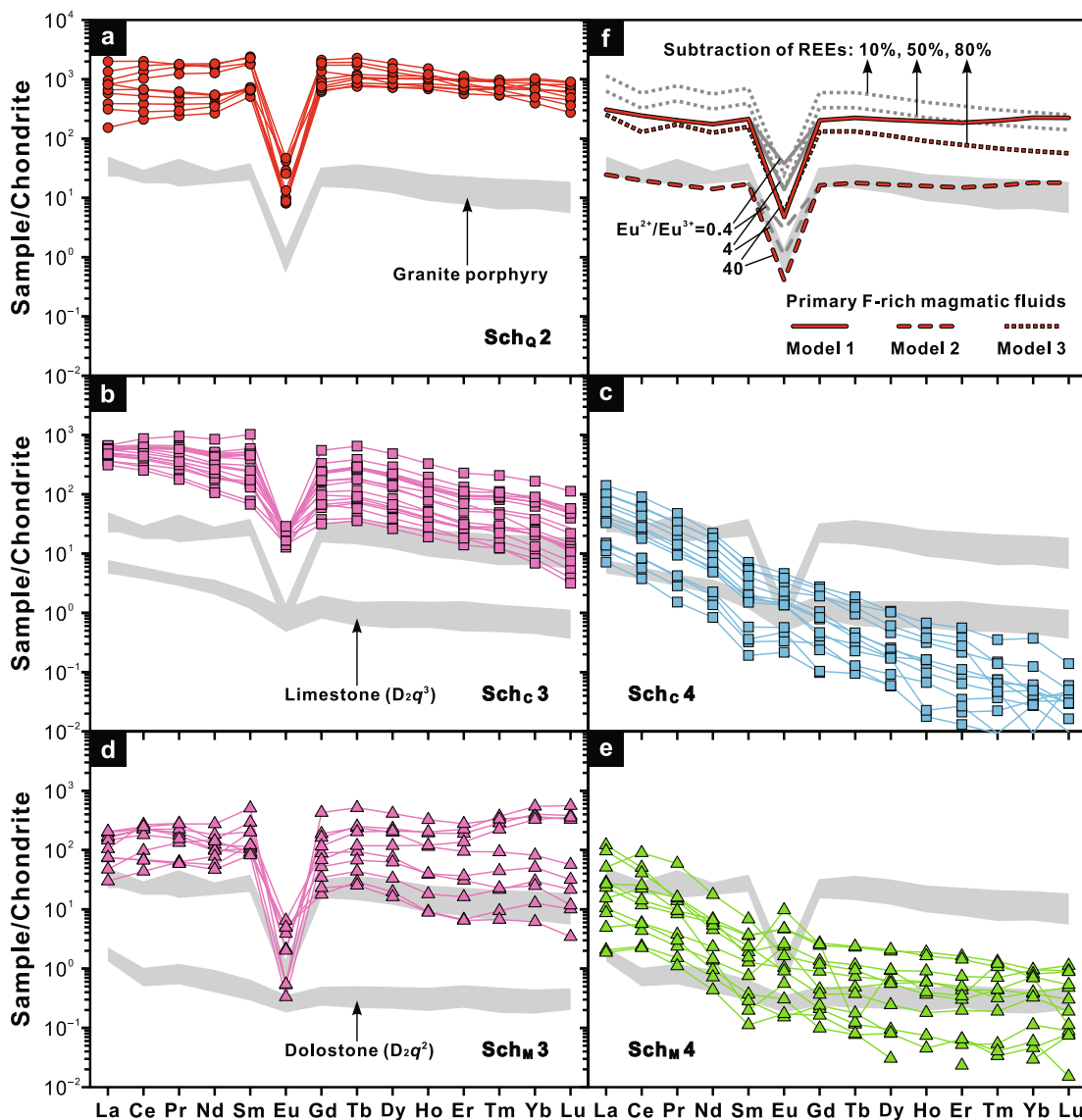
Fig. 11. Chondrite-normalized (Boynnton, 1984) REE patterns of (a–e) different generations of scheelites and (f) model primary F-rich magmatic fluids in the Weijia W skarn deposit. The REE data of granite porphyry and carbonate strata are from Huang et al. (2017) and listed in Supplementary Table S5, respectively. The model 1 and model 2 of primary F-rich magmatic fluids are calculated based on the mean REE compositions of Sch Q 2 and the minimum (model 1) and maximum (model 2) D_{REES}^{Sch/fluid} values from Brugger et al. (2000) with presumed fluid Eu^{2+}/Eu^{3+} ratios of 0.4, 4, and 40. The model 3 of primary F-rich magmatic fluids is calculated based on the mean REE compositions of granitic melts (calculated by subtracting hypothetical proportions of 10%, 50%, and 80% REEs in crystallized accessory minerals from the granite porphyry) and the minimum liquid-liquid D_{REES}^{Fluoride/silicate} values from Veksler et al. (2012). The parameters and calculated results are listed in Supplementary Table S7.
