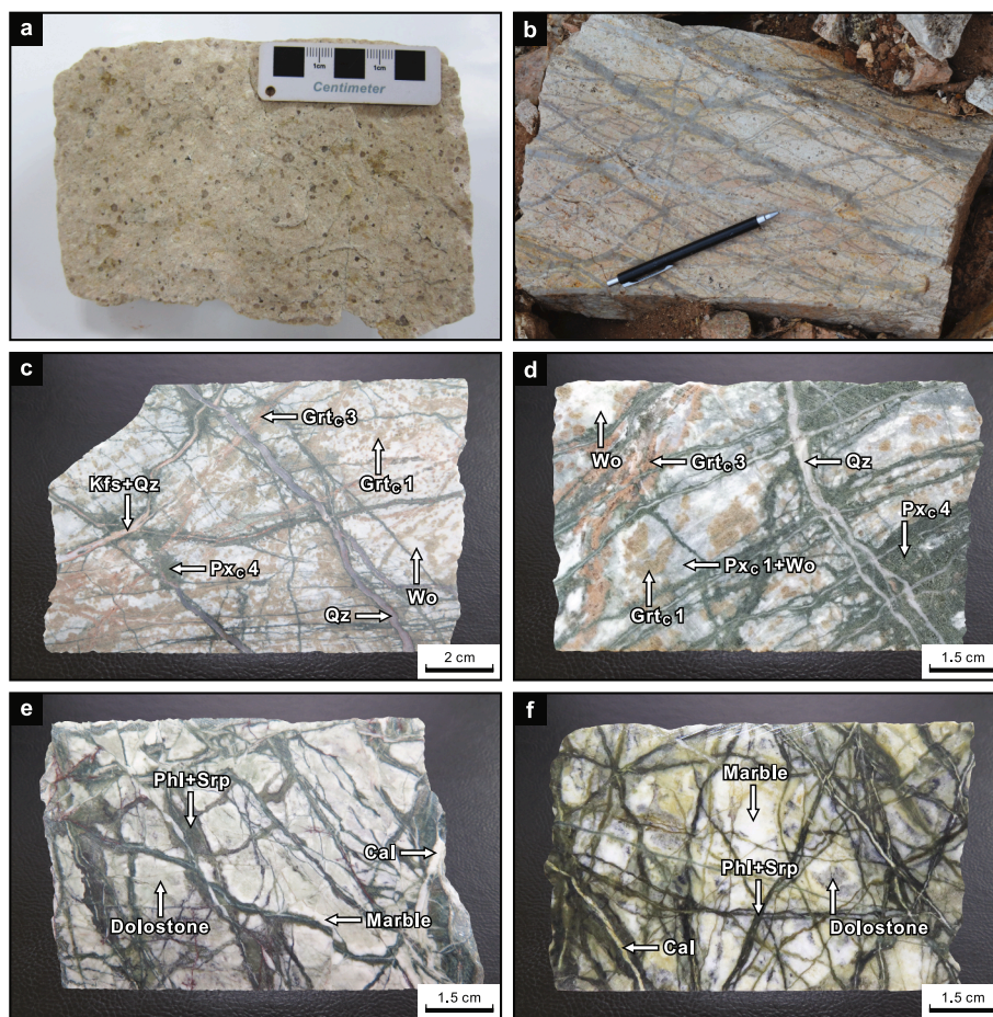
Fig. 3. Representative samples of the (a) granite porphyry and its (b) stockwork quartz veinlets, (c–d) calcic skarn, and (e–f) magnesian skarn from the Weijia W deposit. Mineral abbreviations: Cal = calcite, Grt = garnet, Kfs = K-feldspar, Phl = phlogopite, Px = pyroxene, Qz = quartz, Srp = serpentine, Wo = wollastonite. Subscripts C and M represent calcic and magnesian skarns, respectively, Arabic numerals denote paragenetic stages.
