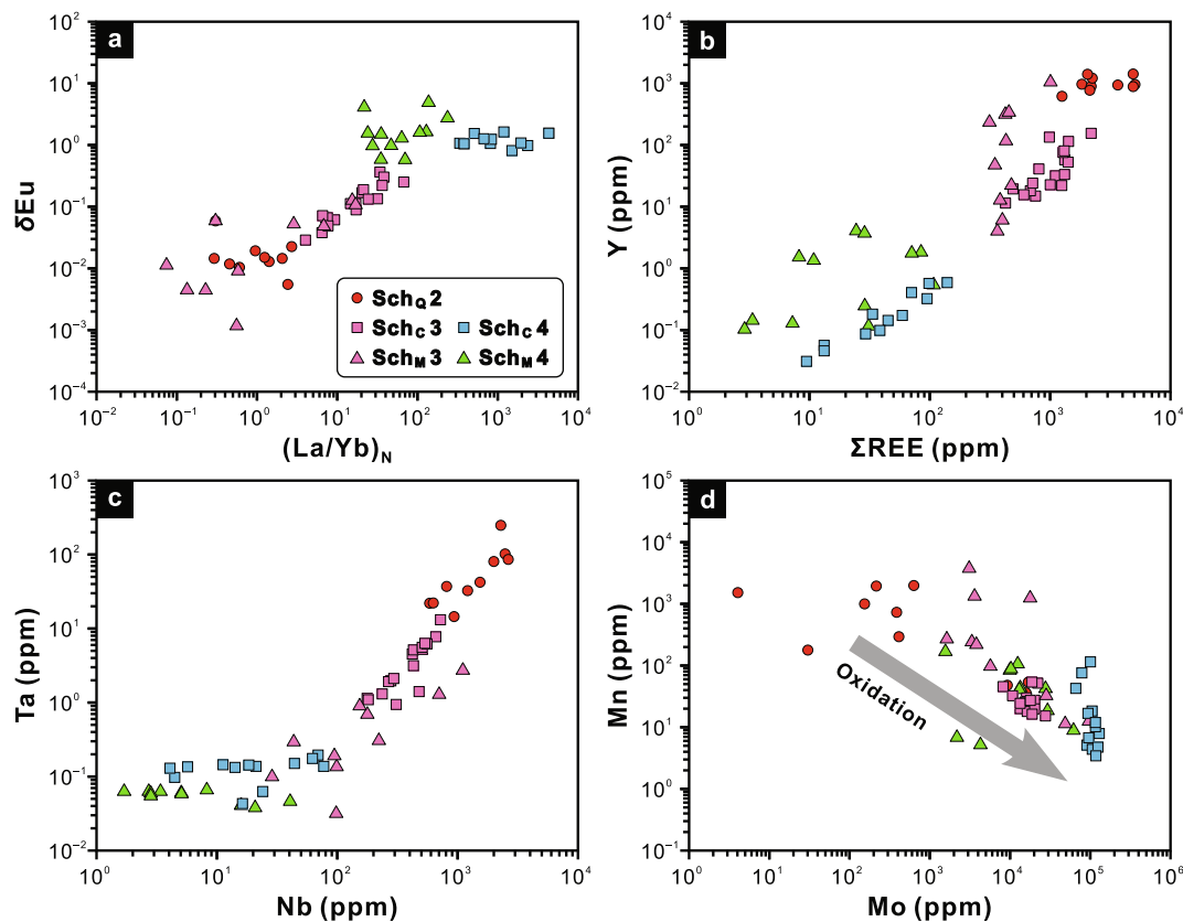
Fig. 12. (a) (La/Yb)_N - \delta Eu , (b) \Sigma REE (ppm)-Y (ppm), (c) Nb (ppm)-Ta (ppm), and (d) Mo (ppm)-Mn (ppm) binary diagrams of the Weijia scheelites.
