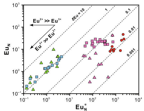
Fig. 16. Eu_N vs. Eu_N^* [( Sm_N \times Gd_N ) 1/2 ] diagram (after Ghaderi et al., 1999) of the Weijia scheelites. Legend refers to Fig. 12.
