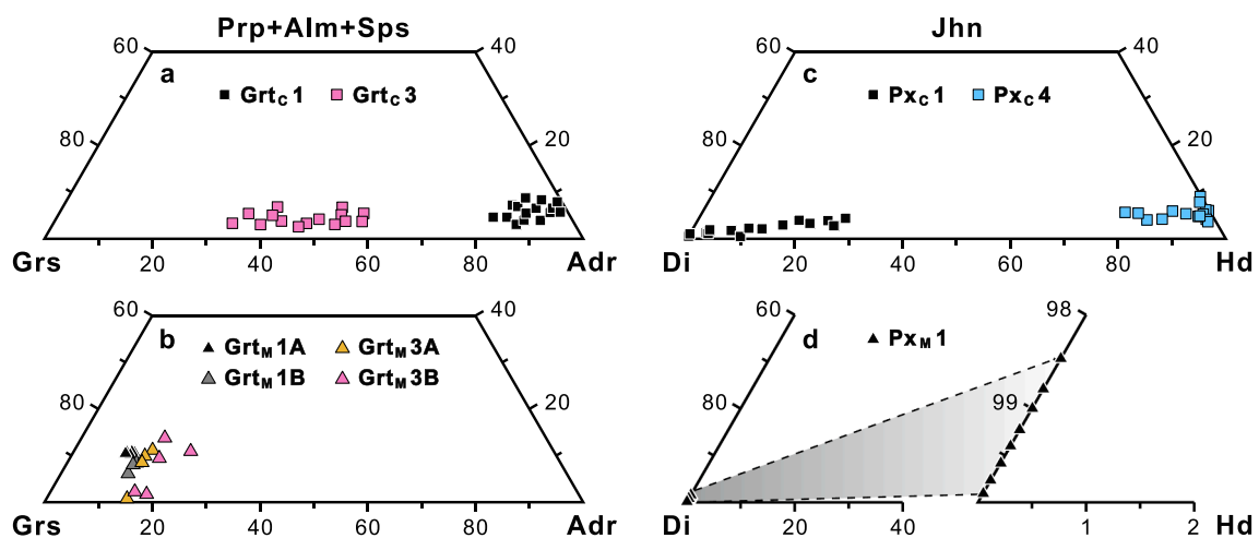
Fig. 8. Major element compositions of different generations of garnets and pyroxenes from the Weijia W skarn deposit. End-member abbreviations: Adr = andradite, Alm = almandine, Di = diopside, Grs = grossular, Hd = hedenbergite, Jhn = johannsenite, Prp = pyrope, Sps = spessartine.
