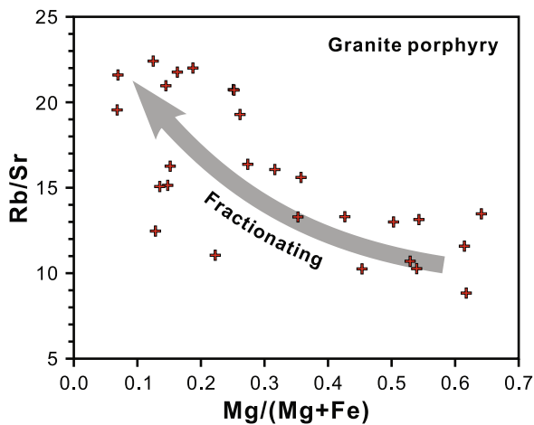
Fig. 15. Rb/Sr vs. Mg/(Mg+Fe) diagram of the Weijia granite porphyry. These whole-rock geochemical data are from Zhao et al. (2016), Huang et al. (2017), and Wu et al. (2021).
