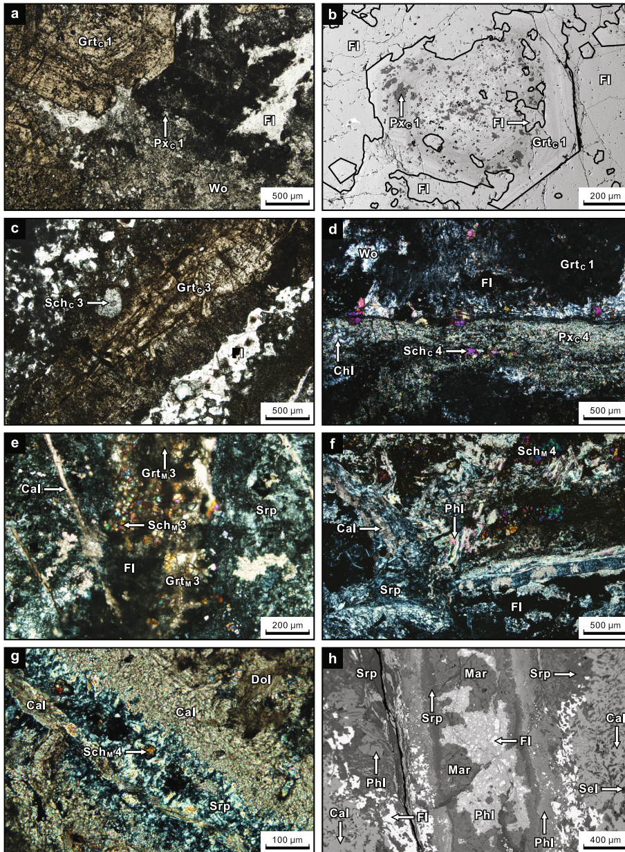
Fig. 5. Petrographic photomicrographs of the calcic and magnesian skarns with different generations of garnets and scheelites from the Weijia W deposit. (a) Stage-1 disseminated garnet and pyroxene in the calcic skarn (PPL). (b) The stage-1 garnet enclosing the stage-1 pyroxene and replaced by fluorite in the calcic skarn (BSE). (c) Stage-3 stockwork garnet and associated scheelite in the calcic skarn (PPL). (d) Stage-4 stockwork pyroxene and associated scheelite in the calcic skarn (XPL). (e) Stage-3 garnet and associated scheelite in the stockwork magnesian skarn (XPL). (f) Stage-4 scheelite coexisting with phlogopite in the stockwork magnesian skarn (XPL). (g) Stage-4 scheelite coexisting with serpentine in the stockwork magnesian skarn (XPL). (h) Stage-1 marialite ( \text{Na}_4\text{Al}_3\text{Si}_9\text{O}_{24}\text{Cl} ) in the stockwork magnesian skarn (BSE). Mineral abbreviations: Cal = calcite, Chl = chlorite, Dol = dolomite, Fl = fluorite, Grt = garnet, Mar = marialite, Phl = phlogopite, Px = pyroxene, Sch = scheelite, Sel = sellaite, Srp = serpentine, Wo = wollastonite.
