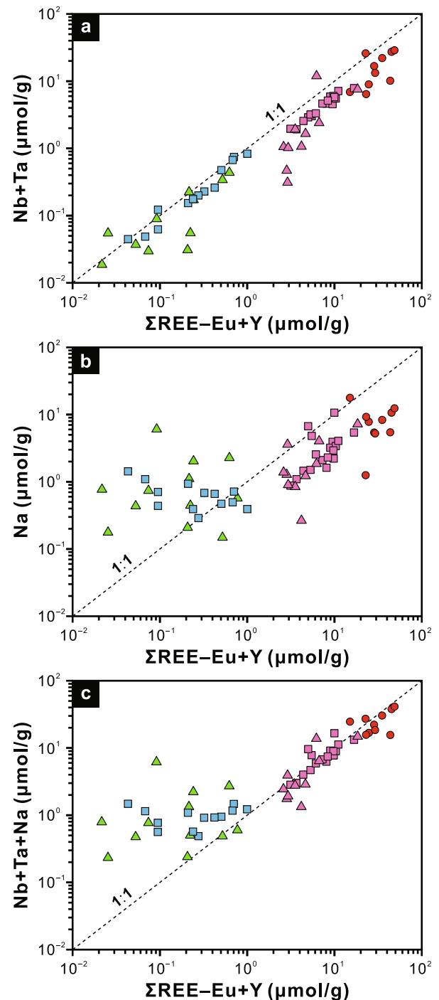
Fig. 14. (a) Nb+Ta ( \mu\text{mol/g} ) vs. \Sigma\text{REE-Eu+Y} ( \mu\text{mol/g} ), (b) Na ( \mu\text{mol/g} ) vs. \Sigma\text{REE-Eu+Y} ( \mu\text{mol/g} ), and (c) Nb+Ta+Na ( \mu\text{mol/g} ) vs. \Sigma\text{REE-Eu+Y} ( \mu\text{mol/g} ) correlational plots of the Weijia scheelites. Legend refers to Fig. 12.
