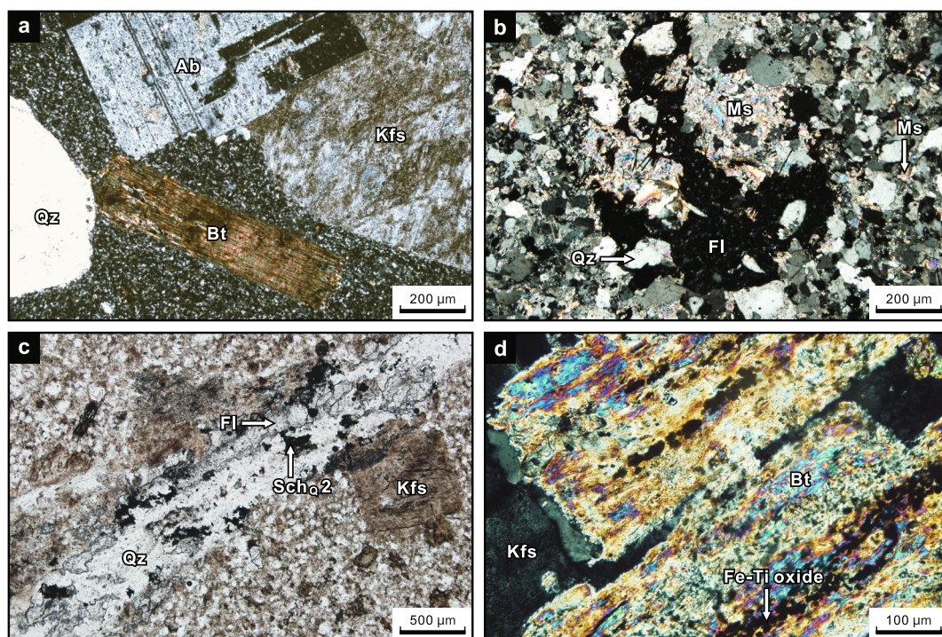
Fig. 4. Petrographic photomicrographs of the granite porphyry and its stockwork quartz veinlets from the Weijia W skarn deposit. (a) Subvolcanic porphyritic texture of the granite porphyry with phenocrysts of quartz, K-feldspar, albite, and biotite (crossed-polarized light, XPL). (b) Interstitial muscovite and muscovite-fluorite aggregates in the matrix of granite porphyry (XPL). (c) Stage-2 scheelite coexisting with fluorite in the stockwork quartz veinlets hosted by weakly greisenized granite porphyry (plane-polarized light, PPL). (d) Altered biotite in the granite porphyry (XPL). Mineral abbreviations: Ab = albite, Bt = biotite, Fl = fluorite, Kfs = K-feldspar, Ms = muscovite, Qz = quartz, Sch = scheelite. Subscript Q represents stockwork quartz veinlets, Arabic numeral denotes paragenetic stage.
