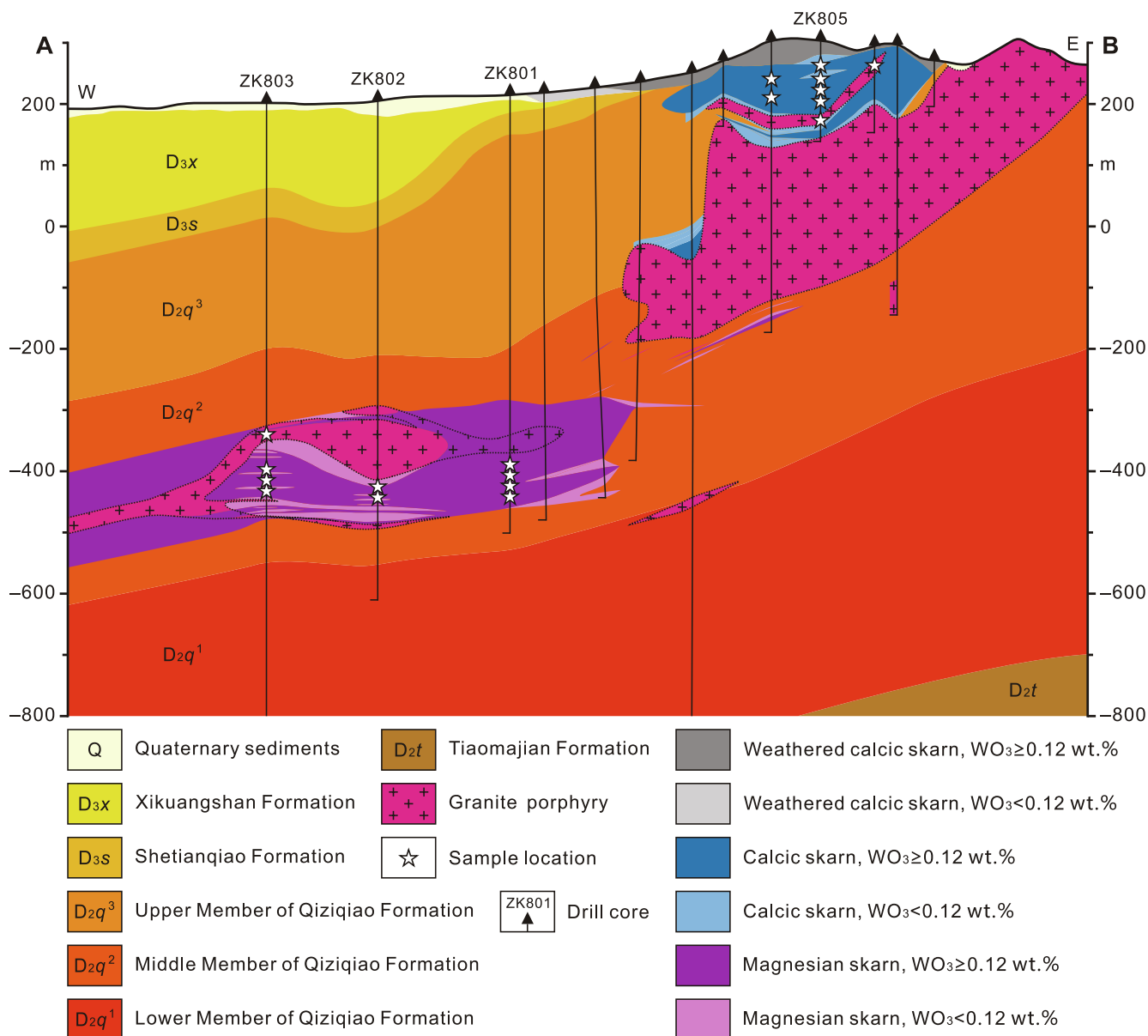
Fig. 2. West-east-trending geological cross section (section line shown in Fig. 1b) of the Weijia W skarn deposit.
