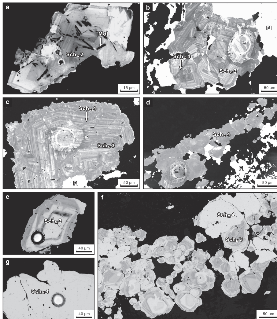
Fig. 7. (a–d) CL and (e–g) BSE images showing the textures of scheelites in the stockwork quartz veinlets (a), calcic skarn (b–d), and magnesian skarn (e–g). Mineral abbreviations: Fl = fluorite, Mol = molybdenite, Sch = scheelite. Subscripts Q, C, and M represent stockwork quartz veinlets, calcic skarn, and magnesian skarn, respectively, Arabic numerals denote paragenetic stages.
