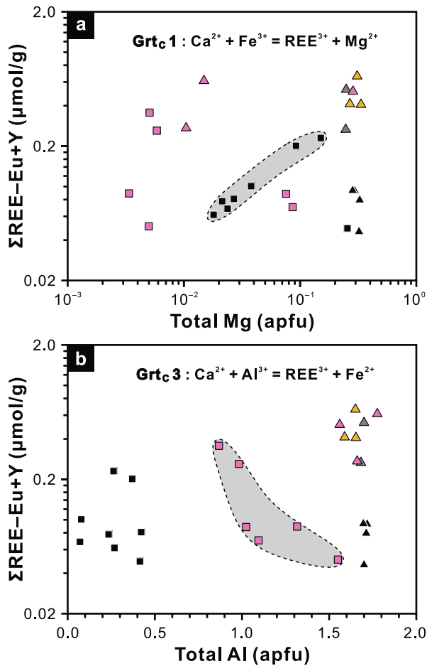
Fig. 13. (a) \Sigma\text{REE-Eu+Y} ( \mu\text{mol/g} ) vs. Total Mg (apfu: atoms per formula unit) and (b) \Sigma\text{REE-Eu+Y} ( \mu\text{mol/g} ) vs. Total Al (apfu) correlational plots of the Weijia garnets. Legend refers to Fig. 10.
