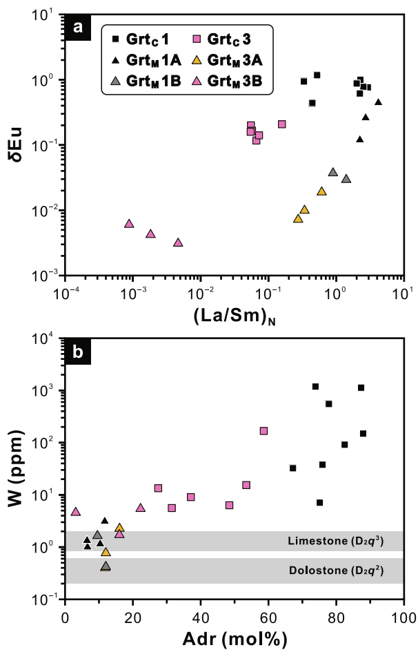
Fig. 10. (a) (La/Sm)_N - \delta Eu [ Eu_N/(Sm_N \times Gd_N)^{1/2} ] and (b) Adr (mol%)-W (ppm) binary diagrams of the Weijia garnets. The W data of carbonate strata are listed in Supplementary Table S5.
