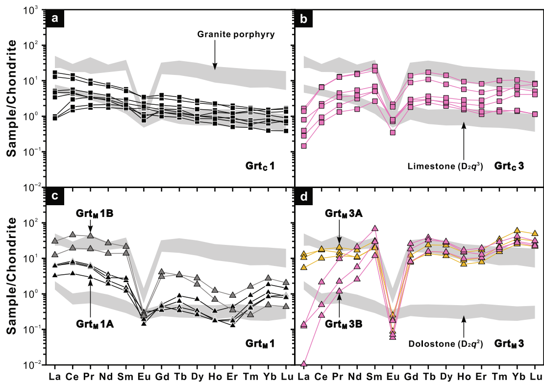
Fig. 9. Chondrite-normalized (Boynton, 1984) REE patterns of different generations of garnets from the Weijia W skarn deposit. The REE data of granite porphyry and carbonate strata are from Huang et al. (2017) and listed in Supplementary Table S5, respectively.
