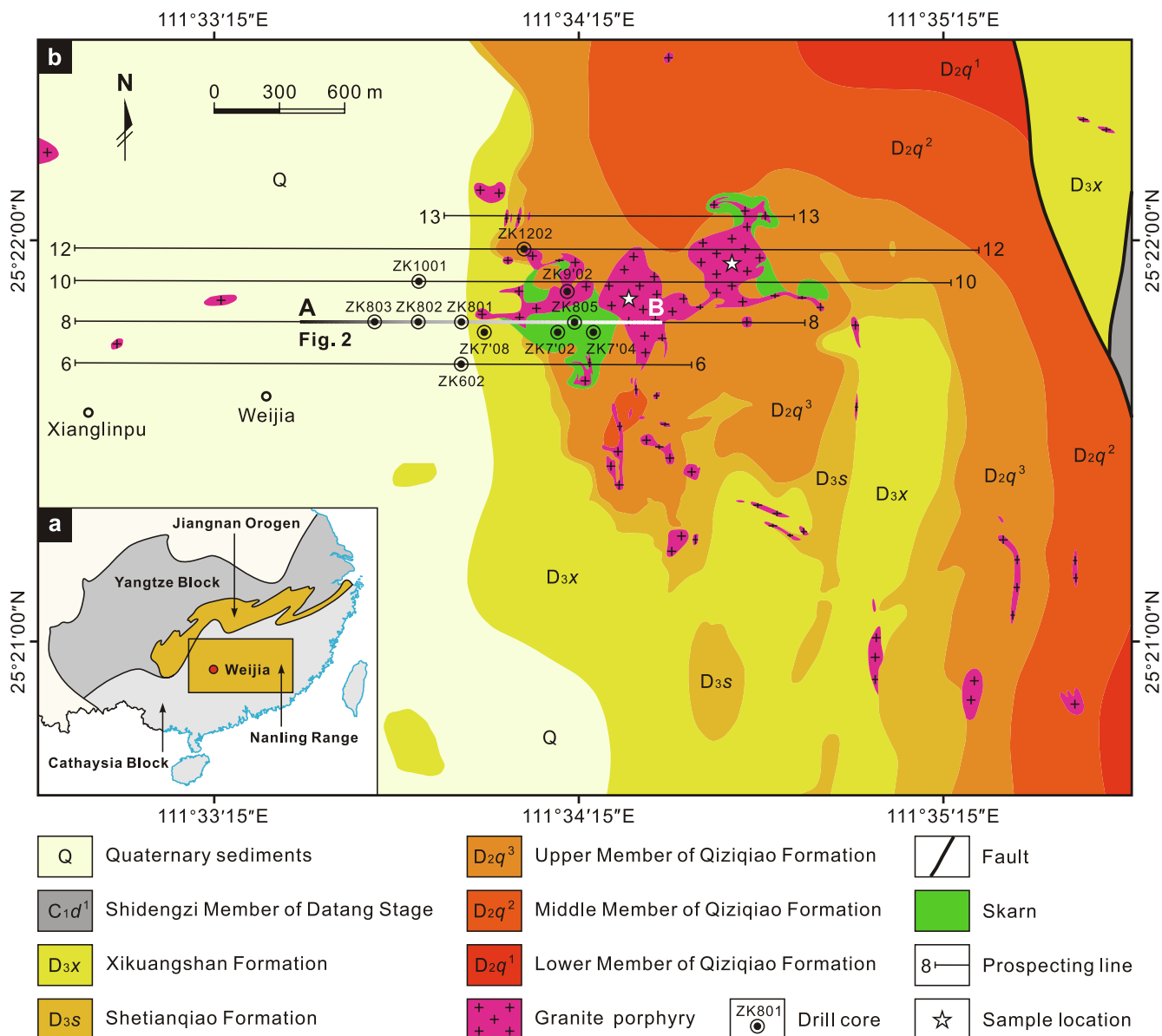
Fig. 1. (a) Map of South China showing the location of the Weijia W skarn deposit. (b) Geological map of the Weijia W skarn deposit.
