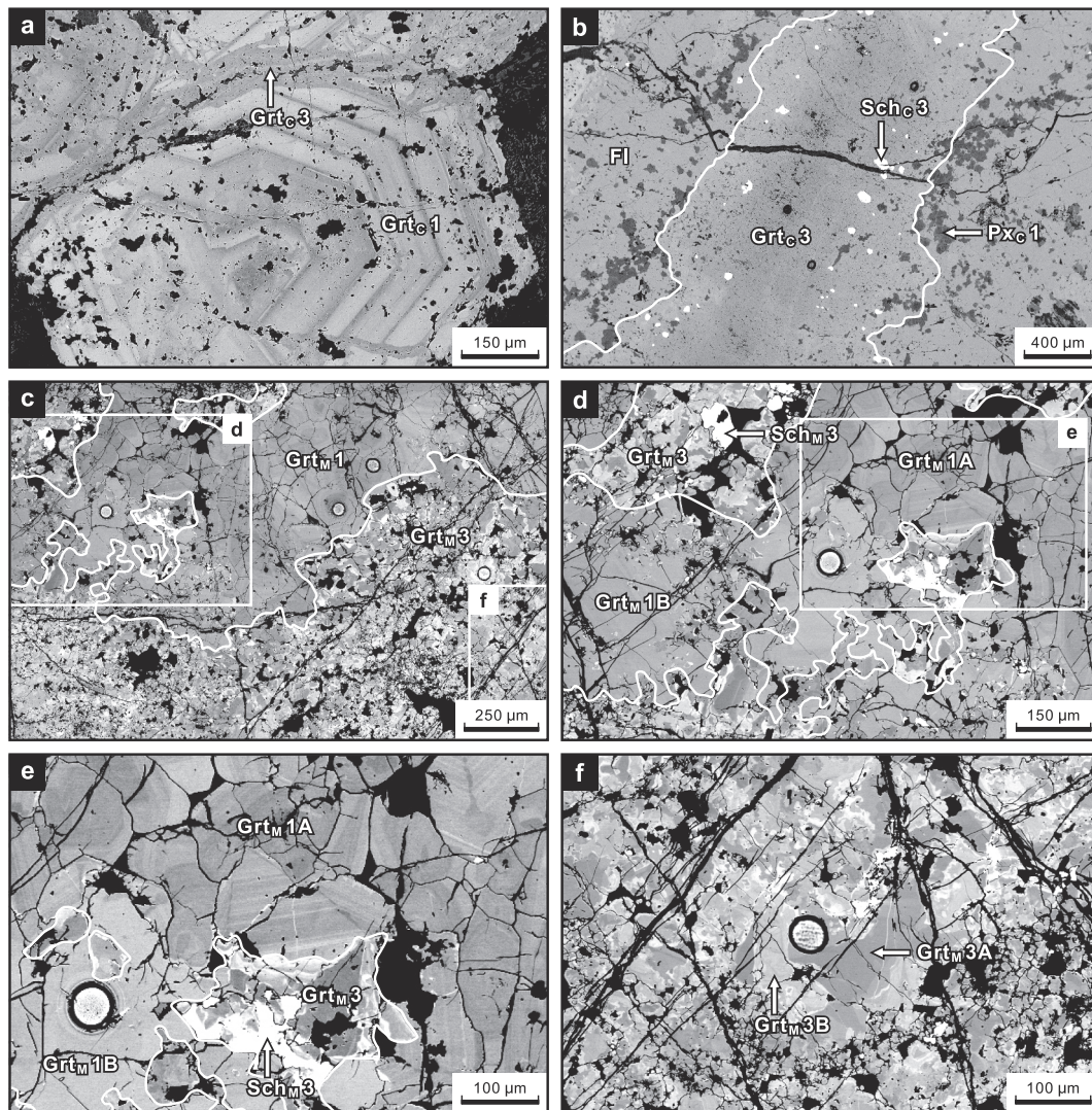
Fig. 6. BSE images showing the textures of garnets in the calcic skarn (a–b) and magnesian skarn (c–f). Mineral abbreviations: Fl = fluorite, Grt = garnet, Px = pyroxene, Sch = scheelite. A and B denote two subgenerations of the Grt M 1 and Grt M 3.
