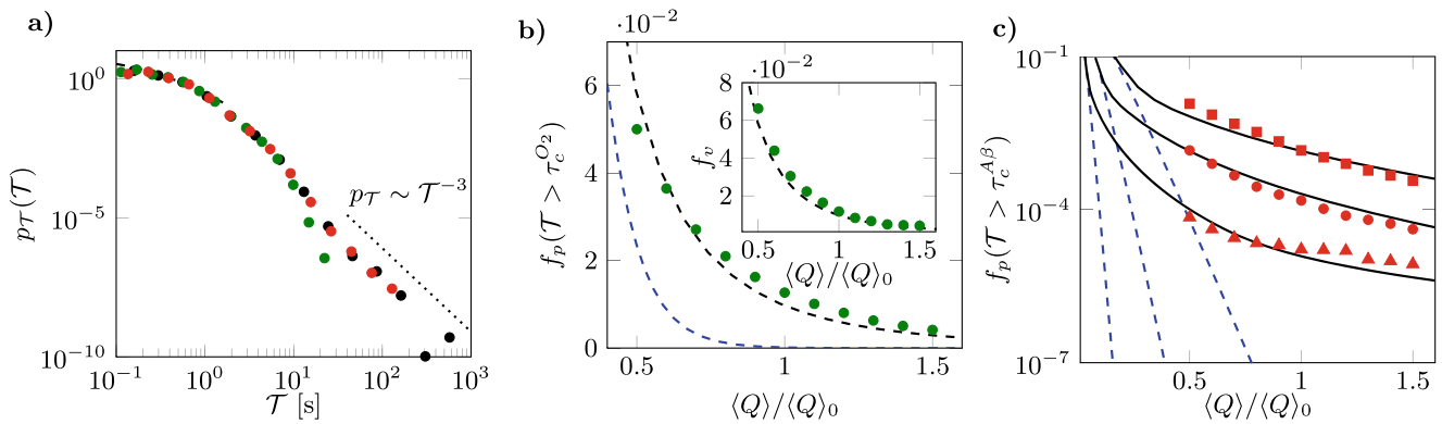
Fig. 4 Long travel times, captured by our mechanistic model, drive the emergence of critical areas with impaired oxygen delivery and amyloid-β clearance under hypoperfusion. a CTRW model predictions (full black line) compared to purely advective, amyloid-β, and oxygen transport simulations (black, red, and green dots, respectively). The prediction of the mean-field transport model (Eq. (6)) and of the reference CTH model (Supplementary Note 7) are shown as dashed black and blue lines, respectively. b Fraction f_p of network travel times larger than \tau_c^{O_2} for oxygen delivery as a function of average flow rate \langle Q \rangle / \langle Q \rangle_0 . Simulations (green dots) are compared to the predictions of the mean-field model (dashed black line) and of the reference CTH model (dashed blue line). The inset shows the fraction f_v of vessels in the network that are only reached by flow paths with travel times to these vessels larger than \tau_c^{O_2} , as a function of the flow rate. c Fraction f_p of network travel times larger than \tau_c^{AB} = 8 s (squares), \tau_c^{AB} = 16 s (dots) and \tau_c^{AB} = 40 s (triangles), as a function of average flow rate for amyloid-β clearance. The predictions of the CTRW model (Eq. (7)) for each value of \tau_c^{AB} are shown as continuous black lines. The predictions of the reference CTH model (see Supplementary Note 7) for each value of \tau_c^{AB} are shown as blue dashed lines.
