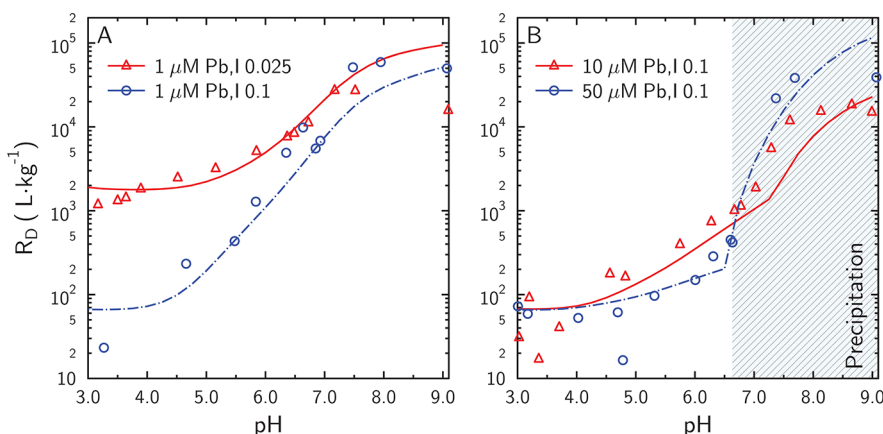
Figure 10. Model predictions (lines) of \text{Pb}^{2+} adsorption data (symbols) on Kunipia-P from Orucoglu et al. 67 (A) \text{Pb}^{2+} ( 1 \mu\text{mol} \cdot \text{L}^{-1} ) in the presence of 0.025 \text{ mol} \cdot \text{L}^{-1} \text{NaCl} (red triangles and red full line) and 0.1 \text{ mol} \cdot \text{L}^{-1} \text{NaCl} (blue circles and blue dashed line). (B) \text{Pb}^{2+} ( 10 \mu\text{mol} \cdot \text{L}^{-1} (red triangles and red full line) and 50 \mu\text{mol} \cdot \text{L}^{-1} (blue circles and blue dashed line)) in the presence of 0.01 \text{ mol} \cdot \text{L}^{-1} \text{NaCl} . Dashed area (////) highlights the pH region in which hydrocerussite ( \text{Pb}_3(\text{CO}_3)_2(\text{OH})_2 ) precipitation was expected at 50 \mu\text{M Pb}^{2+} total concentration..
