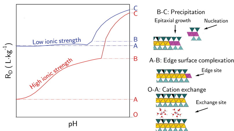
Figure 1. Sorption processes as a function of pH and ionic strength. Dominant mechanisms are cation exchange between O and A region, edge surface complexation between A and B region and precipitation between B and C region.
