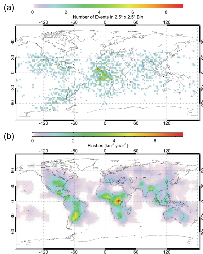
Figure 6. (a) Map of event locations. The location of a given event is determined as the location of the DEMETER spacecraft at the time of the minimum of the event frequency dependence. The number of events in each 2.5^\circ \times 2.5^\circ bins is color coded according to the scale on the top. (b) The average lightning activity from LIS/OTD in the local time window 20.7–23.7 h is color coded according to the scale at the top. This local time range corresponds to DEMETER nighttime half orbits.
