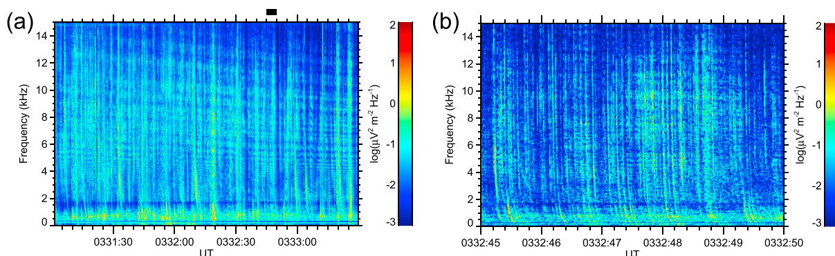
Figure 3. (a) Detailed frequency-time spectrogram of power spectral density of electric field fluctuations corresponding to the first Burst mode interval from Figure 1. (b) Detailed frequency-time spectrogram corresponding to a 5 s long time interval marked by the black bar on the top of Figure 3a.
