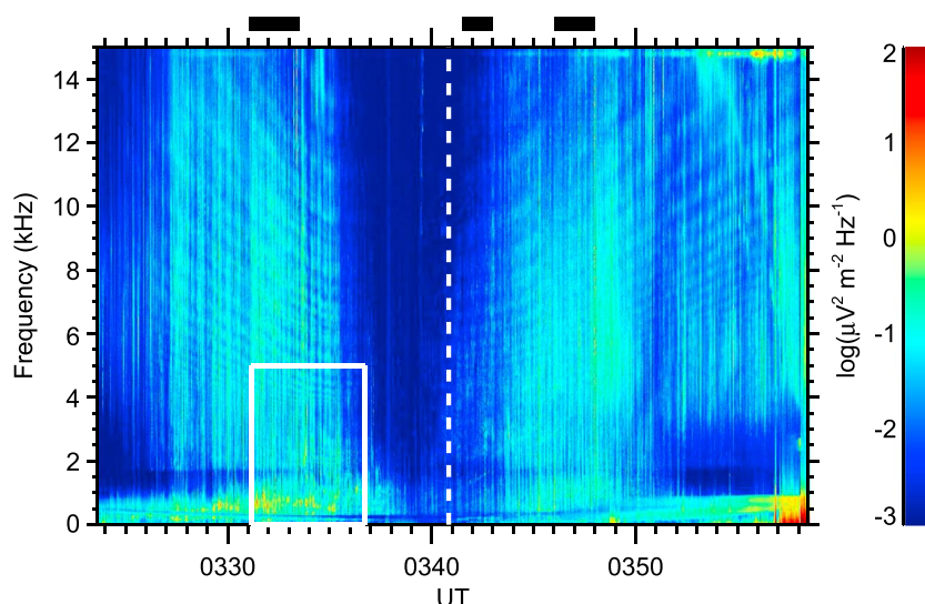
Figure 1. Frequency-time spectrogram of power spectral density of electric field fluctuations corresponding to one of the observed events. The frequencies of reduced intensity first decrease with time, then there is an apparent gap in the event, and, finally, the frequencies of reduced intensity increase with time. The data were measured on 7 February 2007. The white vertical dashed line at about 03:41 UT corresponds to the time when DEMETER crossed the geomagnetic equator. Black bars on the top mark the time intervals when the Burst mode was active and high-resolution data were available.
