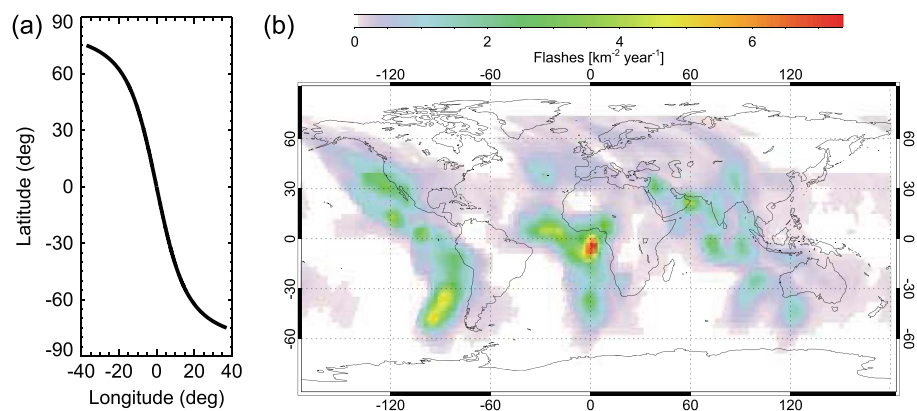
Figure 7. (a) Trajectory corresponding to a DEMETER nightside half orbit. (b) Map of lightning locations from LIS/OTD shifted by 3000 km in the west/southwest direction. The direction of the shift was determined in each location to be perpendicular to the DEMETER orbit at the resulting shifted location; i.e., the shifted location is the place where the DEMETER spacecraft gets closest to the original location.
