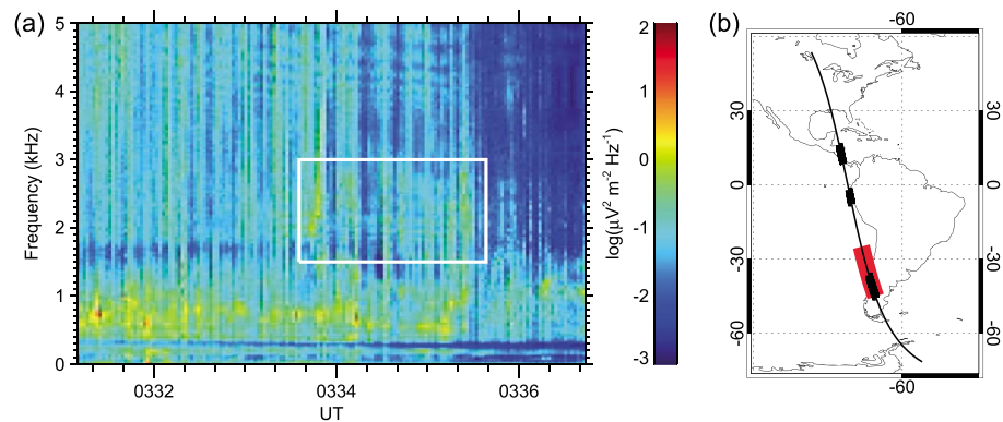
Figure 2. (a) Zoomed frequency-time spectrogram of power spectral density of electric field fluctuations corresponding to the interval marked by the white rectangle in Figure 1. The white rectangle marks an additional faint reduced intensity event at lower frequencies. (b) Map showing the DEMETER locations during the time interval analyzed in Figure 1 (thin curve). The part of the DEMETER orbit corresponding to the zoomed interval from Figure 2a is shown by the solid red rectangle. Parts of the DEMETER orbit with the active Burst mode are shown by the thick black curves. Note that DEMETER moved from the south to the north.
