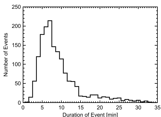
Figure 4. Histogram of the observed event durations.
