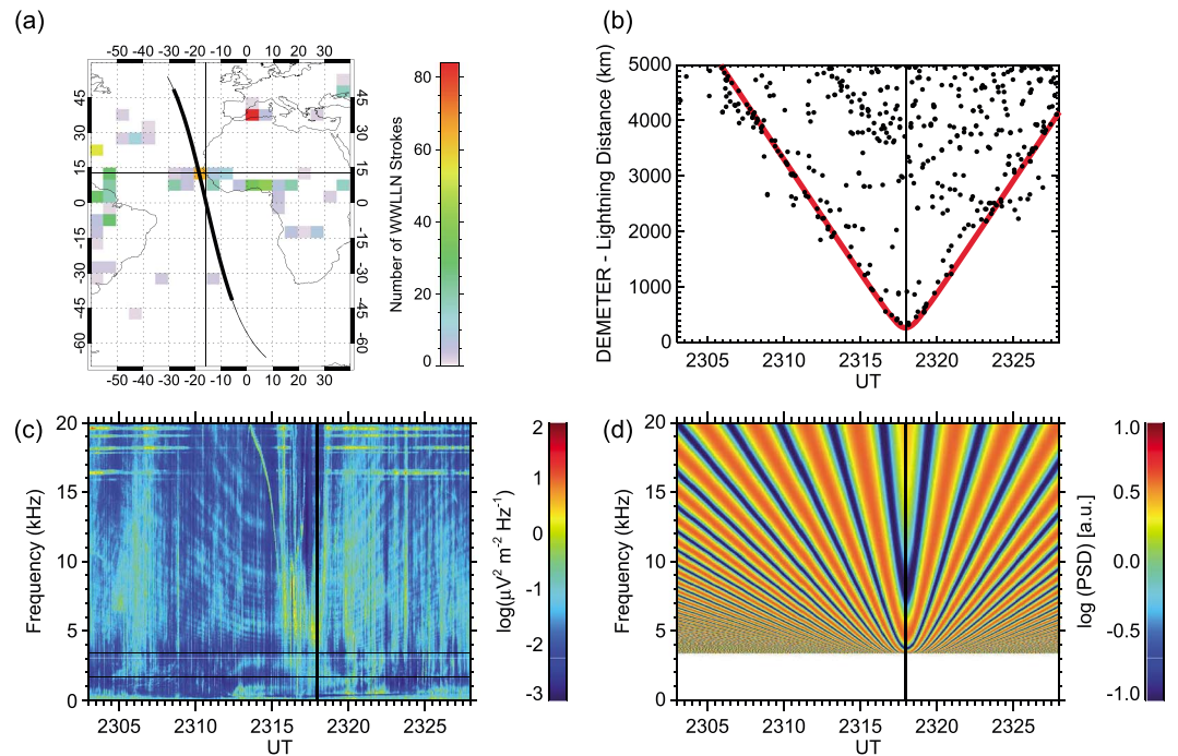
Figure 9. The same as Figure 8 but for the event measured on 22 September 2007. Note that the situation is less clear than in Figure 8, with several different storms occurring in the vicinity of the DEMETER spacecraft at the time of the event. Also note that the DEMETER spacecraft passed very close to the source storm in this particular event.
