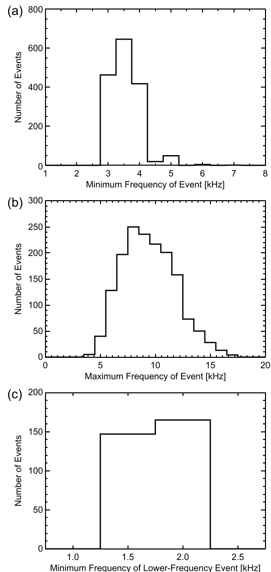
Figure 5. (a) Histogram of minimum frequencies of events. (b) Histogram of maximum frequencies of events. (c) Histogram of minimum frequencies of lower frequency events. The frequency resolution of all these histograms is 0.5 kHz.
