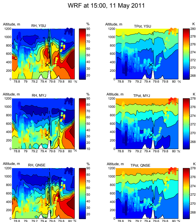
Figure 10. Cross-section of the WRF model relative humidity (RH) and potential temperature (TPot) at 15:00 UTC (JD 131.6) shown as a function of altitude along the transect line. CMET observations for the whole flight are also illustrated, with approximate balloon location at 15:00 denoted by a cross.
