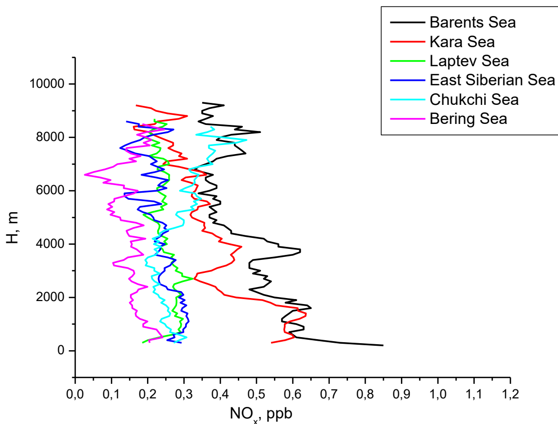
Figure 16: Vertical distribution of nitrogen oxides over sea areas.
