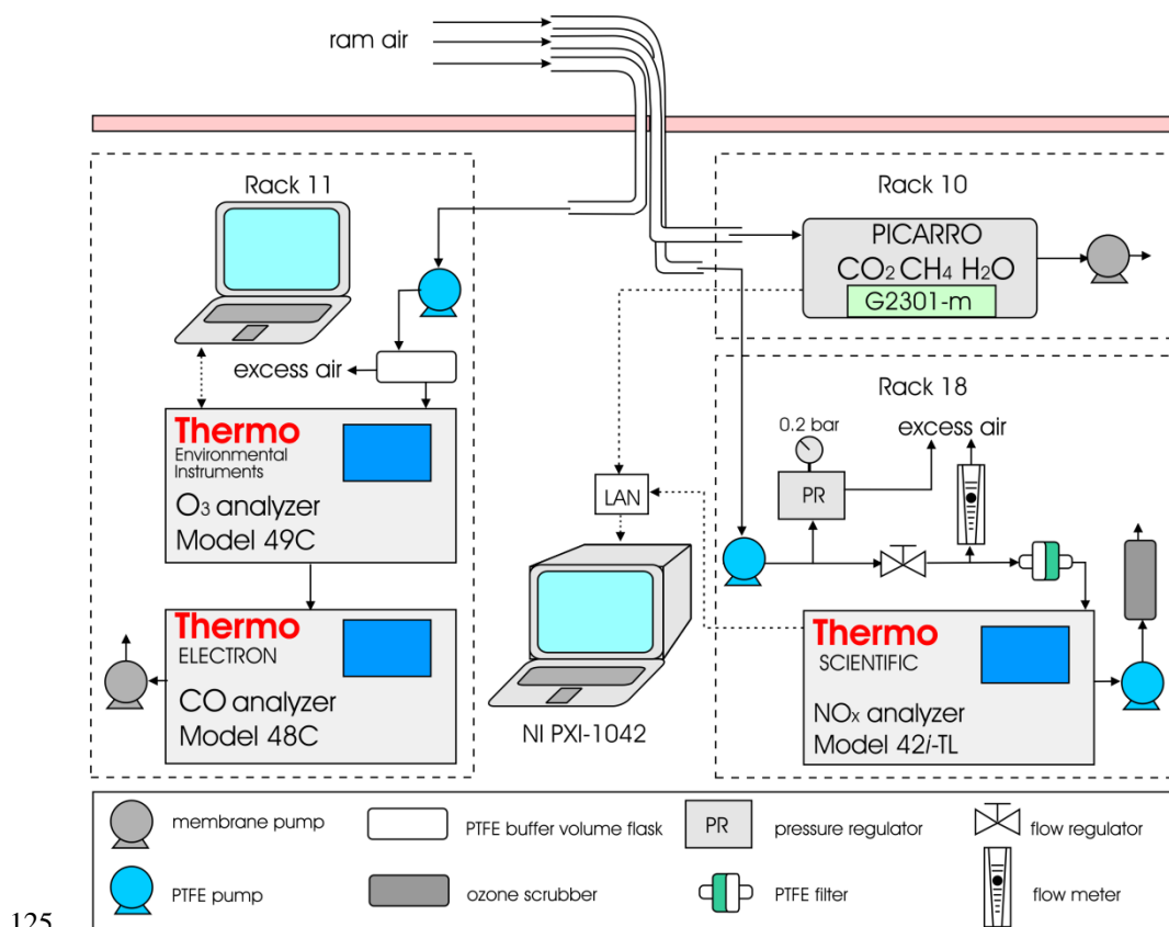
Figure 2: Schematic diagram of the gas analysis instrument suite: solid lines – air ducts; dash lines – communication cables.
