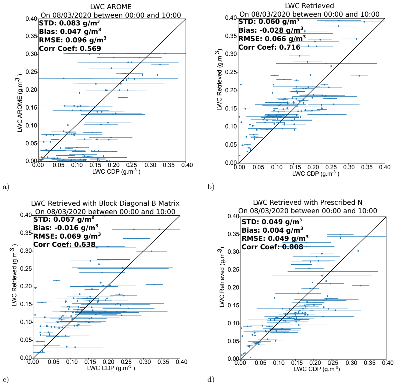
Figure 10. Scatter plots of the liquid water content a) background and b) ,c) ,d) retrieved versus the liquid water content observed through with in-situ sensor. Panels b, c and d refer respectively to 1D-Var retrievals run with the nearest background profiles and full fog B matrix with cross-correlations between variables, 1D-Var retrievals run with the nearest background profile and a bloc-diagonal B matrix, 1D-Var retrievals run with the nearest background profiles and full fog B matrix with cross-correlations with the use of the CDP droplet number concentration inside the radar simulator during the minimization. Error bars indicate the range of in-situ observations recorded throughout the height level corresponding to the retrieval height levels.
