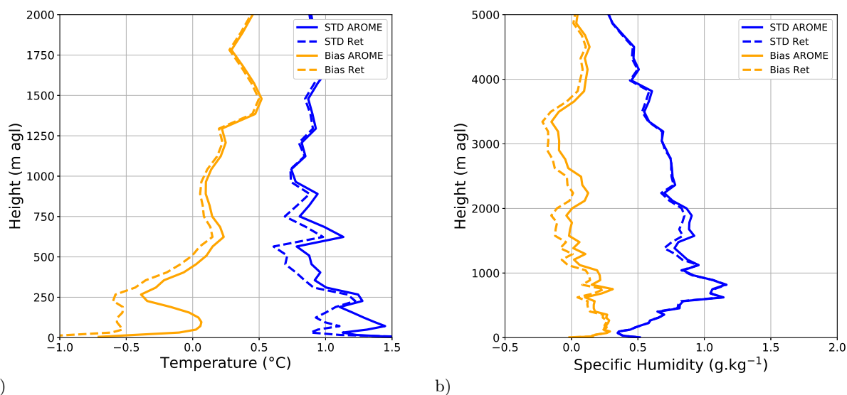
Figure 12. RMSE and bias of a) temperature retrievals and b) specific humidity retrievals made throughout the SOFOG-3D field campaign. Dotted lines correspond to the background profile and dotted lines to retrieved profile statistics, where blue lines denote the standard deviation of errors and yellow lines to the bias.
