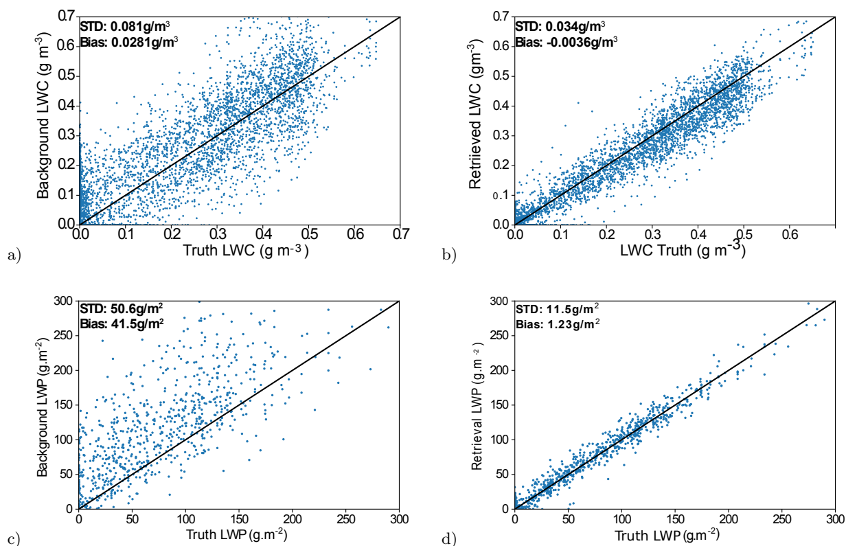
Figure 2. Scatter plots showing the values of LWC of the a) background and truth and b) the retrieval and truth; and the LWP for c) background and truth and d) retrieval and truth. Where points lie on the black line, a perfect prediction of the LWC/LWP is made, and the further from the black line, the worse the prediction is. The standard deviation and bias of the background/retrieval - true values is also indicated.
