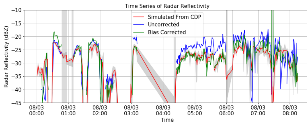
Figure 5. The radar reflectivity simulated from the CDP droplet measurements, observed with the BASTA cloud radar, and the observation after a bias correction had been performed.
