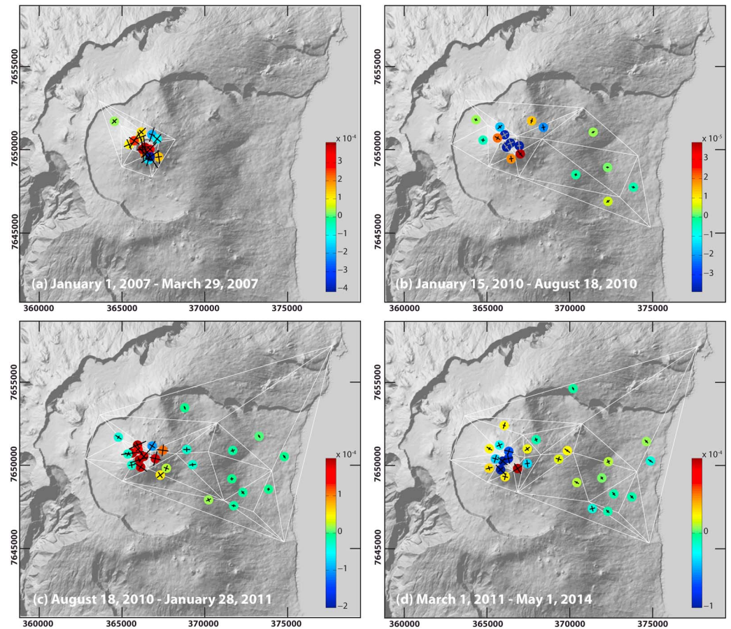
Figure 4. Major principal strain \varepsilon_1 spatial distribution (in color) during representative periods of (a, c) activity and (b, d) rest. Figure 4a period includes one eruption (18 February 2007), and Figure 4c period includes two eruptions (14–31 October and 9–10 December 2010) and two intrusions (19 and 23 September 2010). Black crosses represent the orientation of the principal strains. The center of each solid colored circle is the weighted geometric center of the corresponding triangle, the weight being the module of the horizontal displacement recorded at each station. Coordinates in UTM WGS84.
