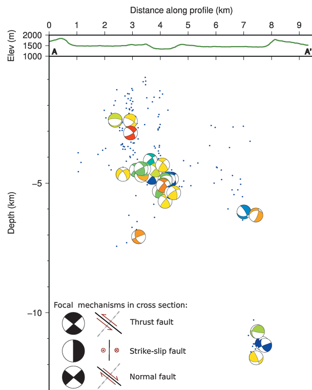
Figure 9. (top) Topography of Nabro along transect A-A'. (bottom) All focal mechanisms have been projected on to transect A-A' (Figure 6), then rotated to a side view, as viewed from south to north.
