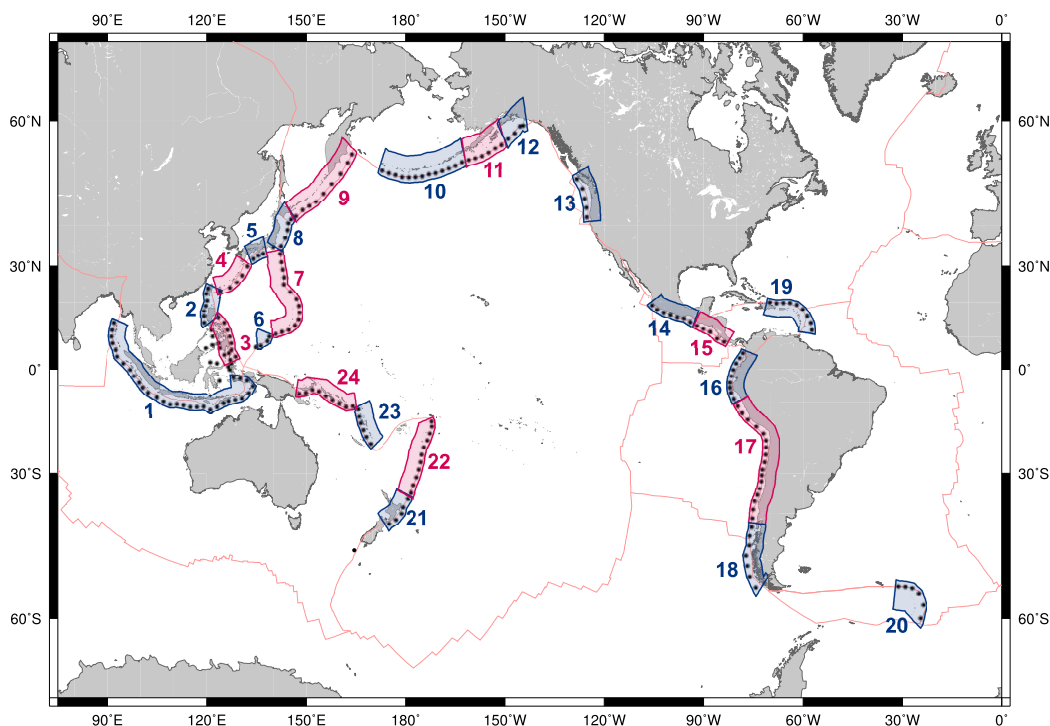
Figure 12. Map of the Pacific, Sandwich, and Antilles subduction zones. Black dots show the locations of the profiles defined in Lallemand et al. [2005] which are used in Figures 10 and 11. The 24 colored boxes show the grouping of these profiles used in the analysis of seismicity (Figure 13 and supporting information Table S1). Light red lines represent plate boundaries.
