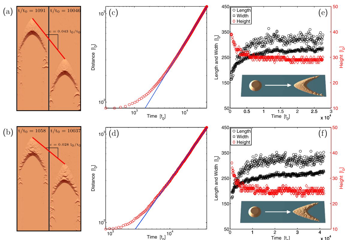
Figure 2. Barchans in quasi-stationary equilibrium states for high and low flows: (a) \tau_1/\tau_0 = 1 and (b) \tau_1/\tau_0 = 20 . The initial condition at t = 0 is a truncated conical sand pile. All the sedimentary cells ejected downstream are randomly reinjected upstream. (c and d) Position of the center of mass and (e and f) evolution of the length, width, and height of the sand pile with respect to time. Over a short time, some sediment is redistributed within the entire system and the dune accelerates as it decreases in height. Over a long time, the steady state barchans are characterized by constant propagation speed and size. Note that superimposed bed forms are responsible for the systematic fluctuations of the dune dimensions.
