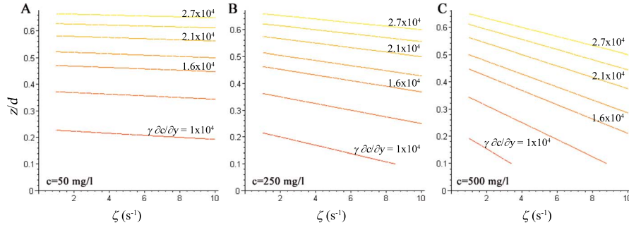
Figure 6. Contour plot of \gamma \partial c / \partial y from equation (7) as a function of the vertical vorticity component, \zeta , and the normalized depth z/d , for different suspended sediment concentration (SSC): (a) c = 50 mg/L, (b) 250 mg/L, and (c) 500 mg/L. Note how the proportionality between \zeta and \gamma \partial c / \partial y is strongly affected by the local SSC: At a given depth, for large (small) sediment in suspension, variations of \zeta correspond to large (small) variations of \gamma \partial c / \partial y . The proportionality depends only weakly on depth.
