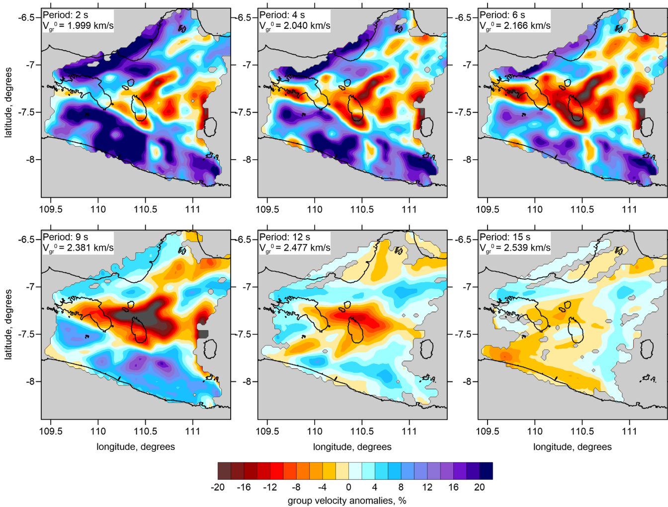
Figure 7. Examples of the two-dimensional maps of group velocities deviations for different periods indicated in the top-left corners of each plots. An average group velocity for each period used as reference values are indicated.
