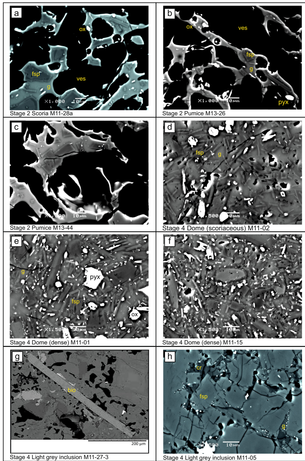
Fig. 2 a–h Representative BSE images of 2010 lithologies showing feldspar microlites ( fsp ), pyroxene microlites ( pyx ), Fe-Ti oxide microlites ( ox ), groundmass glass ( g ) and vesicles ( ves ). Note the presence of biotite ( bio ) and cristobalite ( cr ) and the speckled
