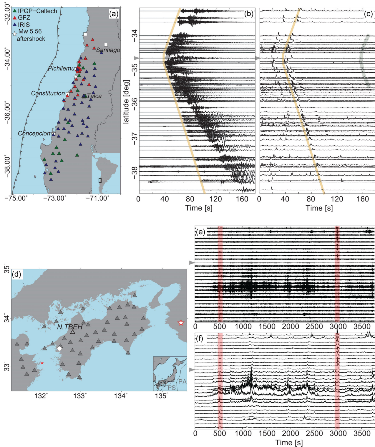
Figure 7. (a–c) Example of MBF signal characterization applied to IMAD post-seismic network in Chile: (a) Map view of central Chile; coloured triangles indicate the IMAD seismic stations. The colour of triangle corresponds to the institution to which the station belongs. White star shows the epicentre of the M 5.2 earthquake after Rietbrock et al. (2012). (b) Record section of UD component seismograms corresponding to the 3 min record of M 5.2 earthquake at the stations. Dark yellow line indicates the P -wave moveout. Grey triangle marks the record presented in Figs 2(a)–6(a), shown in grey. (c) Record section of broad-band kurtosis HOS CFs from MBF analysis in the frequency range 0.02–50.00 Hz. Dark yellow and grey lines indicate, respectively, the move-out of P -wave corresponding to M 5.2 event, and later small event in its coda. (d)–f) Example of MBF signal characterization scheme applied to Hi-net stations in southwestern Japan: (d) Map view of southwestern Japan; grey triangles indicate the Hi-net seismic stations. White stars show the epicentres of earthquakes during 2100–2200 JST, 2012 May 27, from JMA catalogue. White circle correspond to the position of the tectonic tremor activity during same period reported by NIED. (e) Record section of 1 hr EW component seismograms of the tremor activity recorded during 2100–2200 JST, 2012 May 27 at Hi-net stations. Red shadow lines mark the times corresponding to the two earthquakes from JMA catalogue. (f) Broad-band RMS envelope CFs, estimated by applying the MBF analysis in the frequency range 2.0–40.0 Hz to the records in panel (e).
