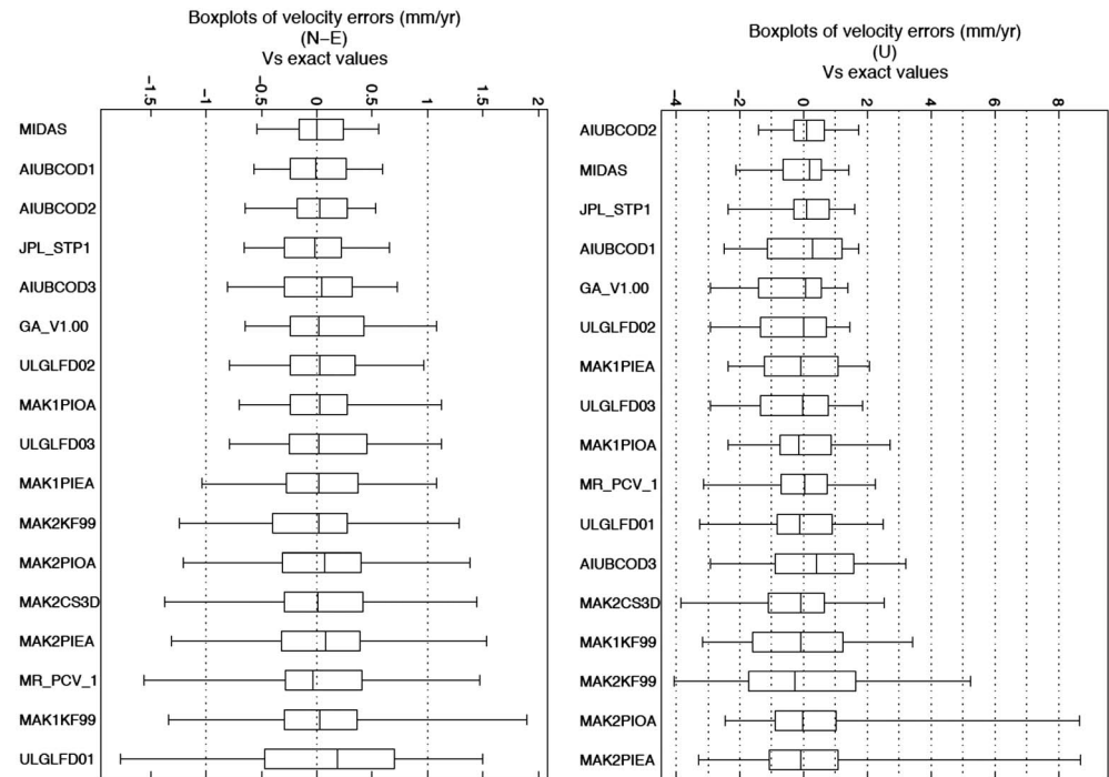
Figure 4. Boxplots summarizing the velocity error distributions using the DOGE synthetic data for (left) north and east components and (right) up component. Results are from MIDAS and from least squares using steps identified by 16 of the best automatic step detection programs. The box width is the IQR, and the central line is the median. The width between whiskers is the IPR. Boxplots are ranked top to bottom in order of increasing IPR. MIDAS outperforms least squares with step detection.
