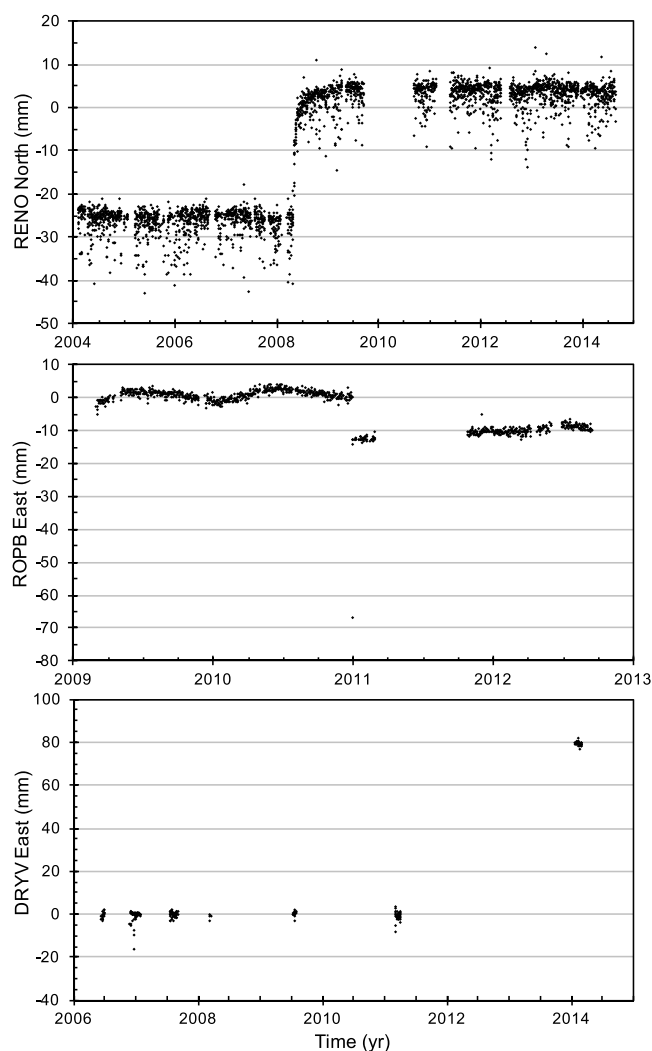
Figure 2. Coordinate time series that have been detrended using the MIDAS velocities for pathological examples detailed in the text: (top) station RENO north component, with an earthquake and skewness; (middle) station ROPB east component, with previously undetected step and outliers; (bottom) station DRYV east component, with displaced monument in the final campaign. Trends agree visually with zero slope lines.
