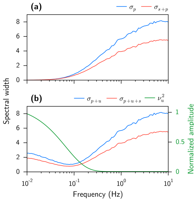
Figure 14. (a) Covariance matrix spectral width as function of frequency estimated for a combination of two first terms from eq. (3): with an propagating noise only ( \sigma_p ) and adding one coherent signal ( \sigma_{s+p} ). (b) Similar to (a) but after adding the third term: the non-propagating noise (whose spectral intensity \nu_u^2(f) is schematically illustrated with the green line).
