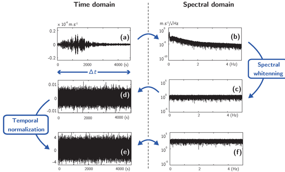
Figure 6. Illustration of the pre-processing of seismic records. (a) Raw data. (b) Raw data amplitude Fourier spectra. (c) Whitened spectral amplitude. (d) Real part of the inverse Fourier transform of the of whitened spectrum. (e) Temporally normalized time-series. (f) Fourier amplitude spectra of (e).
