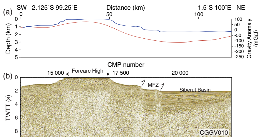
Figure 8. Profile CGGV10: (a) Gravity anomaly (red) and bathymetry (blue) and (b) seismic reflection image. MFZ: Mentawai Fault Zone. Location of profile off of central Sumatra, see Figure 1.
