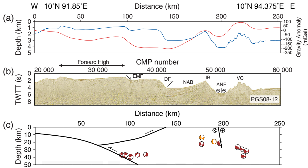
Figure 6. Profile PGS08-12: (a) Gravity anomaly (red) and bathymetry (blue), (b) seismic reflection image, and (c) hypocenters of earthquakes projected along profile in a 50 km wide zone along with their rotated fault plane solutions. The black lines indicate the approximate positions of the plate interface and back thrust. EMF: Eastern Margin Fault, DF: Diligent Fault, IB: Invisible Bank, NAB: Nicobar Andaman Forearc Basin, ANF: Andaman-Nicobar Fault (previously interpreted as WAF), VC: Volcanic Complex.
