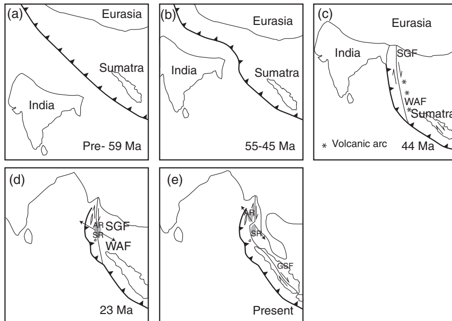
Figure 3. Map diagram illustrating the tectonic history of the Sumatra subduction and the Andaman Sea.
