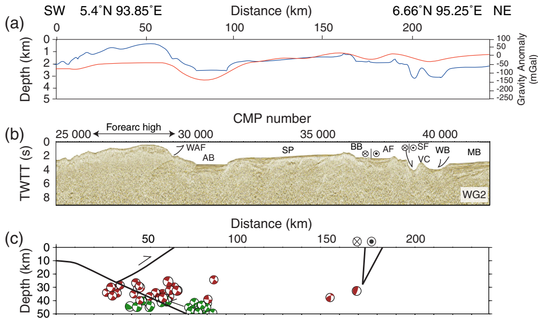
Figure 4. Profile WG2: (a) Gravity anomaly (red) and bathymetry (blue), (b) seismic reflection image, and (c) hypocenters of earthquakes projected along profile WG2 in a 50 km wide zone along with their rotated fault plane solutions. The black lines indicate the approximate positions of the plate interface and back thrust. West Andaman Fault (WAF) is a back thrust. AB: Aceh Basin, SP: Sumatra Platform, AF: Aceh Fault, SF: Seulimeum Fault, VC: Volcanic Centre, BB: Breueh Basin, WB: Weh Basin, MB: Mergui Basin.
