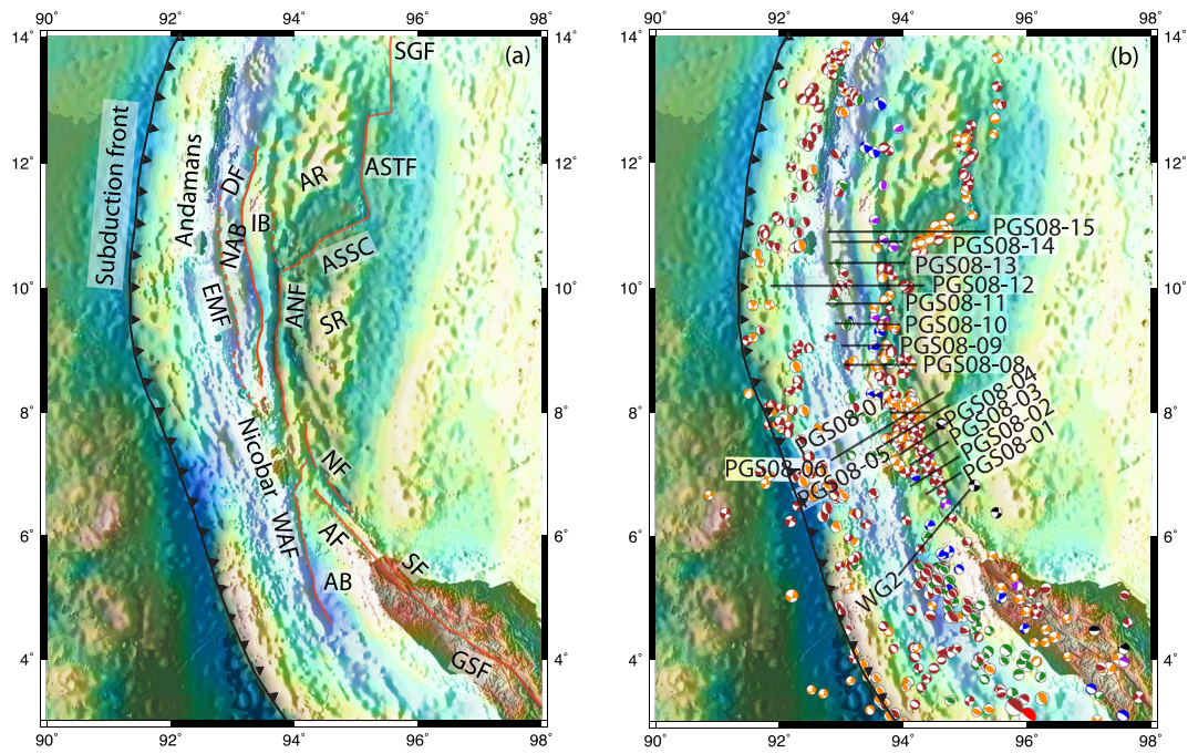
Figure 2. Combined bathymetry and gravity image of the Andaman Sea region showing (a) different tectonic features. AB: Aceh fore-arc basin, WAF: West Andaman Fault, AF: Aceh Fault, GSF: Great Sumatra Fault, SF: Seulimeum Fault, NF: Nicobar Fault, ANF: Andaman-Nicobar Fault, ASSC: Andaman Sea Spreading Centre, ASTF: Andaman Sea Transform Fault, SGF: Sagaing Fault, AR: Alcock Rise, SR: Sewell Rise, EMF: Eastern Margin Fault, DF: Diligent Fault, IB: Invisible Bank, NAB: Nicobar Andaman Forearc Basin. (b) Recent earthquakes with their fault plate solutions for different depths: Orange: 0–20 km; Red: 21–40 km; Green: 41–60 km; Blue: 61–80 km; Purple: 81–100 km; Black: 101–120 km. The black lines indicate the positions of seismic profiles used in this study.
