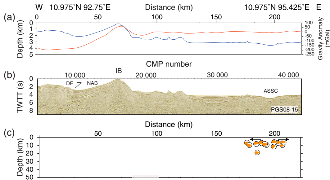
Figure 7. Profile PGS08-15: (a) Gravity anomaly (red) and bathymetry (blue), (b) seismic reflection image, and (c) hypocenters of earthquakes projected along profile in a 20 km wide zone along with their rotated fault plane solutions. DF: Diligent Fault, IB: Invisible Bank, NAB: Nicobar Andaman Forearc Basin, ASSC: Andaman Sea Spreading Center.
