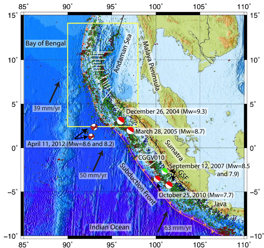
Figure 1. Map of the study area showing the Andaman-Sumatra Subduction zone and Andaman Sea Spreading Centre. Convergence directions and rates are shown with black arrows. Small circles represent earthquakes locations with hypocenter depth < 30 km (red), 30–60 km (green) and >60 km (blue). Focal mechanisms are also shown for seven large earthquakes of 21st century. White lines indicate the location of seismic profiles used in this study (15 profiles in the Andaman Sea; one profile (CGGV010) off of central Sumatra). The yellow rectangle marks the area of focus of this study, shown in Figure 2. GSF: Great Sumatra Fault.
