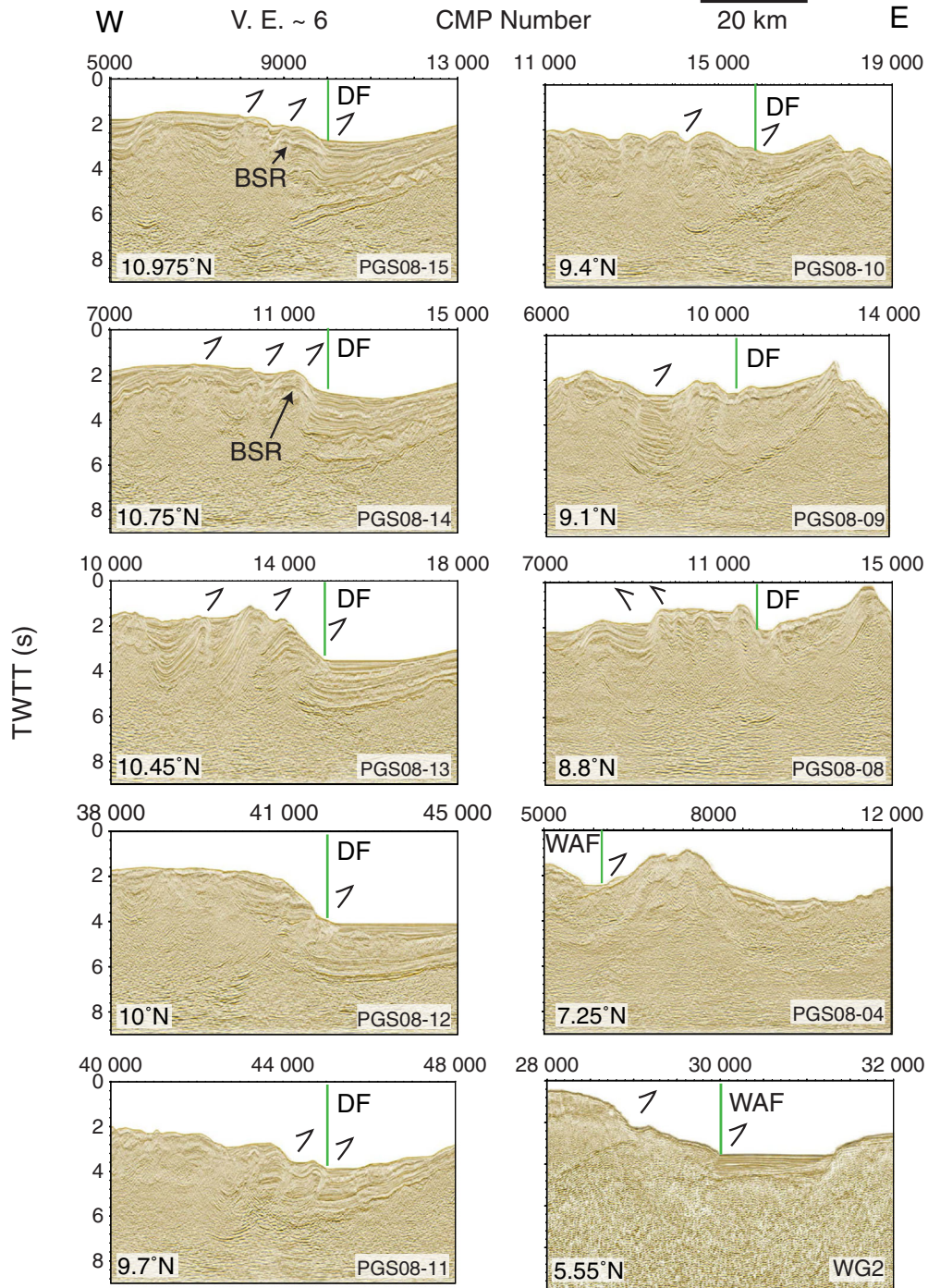
Figure 9. Seismic reflection images from north to south of the back thrust which has been interpreted as Diligent Fault (DF) in the north of Nicobar and West Andaman Fault (WAF) in the south. The green line indicates the surface arrival of the DF. BSR: Bottom-Simulating Reflector. All profiles are ~50 km long.
