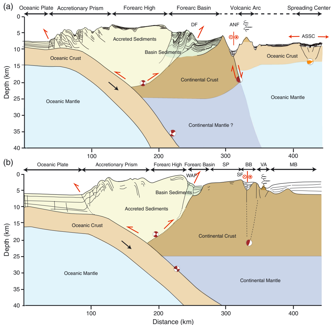
Figure 11. Summary sketch across the subduction zone from the oceanic plate to the back-arc basin down to 40 km depth (a) in the Andaman Sea (e.g., PGS08-12 to PGS08-15), and (b) off of northern Sumatra (e.g., WG2). Focal mechanisms are shown to illustrate the deformation and the orientation of the fault planes. DF: Diligent Fault, ANF: Andaman-Nicobar Fault, ASSC: Andaman Sea Spreading Center, WAF: West Andaman Fault, SF: Seulimeum Fault, BB: Breueh Basin, MB: Mergui Basin, SP: Sumatra Platform, VA: Volcanic Arc.
