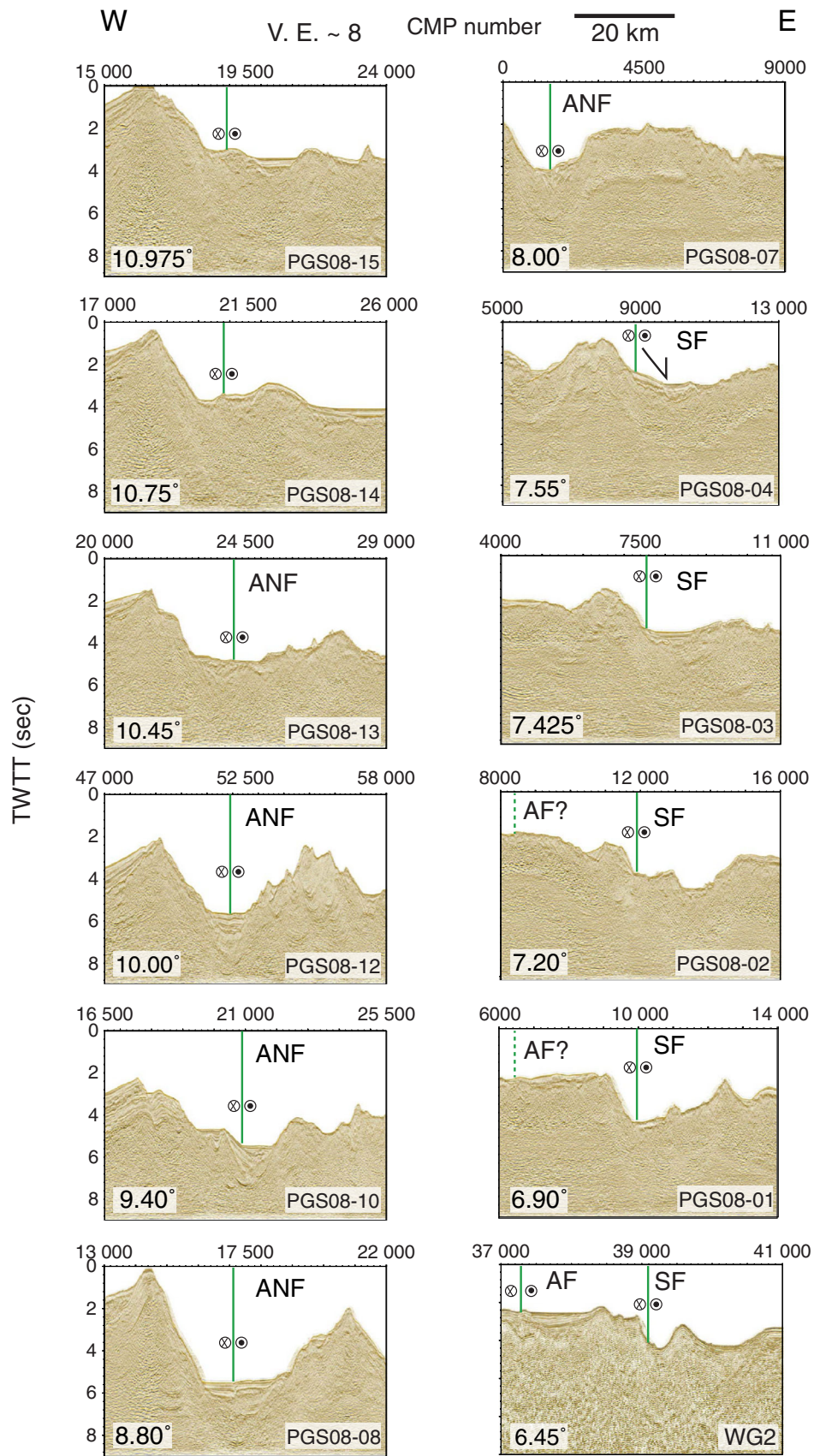
Figure 10. Seismic reflection images, from north to south, of the northward extension of the Great Sumatra Fault, which has been interpreted as Andaman-Nicobar Fault (ANF) north of Nicobar Island and the Aceh (AF) and Seulimeum Faults (SF) to the south. The green line marks the faults' surface arrivals.
