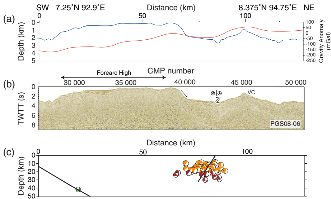
Figure 5. Profile PGS08-06: (a) Gravity anomaly (red) and bathymetry (blue), (b) seismic reflection image, and (c) hypocenters of earthquakes projected along profile in a 20 km wide zone along with their rotated fault plane solutions. The black lines indicate the approximate positions of the plate interface and back thrust. VC = Volcanic Cone.
