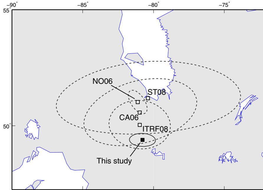
Figure 13. Map view of location and uncertainty of the Nubia-ITRF2008 rotation pole estimated here (solid line) and determined in other recent studies (dashed lines). Error ellipses are 95% confidence. ITRF08 = Altamimi et al. [2012]; ST08 = Stamps et al. [2008]; CA06 = Calais et al. [2006b]; NO06 = Nocquet et al. [2006]. Our result plots close to the ITRF2008 solution.
