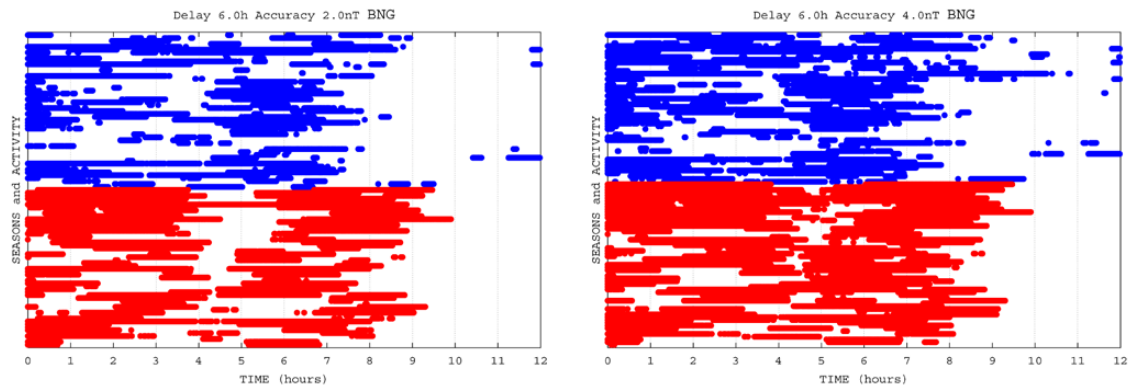
Fig. 11. Time table for BNG data, with t_0 = 6 h, \alpha = 2 nT (left panel) and \alpha = 4 nT (right panel) periods for the B_1(t) . Note the distinction between subsets \mathcal{D}_i and \mathcal{Q}_i : blue lines for disturbed days, red lines for quiet days. Yearly variation reads from top to down (starting with the first five days from January, up to the last five days of December, separately for \mathcal{D}_i and \mathcal{Q}_i sets).
