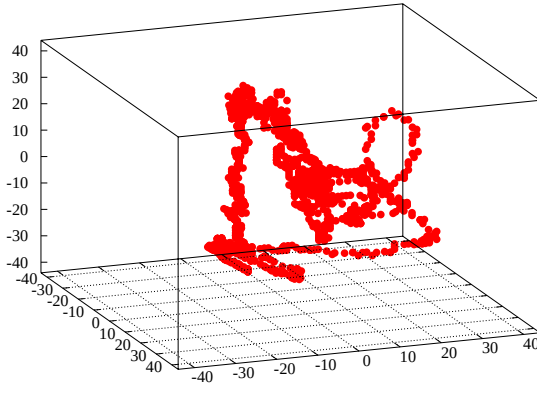
Fig. 2. Magnetic vector evolution (in nT) for the record CLF (6 September 1999): in 3-D frame centered to its mean (left panel), intensity only (right panel).
