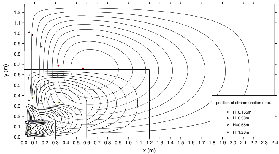
Figure 11. Streamfunction for variable H at t = 1000 s. The position of the streamfunction maximum is plotted by the diamonds. The position of this extremum tends towards x=y=H/2 for L/H \geq 2 . For clarity we plot the streamfunction for each height in the box with L/H \sim 2 . the streamfunction contours are for 10 equidistant intervals to the streamfunction maximum, with \psi_{\max} = 8 \cdot 10^{-6} , 3 \cdot 10^{-5} , 1.1 \cdot 10^{-4} , and 3.4 \cdot 10^{-4} for H = 16.5 , 33, 65, and 128 cm, respectively. The blue box in the lower left corner indicates the size of the smallest box used in this study. The largest box used in the study is twice as wide as the largest frame.
