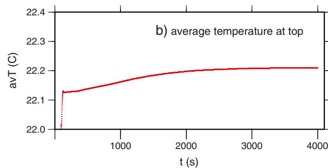
Figure 12. (a) Evolution until t = 4000 s of the streamfunction (a) in the smallest box ( H = 16.5 cm, L = 8.5 cm). After an initial apparent steady state with symmetrical streamfunction the pattern becomes asymmetric. (b) average temperature in a rectangle in the top left corner of 5 mm wide by 2 mm high.
