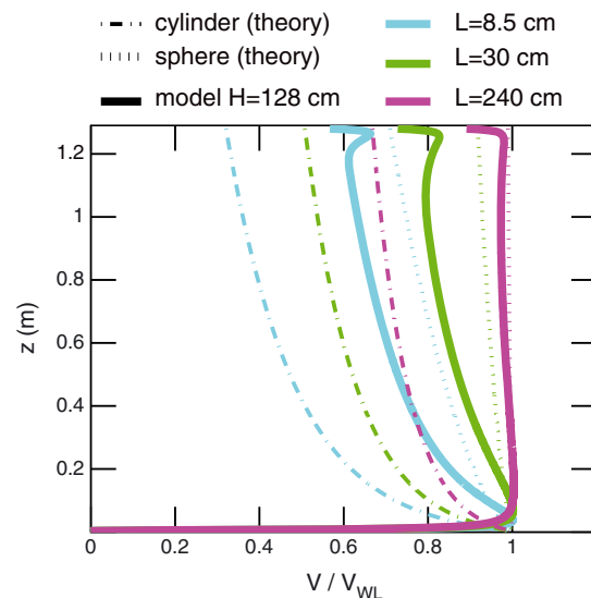
Figure 15. Comparison between V/V_{WL} observed in the open boundary simulations (solid lines) and the drag reduction predicted for a sphere (short dash lines [Happel and Brenner, 1973, pp. 318]) or for a cylinder (dot-dashed lines [Happel and Brenner, 1973, pp. 342]) for H = 128 cm.
