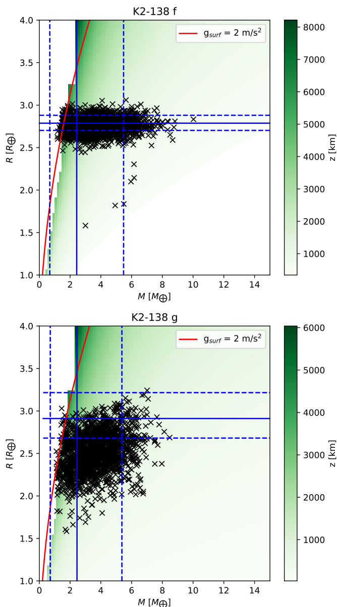
Fig. 3. Total mass and radius of K2-138 f (upper panel) and K2-138 g (lower panel) from the different realisations of the MCMC (black crosses). The solid blue lines show the mass and radius measurements from PASTIS, and the dashed lines give the related uncertainties. The red line indicates the limit below which the planet cannot maintain an atmosphere.
