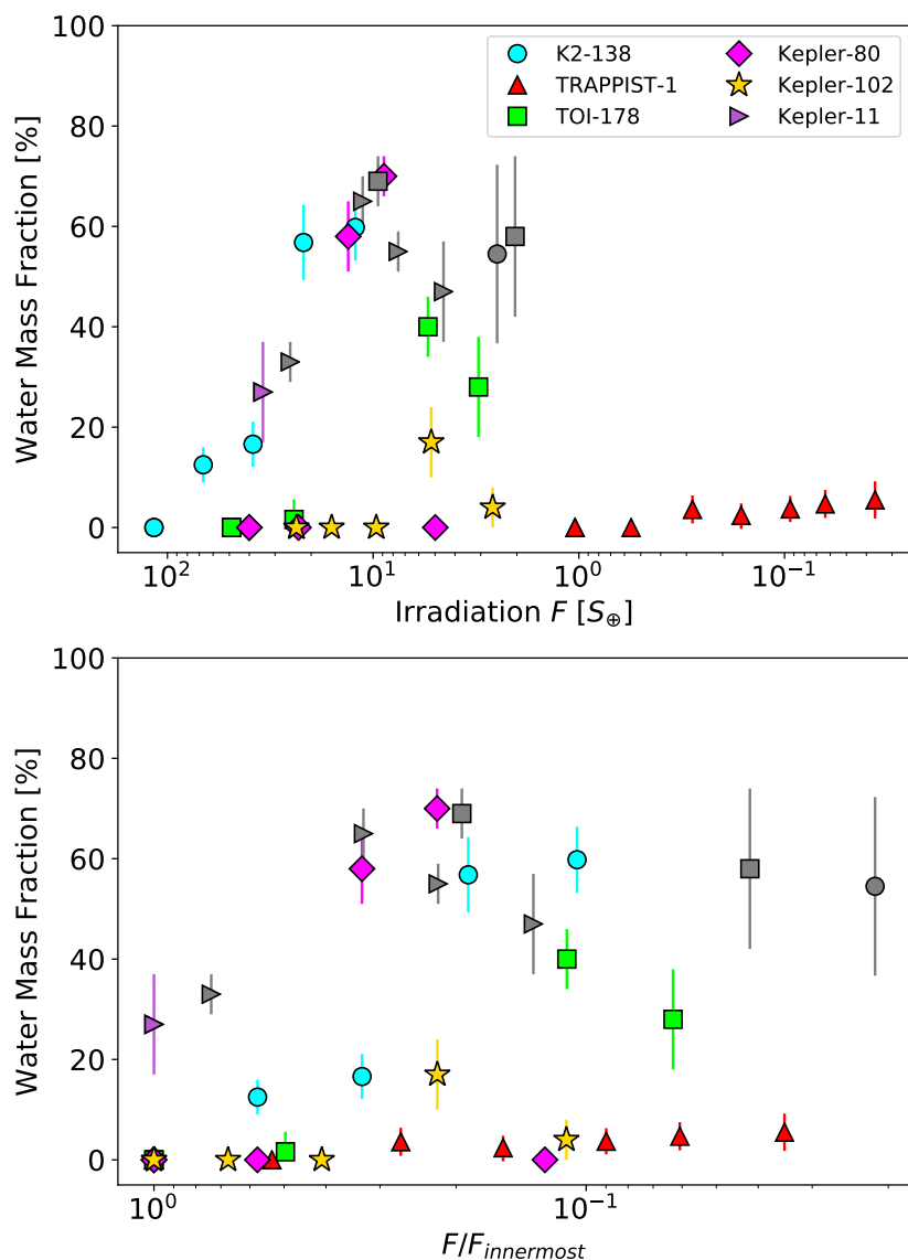
Fig. 4. Volatile mass fraction trends of the six multiplanetary systems analysed with our interior-atmosphere model. We show the water mass fraction estimates (see text) as a function of the stellar incident flux or irradiation, F , in Earth irradiation units ( S_{\oplus} = 1361 \text{ W/m}^2 ) in the upper panel. In the lower panel, the incident flux is normalised with respect to the inner, most irradiated planet in each system, F_{\text{innermost}} . Planets whose atmospheric composition is likely to be H/He-dominated instead of water-dominated ( d_{\text{obs-ret}} > 1 \sigma ) are indicated in grey color.
