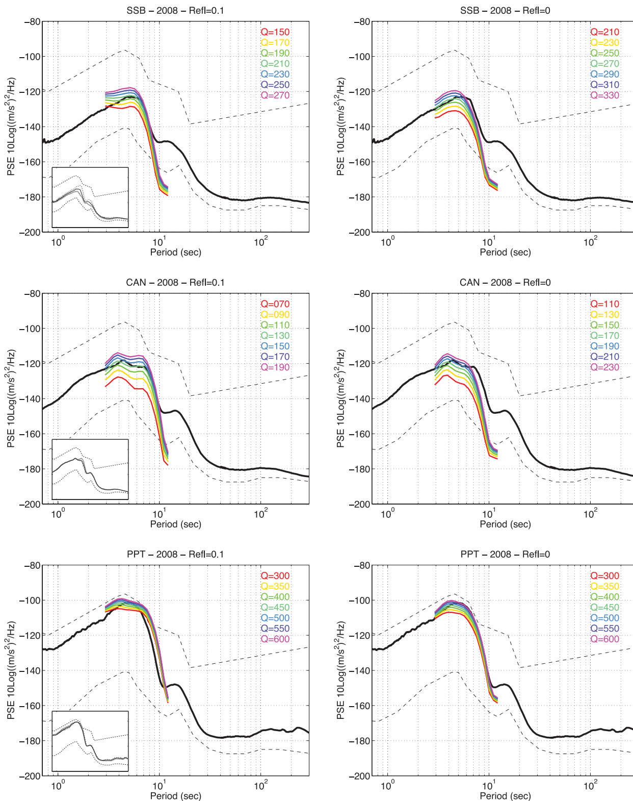
Figure 4. Real (black) and synthetic (colour) power spectra averaged over the year 2008 for two continental stations, SSB in France and CAN in Australia and an island station PPT in french Polynesia (Tahiti). Synthetic spectra are computed with the IOWAGA ocean wave model with (left-hand side, R^2 = 0.1 ) and without (right-hand side, R^2 = 0 ) ocean wave coastal reflection. Synthetic spectra are computed for different fixed attenuation Q whose value is written in colour on each plot. Inlets show averaged power spectra for 1 year (solid black line), January (dashed grey line) and August (solid grey line).
