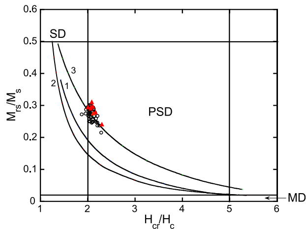
Figure 9. Day et al. [1977] plot of the hysteresis parameters: M_r , saturation remanence; M_s , saturation magnetization; H_{cr} , remanent coercivity; H_c , coercive force. SD, PSD and MD indicate single domain, pseudo single domain and multidomain fields, respectively, with the limits in Dunlop [2002a]. Curves 1–3 are theoretical SD + MD mixing curves from Dunlop [2002a, 2002b]. Results of samples from layers of geomagnetic excursions are denoted by red triangles while others are denoted by open circles.
