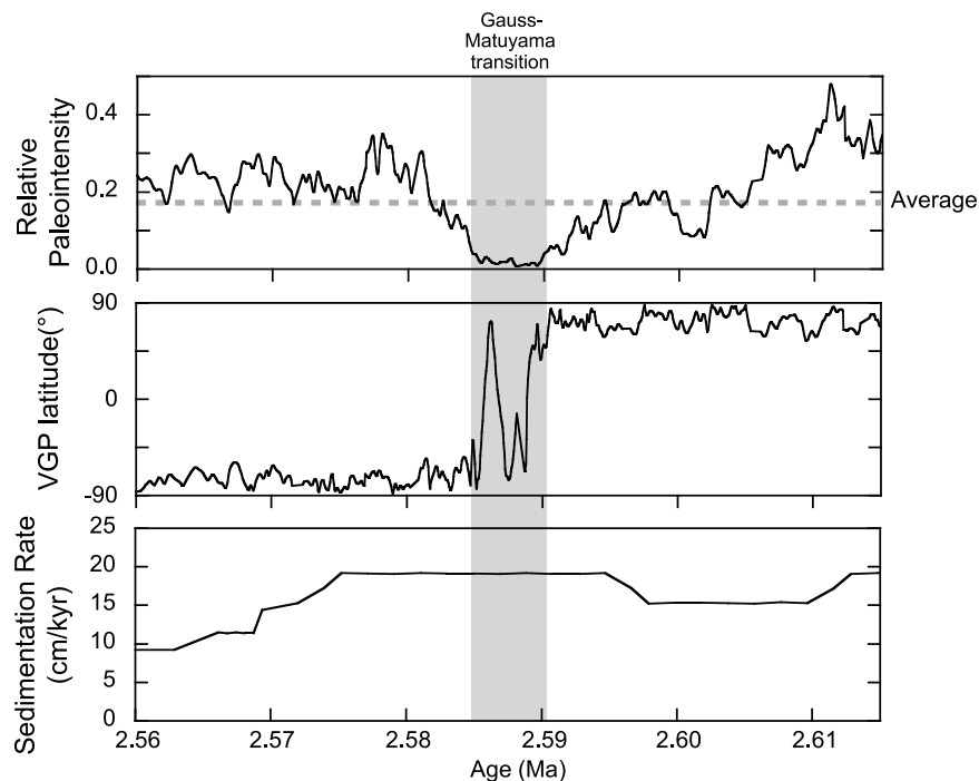
Figure 11. Relative paleointensity, the latitude of VGP, and the sedimentation rate of Site U1314 for the period including the G-M polarity transition.
