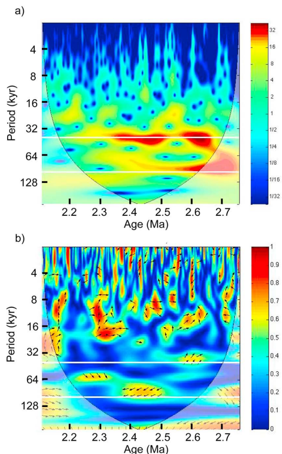
Figure 7. Results of wavelet analysis: (a) Wavelet power spectrum of ARM and (b) wavelet coherence between the paleointensity proxy (slopes of NRM intensity versus ARM intensity plot) and ARM. The white-shaded areas show the cone of influence in which edge effect due to ends of the signals cannot be ignored. Two horizontal white lines indicate periods of 41 and 100 kyr, respectively.
