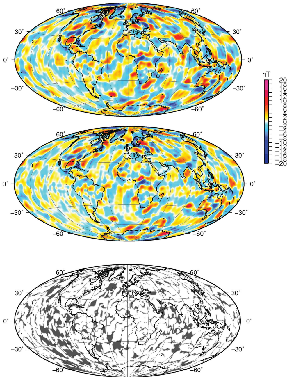
Figure 4. Radial component of the CM4 crustal field model (Sabaka et al. 2004) for SH degree 15–65 before (top panel) and after the filtering along a complete half-orbit (middle panel; see text for details). The bottom panel highlights the regions where the sign of the magnetic field was changed by the filtering process. Projections are Hammer-Aitoff.
