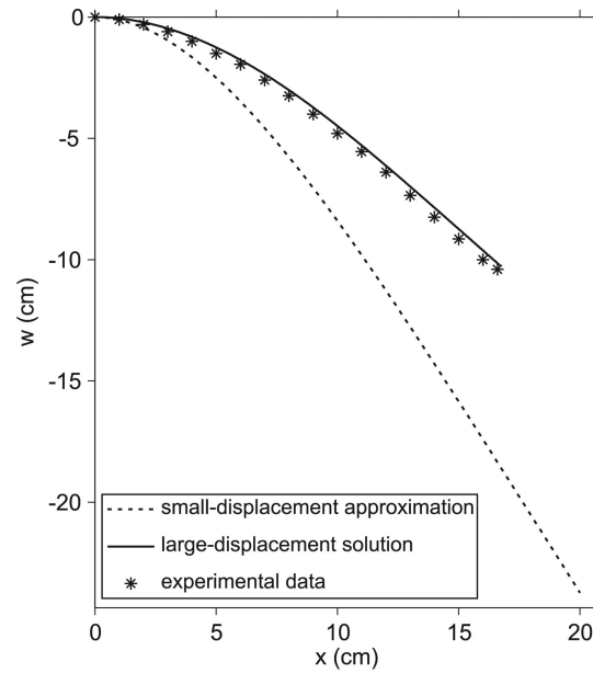
Figure 7. Flexure of an elastic plate bent under its own weight. The plate properties are L = 20 cm, h_p = 300 \mu\text{m} , \rho = 1296 \text{ kg m}^{-3} , E = 1.2 \text{ GPa} and \nu = 0.4 . Stars indicate measurements made with a laser positioning device. Theoretical predictions made with the small-displacement approximation (dashed line) and with beam equations for large deflections (continuous line) are shown. The small-displacement solution overestimates the vertical deflection and the plate length. Furthermore, it does not allow for the opening of a gap at the tip of the downgoing plate.
