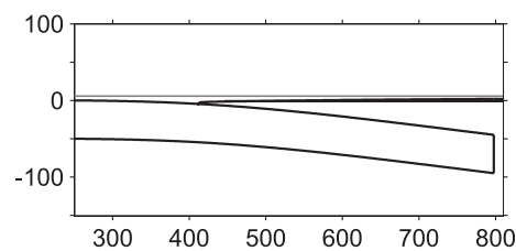
Figure 17. Calculated flexure of a buoyant plate ( (\rho_2 - \rho)/\rho_2 = +0.006 ) deflected by highly extended continental crust and mantle. The plate is 50 km thick, has a Young's Modulus of 100 GPa and is 20 \text{ kg m}^{-3} less dense than the mantle. The thin light grey line stands for the sea surface and stretched continental crust appears a thick black line.
