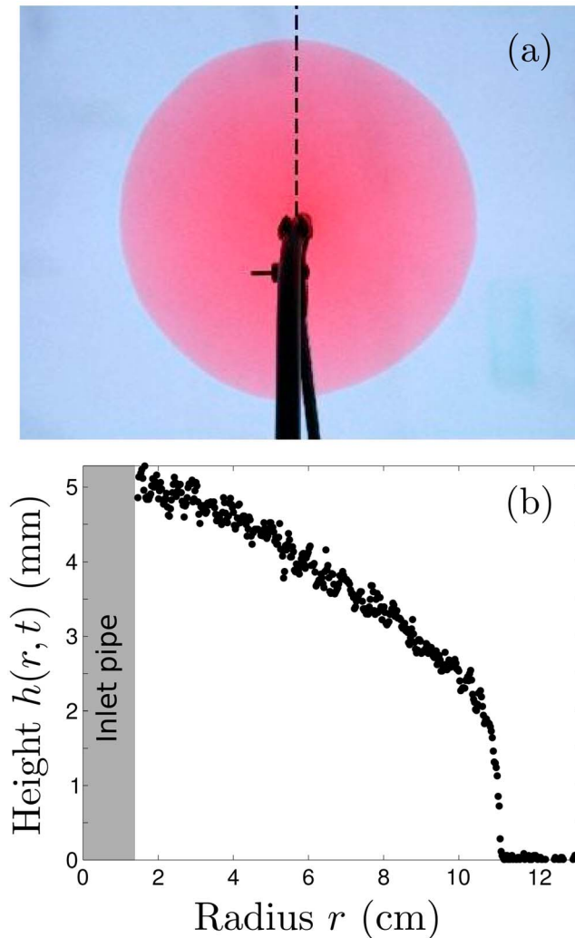
Figure A4. (a) Photograph of experiment M13, with the light transmitted through the thin polystyrene plate and an injection from above. (b) Height calculated using the colorimetric technique as a function of distance from the source on the profile (dashed line) shown in Figure A4a. The uncertainty on height measurements is around 0.2 mm. For each photograph, the height is retrieved from several profiles across the oil pancake.
