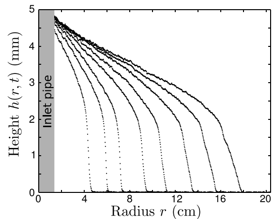
Figure B1. Advance and shape of the flow front with time for experiment M10. The different flow shapes are calculated by averaging several profiles across the pancakes at t = 69, 119, 169, 269, 369, 519, 669, and 844 s.
