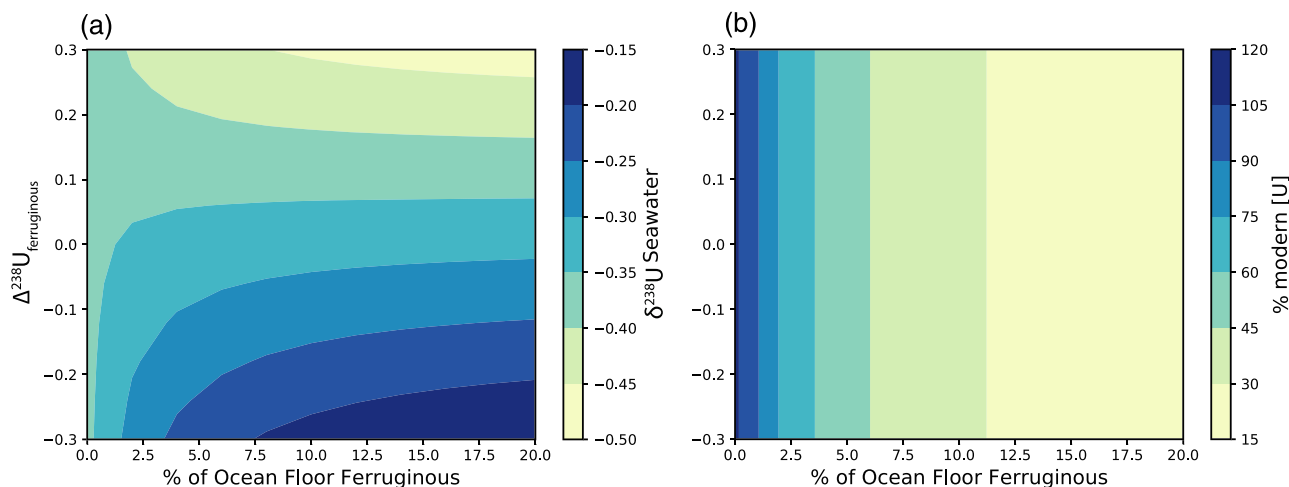
Figure 8. Isotope mass balance model outputs as result of varying \Delta^{238}\text{U}_{\text{ferr}} and area of ferruginous ocean floor. (a) Colorbar indicates \delta^{238}\text{U} value of seawater at steady state. (b) Colorbar indicates [U] in seawater expressed as a percentage of modern.
