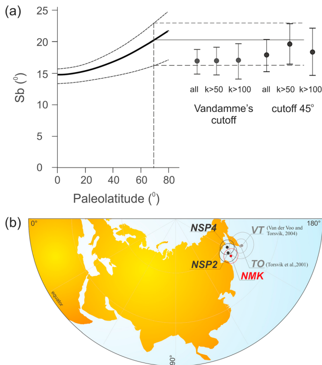
Figure 9. (a) Secular variations at the Permian-Triassic boundary as inferred from obtained data (black dots and corresponding error bars; Table 2) and their comparison with latitude dependence suggested by Biggin et al. (2008) on the basis of data, compiled by Johnson et al. (2008) for last 5 million years. Dashed curves represent 95% uncertainty. (b) Comparison of refined pole position (Norilsk-Maymecha-Kotuy, NMK) with location of previously suggested PT Siberian (NSP2 and NSP4; Pavlov et al., 2007) and European paleomagnetic poles (TO: Torsvik et al., 2001; VT: van der Voo & Torsvik, 2004). European poles are shown just for illustration; their comparison with new obtained PT Siberian pole lies beyond the scope of this paper.
