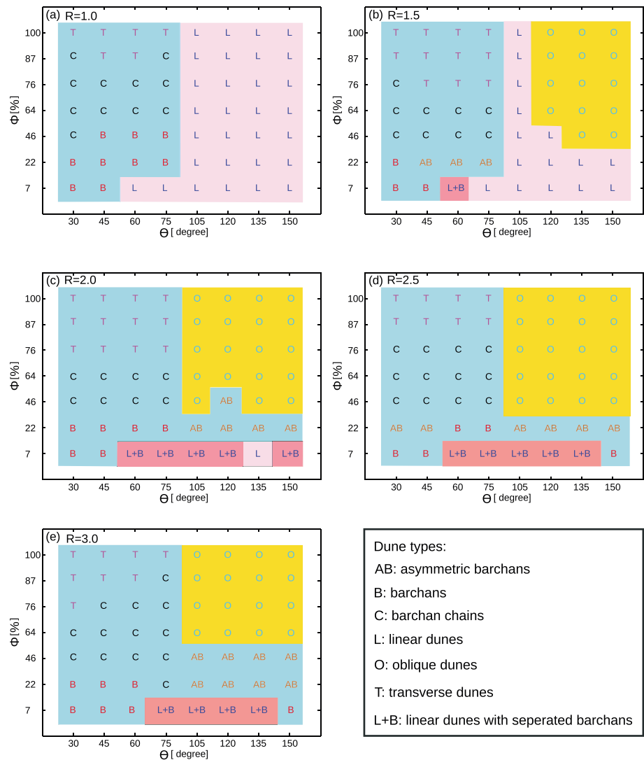
Figure 5. The morphological and orientative evolution of steady state dune types under different wind regimes and sediment availability. Dune types were similar for wind strength ratios of 2.5 and 3.0 with less than 10% sediment availability. In both cases, linear dunes and detached barchans coexisted, with barchans sometimes tracking linear dunes and sometimes situated on the same flank as linear dunes.
