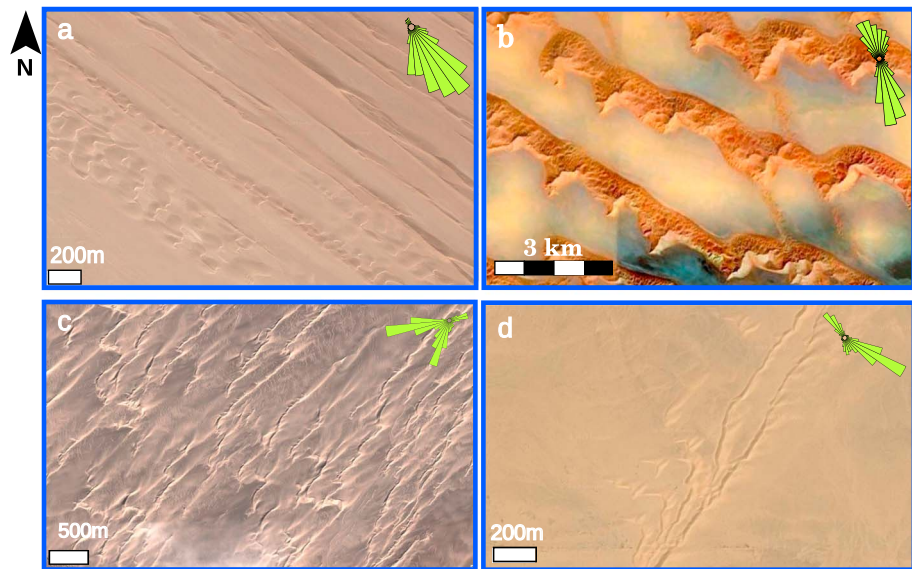
Figure 1. The coexistence of linear dunes and barchans (a) at the margins of the Chaerhan Salt Lake desert, China (37.023°N, 93.871°E); (b) the Rub' al-Khali desert, Saudi Arabia (20.85°N, 54.15°E); (c) northern of the Kumtagh desert (40.016°N, 91.812°E); and (d) northern of the Sahara desert (23.470°N, -5.442°E). Insets in (a)–(d) show the local flux roses based on 6-hr winds (above 5-m/s threshold wind speed at 10-m height) from the full period 1979–2016, and the roses show the direction of sand flux. Source: https://www.google.com/earth/ .
