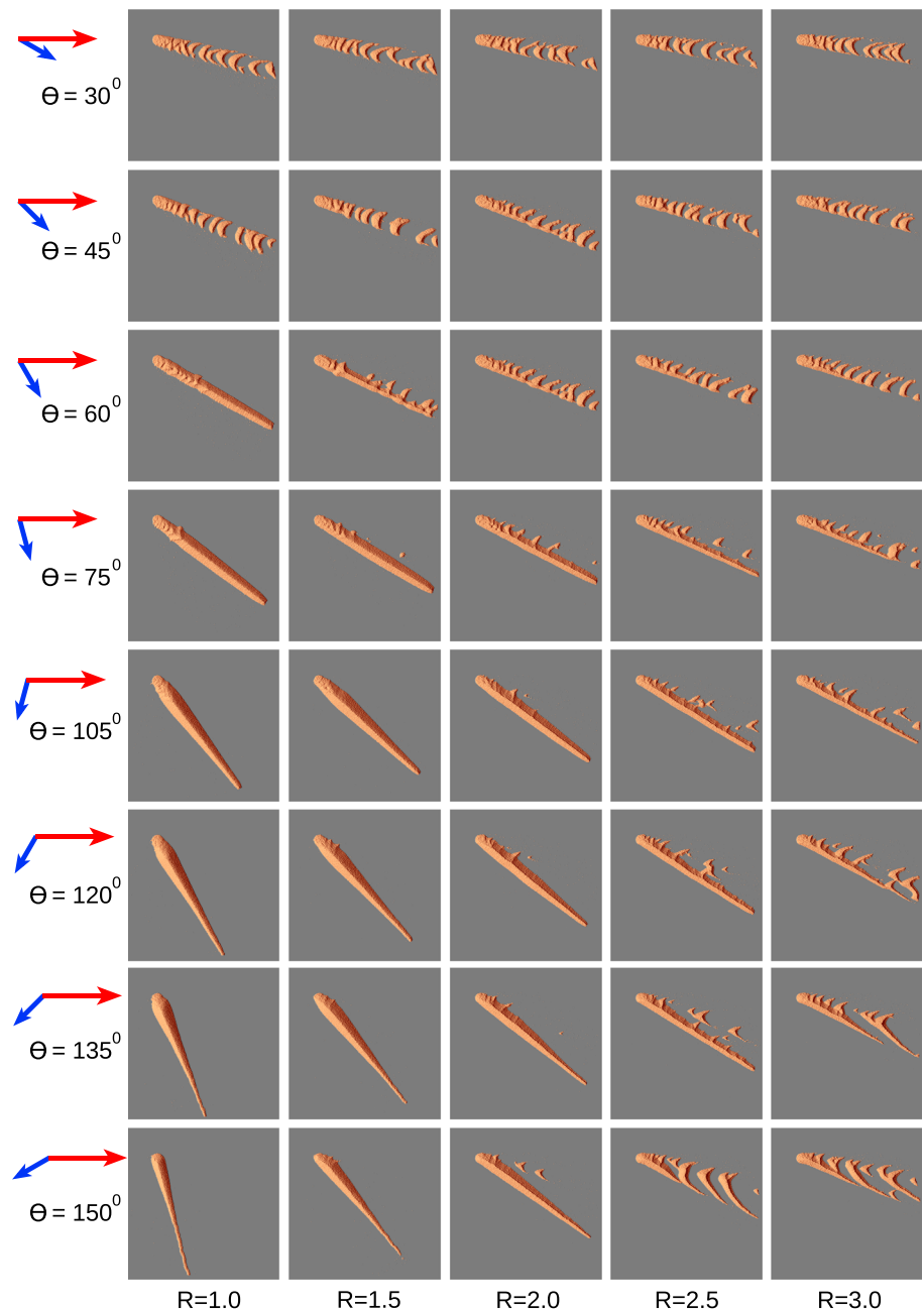
Figure 4. Evolution of dune morphology under conditions of limited sediment availability ( \Phi < 10\% ). R represents the wind strength ratio (i.e., wind strength on the left side of the figure divided by wind strength on the top of the figure). \theta represents the angle between the two wind directions, and the vector arrows represent a wind direction of R = 1.5 . ReSCAL software was used to produce images.
