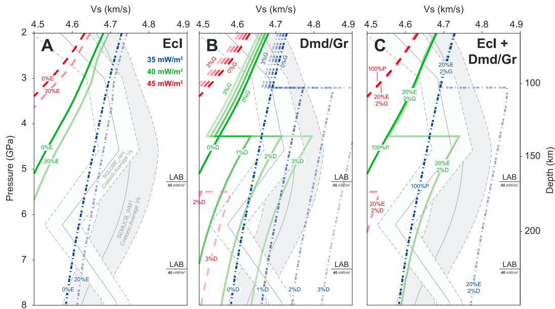
Figure 9. Results of peridotite \pm eclogite \pm diamond mixing models. See Text S1 for details of the mixing calculations, Figure 8 for individual, anharmonic lithologic V_s profiles, and Data Sets S4–S9 for anharmonic (elastic) velocities. All profiles are corrected for anelasticity with a 1 s period and 1 cm grain size (Jackson & Faul, 2010; Data Set S10), and are shown for the compositional “average” peridotite and eclogite (Figure S8; Table S1). Calculated V_s profiles from two shear-wave tomographic models are shown in each figure as gray shaded fields; note that these models are referred to 1 s periods, that is, identical to the anelasticity correction. In each panel, mixing results for the coolest geotherm that brackets xenolith thermobarometry (cf. Figure 7) are shown in blue dashed-dotted lines (35 mW/m 2 ), results for the intermediate geotherm are shown in green solid lines (40 mW/m 2 ), and results for the hottest geotherm are shown in red dashed lines (45 mW/m 2 ). (a) Two-component peridotite + eclogite mixing model results; only 20 vol.% eclogite is shown to account for neutral buoyancy constraints. (b) Results of two-component peridotite + graphite/diamond mixing models, with the position of the graphite to diamond transition determined by the geotherm (see text) and data from Day (2012). (c) Results of three-component peridotite + eclogite + diamond mixing models, showing the effect of combining \sim 20 vol.% eclogite with \sim 2 vol.% diamond or graphite.
