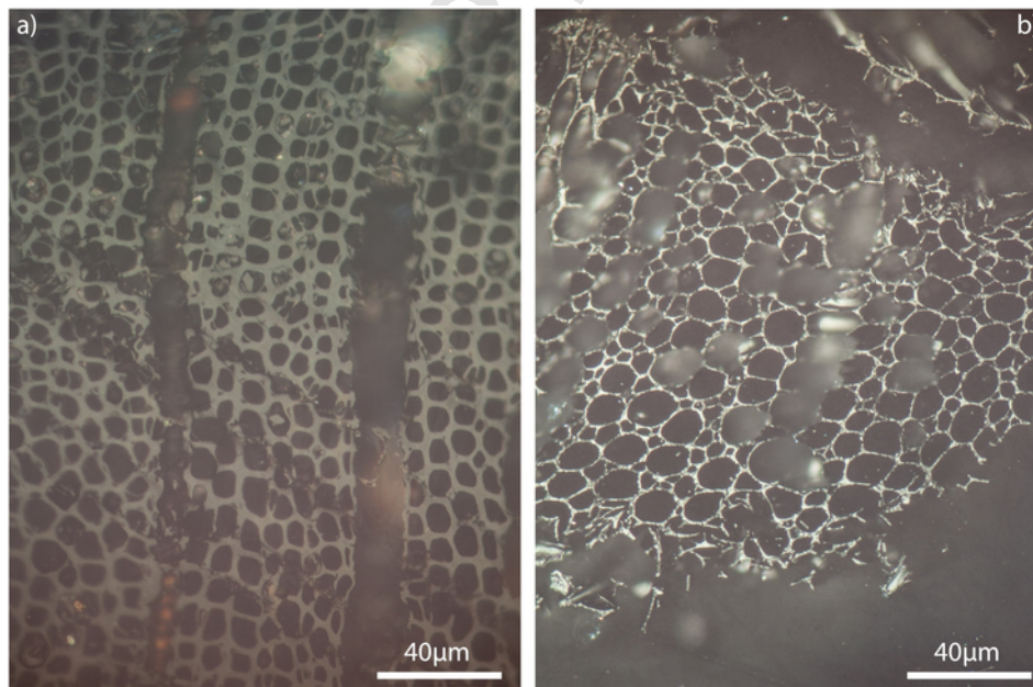
Fig. 3. Reflected light microphotographs of polished blocks under oil showing variable degree of charring. (a) Incompletely charred specimen (from site 270), as evidenced by the cell walls that are not completely homogenized (mean Ro%=0.36). (b) Fully charred fragment (from site 338) with high homogenized cell walls yielding mean Ro%=1.42.
