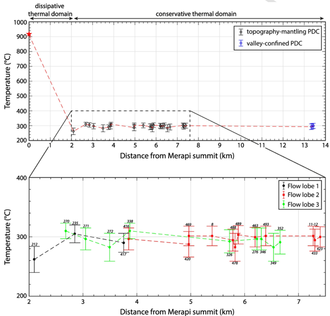
Fig. 6. Emplacement temperature variation as a function of the distance from source for the topography-mantling and co-genetic valley-confined PDC deposits of 5 November eruption. The red star marks the inferred initial temperature of the dome before the paroxysmal event as deduced from studies of the dome petrology and microtextures by Erdmann et al. (2016) and Preece et al. (2016). Inset plot shows an expanded view of the estimated temperatures of the topography-mantling PDC deposits. Colors refer to the main PDC flow lobes (see Fig. 1). Site numbers are in italics. (For interpretation of the references to color in this figure legend, the reader is referred to the web version of this article.)
