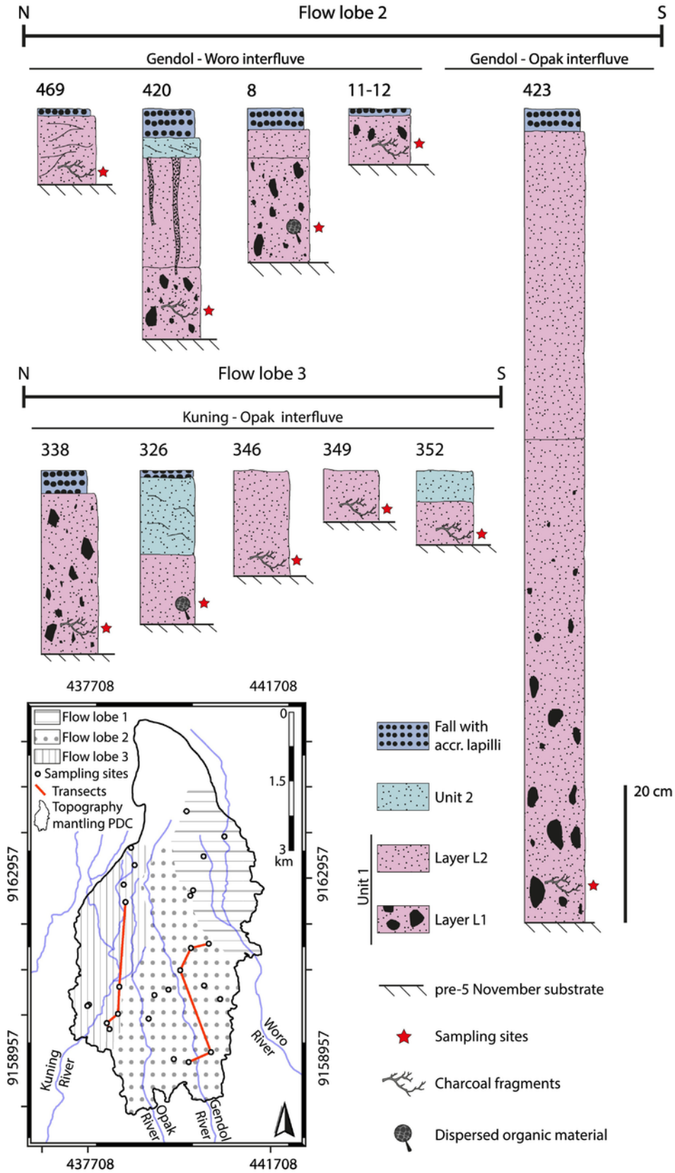
Fig. 2. Selected stratigraphic logs across the impact area of the topography-mantling PDC (refer to inset map for locations) modified after Komorowski et al. (2013), and position of the sampled charcoal fragments. In the absence of macroscopic (>1 mm) charcoal, dispersed organic material was found in bulk samples.
