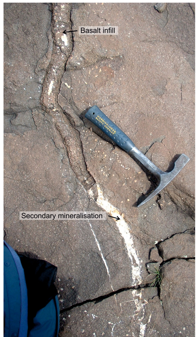
Fig. 10 Narrow termination of an axial cleft in a tumulus, partially infilled by the subsequent flow-lobe. Secondary mineralization has in-filled the vesicles within the lobe and the end of the cleft which was too thin to be filled with lava. 2470 m and 30.76000°S; 28.08335°E
