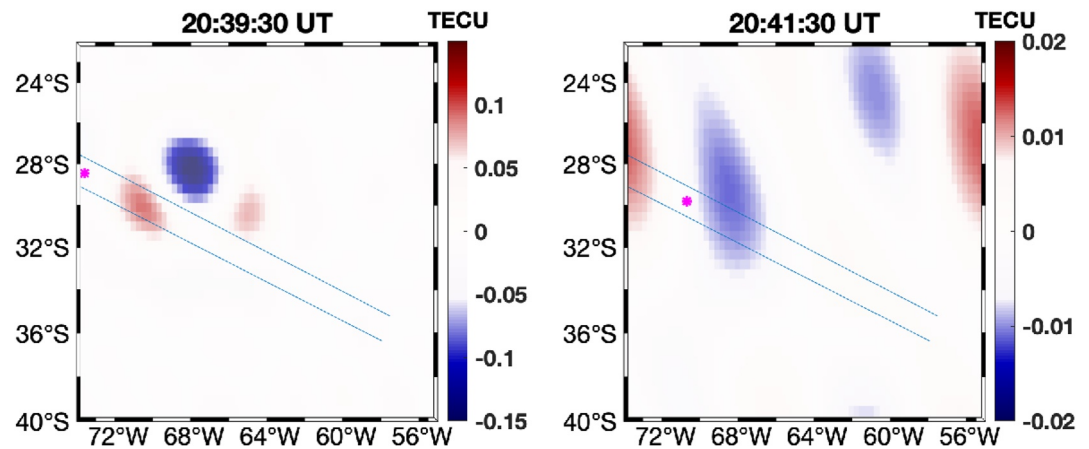
Figure 3. Right, identified traveling ionospheric disturbance (TID; period: 20–50 min, wavelength >200 km) back to the space-time domain (only the identified box in the omega-k diagram is sent back to space-time) for the larger grid with larger resolution (top left omega-k diagram). Results showed here are coherent with Figure 3 of Eisenbeis et al. (2019), related to the Great American Eclipse. Left, same as right plot but for the TID (period 25–120 min, wavelength <150 km).
