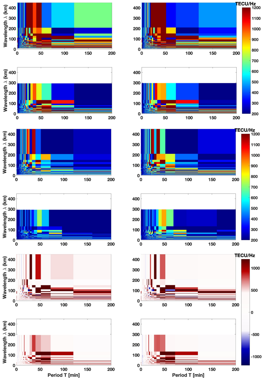
Figure 2. Top four plots, results of the omega-k analysis for the South American Eclipse. The diagrams show the wavelength over the period of the waves. Colors show the intensity for specific wavelengths and periods. We can clearly identify traveling ionospheric disturbances (TIDs) with a period of 20–50 min and a wavelength of >200 km for all different grids used. Displayed on the top are the results using a grid ranging from 74°W to 55°W in longitude and 40°S to 22°S in latitude, on the bottom from 72°W to 60°W in longitude and 36°S to 24°S in latitude. The number of cells varies from 40 in latitude and 70 in longitude for the plots on the left side to 140 cells in longitude and 70 cells in latitude for the right side. Middle four plots show the same results for the day before the eclipse and bottom four plots show the difference of the eclipse day and the day before the eclipse. Here, we can clearly highlight the TIDs with a wavelength >200 and <150 km for periods of 25–120 min.
