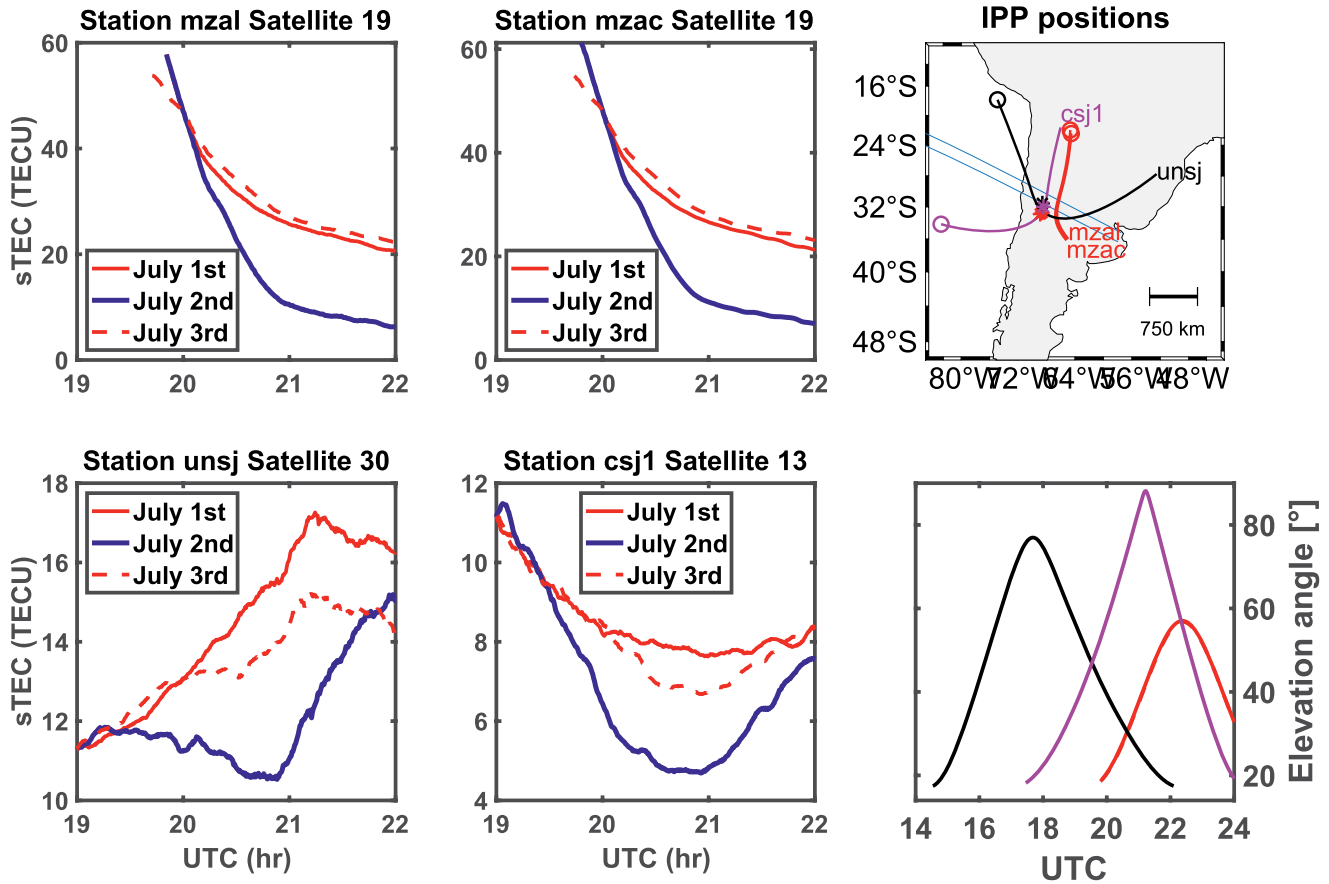
Figure 1. Top left and middle plots: absolute slant total electron content (sTEC) for stations MZAL (left) and MZAC (right) and Satellite 19 for the total solar eclipse (blue) and the surrounding days (red). Both stations lie in western Argentina where for the passing of Satellite 19 the eclipse acted like an early sunset. Bottom left and middle plots: Same absolute sTEC plots as above but for stations UNSJ (left) and CSJ1 (right) for Satellites 30 and 13. Right top plot: Time-space evolution of the IPPs for the station-satellite pairs shown in the four plots to the left. Same colors for same satellites: red for 19, black for 13, and magenta for 30. Positions of the stations (mostly colocated) is marked with an *, the start of the trajectory is marked with an o. Right bottom plot: Elevation angles of the satellite trajectories shown in the plot above.
