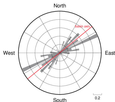
Figure 4. Rose diagram of ray path azimuths showing the striking directions of the higher modes. The red line indicates the basin axis.
