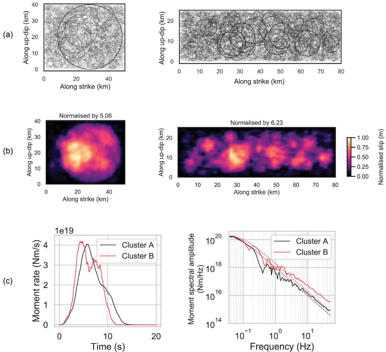
Figure 8. Comparison of source features of the two clusters shown in Fig. 6. (a) Comparison of cluster A (left-hand panel) and cluster B cases (right-hand panel) by subsurface distribution. (b) Same as a for final slip distribution. (c) Comparison of source–time function (left-hand panel) and moment spectra (right-hand panel) between cluster A (in black) and cluster B (in red) cases.
