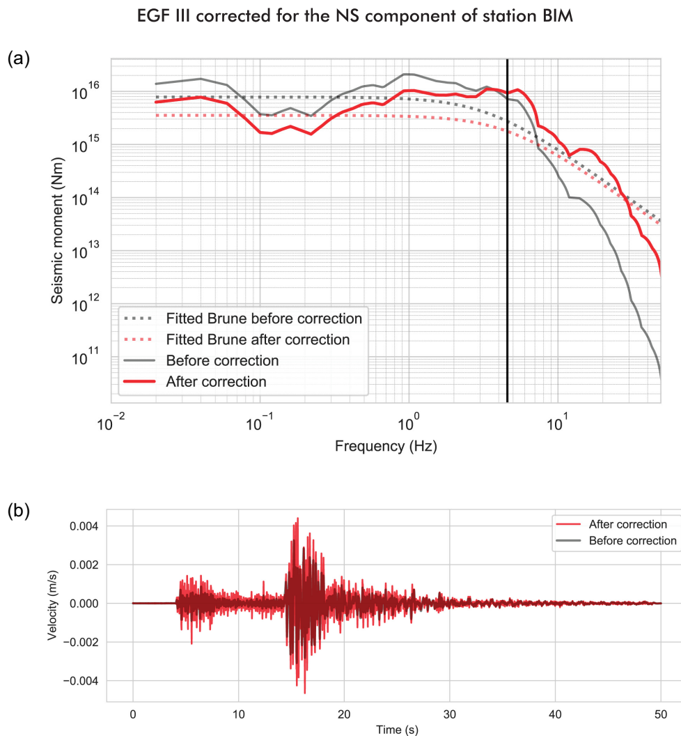
Figure 5. Example of EGF correction. (a) Moment spectra of the north-south component of EGF III signal at station BIM before and after correction. (b) Velocity-time histories before and after correction.
