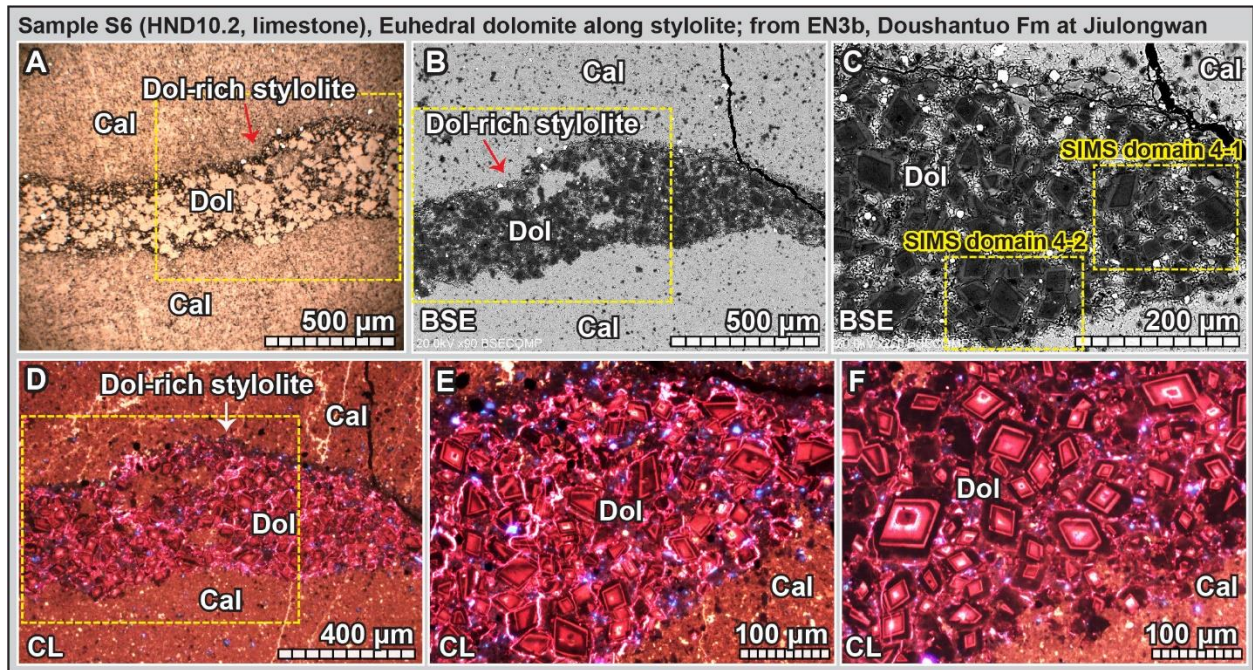
Fig. A11. Petrographic results of sample S6 (HND10.2). The dash boxes in A, B and D show the same views. (A) Optical microscopic image showing a dolomite-rich stylolite in a limestone sample under reflected light. (B) BSE image showing a dolomite-rich stylolite. (C) BSE image of the central right of image B. (D–F) CL images showing zoned dolomite crystals along stylolite.
