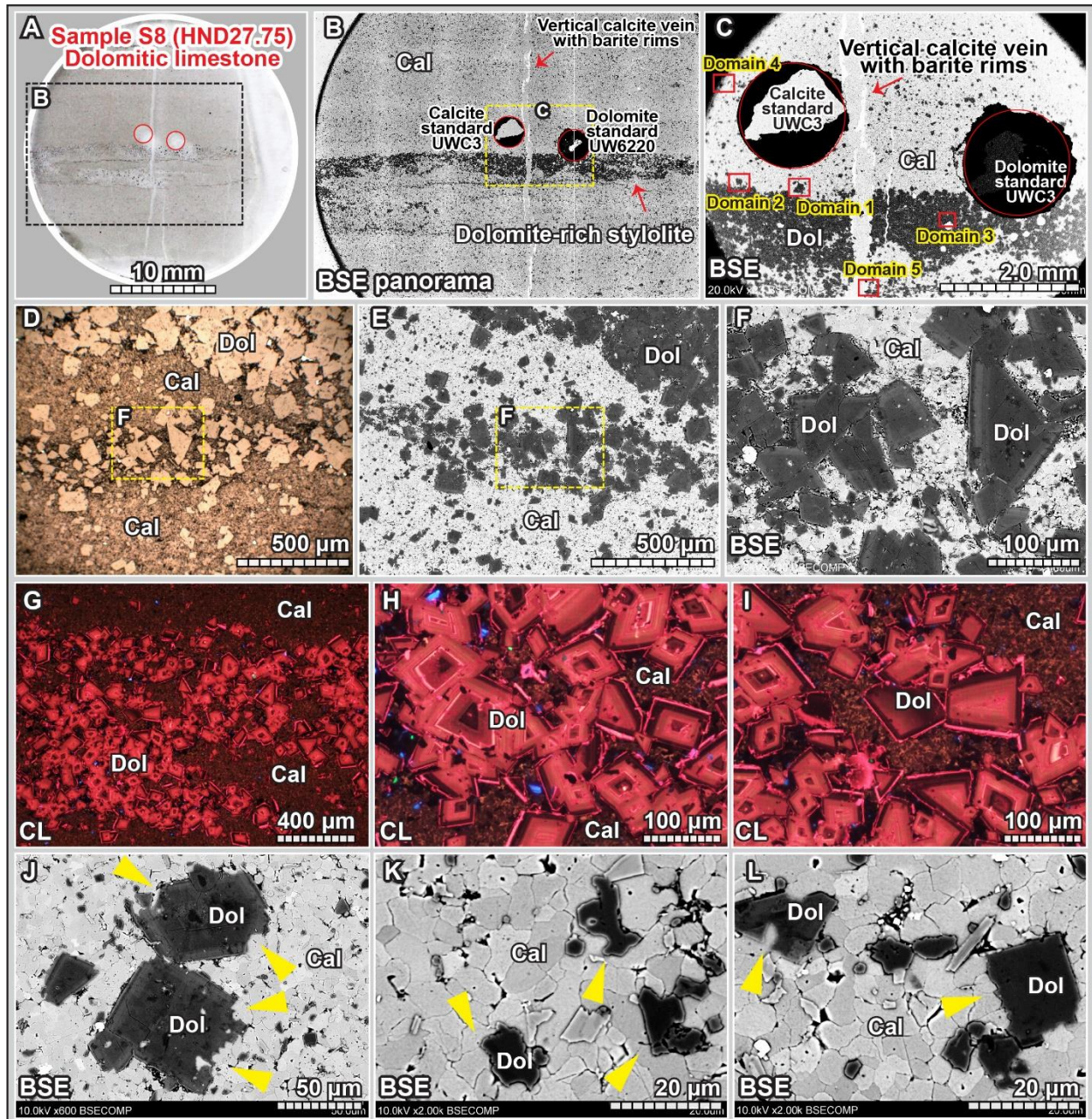
Fig. A13. Petrographic results of sample S8 (HND27.75). (A) SIMS thin section with WiscSIMS calcite standard UWC3 and dolomite standard UW6220 mounted in the center. (B) BSE panorama based on the integration of 6×6 individual BSE images. (C) A closer view of the dash box in B. Note the vertical calcite vein with barite rims. The thin barite rims are shown in the brightest color in the BSE images of this sample. (D–F) Petrographic images of dolomite along stylolite. (G–I) CL images show zoned dolomite crystals along stylolite. (J–L) Petrographic images of dolomite crystals in calcite matrix. Note that the dolomite crystals often show irregular
