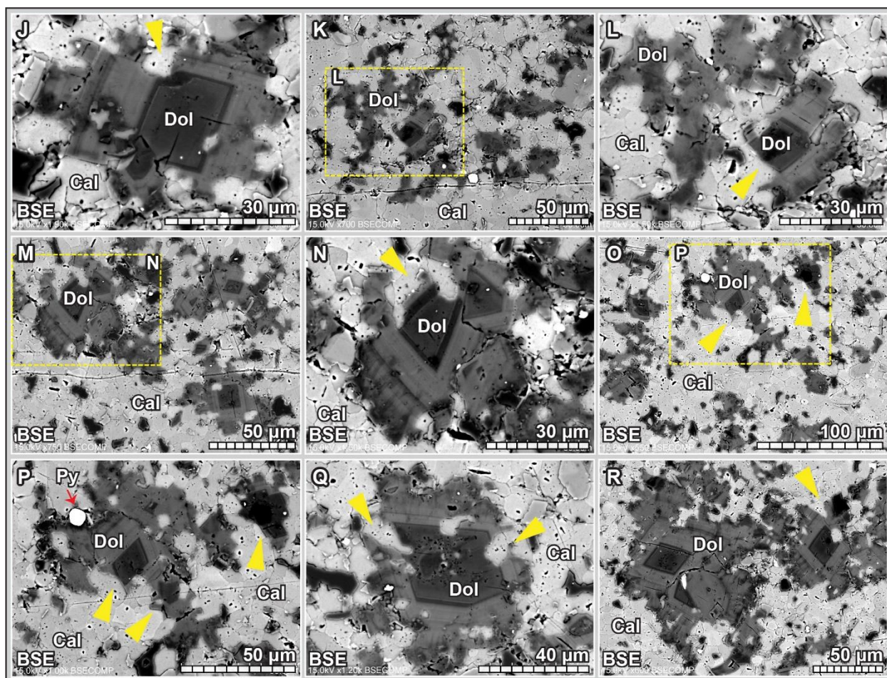
Fig. A10-2. (continued) (J–R) BSE images showing dolomite crystals in calcite matrix. Note that the dolomite crystals show irregular boundaries (arrows) with surrounding calcite microspar. Abbreviations: BSE = backscattered electron; Cal = calcite; Dol = dolomite.
