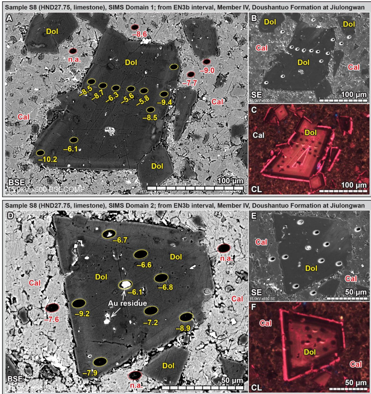
Fig. 12-1. Integrated SEM–CL–SIMS results of sample S8 (HND27.75). Values of \delta^{13}\text{C} are adjacent to 7- \mu\text{m} SIMS pits. (A–C) SIMS domain 1; (D–F) SIMS domain 2. (G–I) SIMS domain 3. (J–L) SIMS domain 4. (M–O) SIMS domain 5. The corrected \delta^{13}\text{C} data of spots on the dolomite crystal of domain 5 are not available due to the lack of corresponding EPMA data. See Fig. A13C for domain location. Abbreviations: BSE = backscattered electron; SE = secondary electron; CL = cathodoluminescence; Cal = calcite; Dol = dolomite.
