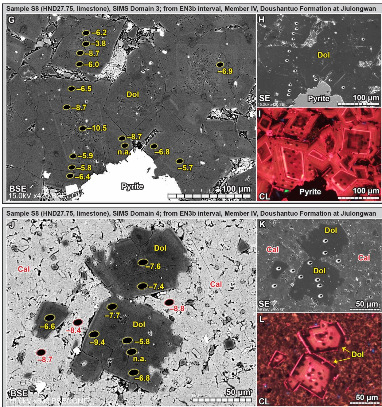
Fig. 12-2. (continued) (G–I) SIMS domain 3. (J–L) SIMS domain 4. (M–O) SIMS domain 5. Values of \delta^{13}\text{C} are adjacent to 7- \mu\text{m} SIMS pits. The corrected \delta^{13}\text{C} data of spots on the dolomite crystal of domain 5 are not available due to the lack of corresponding EPMA data. See Fig. A13C for domain location. Abbreviations: BSE = backscattered electron; SE = secondary electron; CL = cathodoluminescence; Cal = calcite; Dol = dolomite; n.a. = not available.
