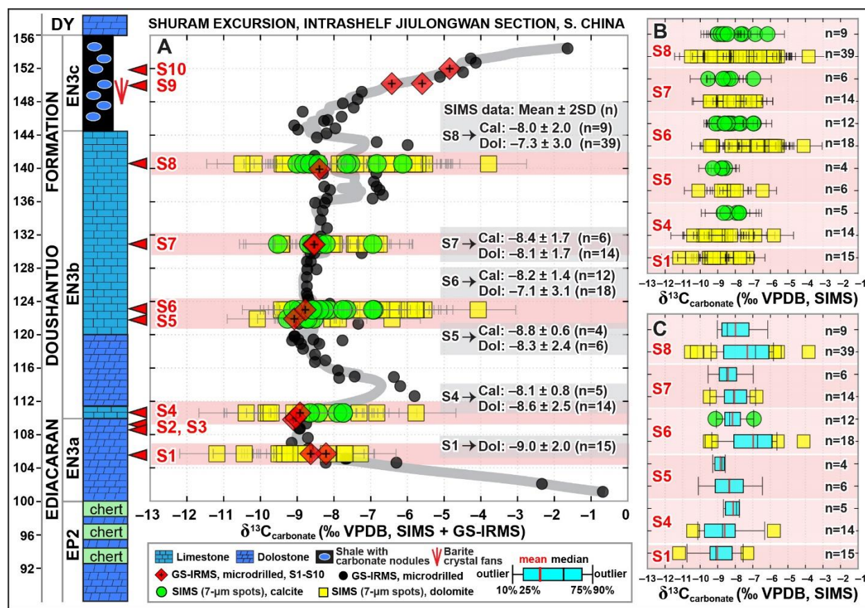
Fig. 5. (A) Integrated lithological and chemostratigraphic \delta^{13}\text{C}_{\text{carb}} results of the Shuram Excursion (i.e., EN3 interval) in the upper Doushantuo Formation at Jiulongwan, South China. Filled black dots represent \delta^{13}\text{C}_{\text{carb}} data analyzed from microdrilled powders by GS-IRMS, with the data for samples also analyzed by SIMS highlighted as red diamonds. Green circles and yellow boxes represent SIMS data analyzed from calcite and dolomite, respectively. Error bars show reproducibility as 2 standard deviations of the bracketing analyses on WiscSIMS standard UWC3. Gray curve represents three-point running average based on the GS-IRMS data. Data source: GS-IRMS data (McFadden et al., 2008); SIMS data (this study). (B) Plot of each individual SIMS sample, with \delta^{13}\text{C}_{\text{calcite}} and \delta^{13}\text{C}_{\text{dolomite}} data offset vertically to improve clarity. (C) Box plots of the SIMS \delta^{13}\text{C}_{\text{calcite}} and \delta^{13}\text{C}_{\text{dolomite}} data. Note that the mean values of \delta^{13}\text{C}_{\text{calcite}} and \delta^{13}\text{C}_{\text{dolomite}} for each sample are identical within uncertainty. The number of SIMS analysis (n) is also provided. Abbreviations: EN = Ediacaran negative excursion; GS-IRMS=gas-source isotope ratio mass spectrometer; SIMS = secondary ion mass spectrometer; SEM = scanning electron microscope; VPDB = Vienna Pee Dee Belemnite; Cal = calcite; Dol = dolomite.
