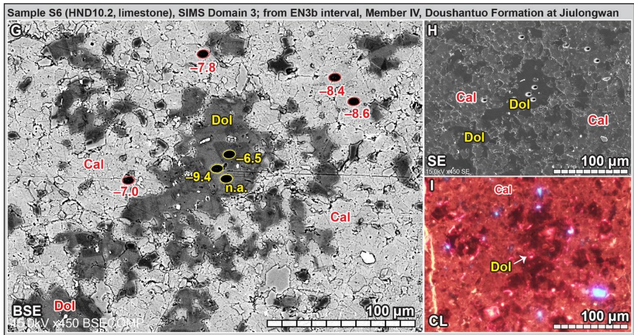
Fig. 9-2. (continued) (G–I) SIMS domain 3. Note that the dolomite crystals show irregular boundaries (arrows) with surrounding calcite microspar. Values of \delta^{13}\text{C} are adjacent to 7- \mu\text{m} SIMS pits. See Fig. A10B for domain location.
