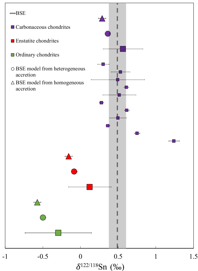
Figure 8. Isotopic compositions of core formation models computed for different types of possible building materials compared to the bulk silicate Earth (BSE) value (Badullovich et al., 2017) in dashed line with uncertainty in gray. Average isotopic compositions of carbonaceous chondrites (purple), enstatite chondrites (red) and ordinary chondrites (green) from Creech and Moynier (2019) are plotted as large squares displaying the standard deviation between single meteorites measurements. Individual measurements of carbonaceous chondrites are represented as small purple squares. Multiple isotopic core formation models were computed using each of the average chondrites \delta^{122/118}\text{Sn} as the isotopic composition of Earth's building blocks. For each chondrite type, a homogeneous accretion model with an \epsilon and k = 0.5 was calculated and represented as a triangle. A heterogeneous model where all the volatiles were brought in the last 10% of Earth's accretion, considering an \epsilon value and k = 0.5 , is represented as a circle. Error bars of the models correspond to the propagation of uncertainty on the regression parameter. The isotopic composition of carbonaceous chondrites overlap with that of the BSE. The modeled \delta^{122/118}\text{Sn} of the BSE are lower than the \delta^{122/118}\text{Sn} from the chosen building block because the heavier isotopes of Sn tend to go preferentially in the core. Models detailing carbonaceous chondrite isotopic compositions generate models that are closer to the BSE than for other potential source materials. Moreover, individual Sn isotopic measurements of carbonaceous chondrites (small purple squares) overlap with that of the BSE (with notable dispersion), and both overlap with our heterogeneous model. Based on this evidence, carbonaceous chondrite-like material appears to be the best potential source of volatile elements on Earth.
