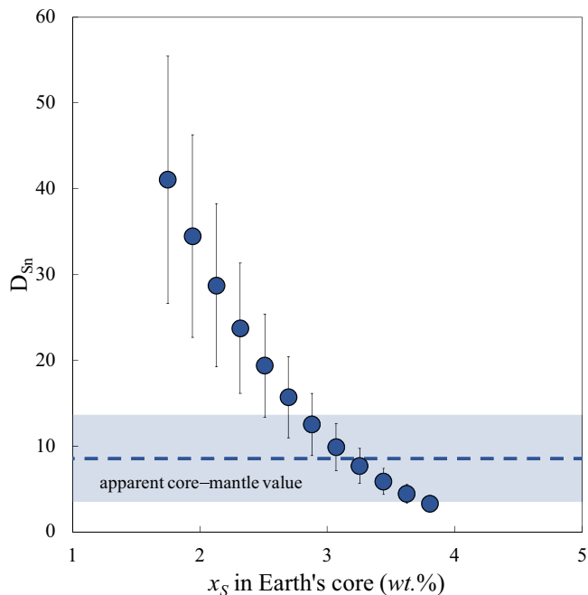
Figure 6. Heterogeneous partial equilibration core formation models. The final D_{\text{Sn}} is plotted for a range of different S concentrations that are forced into the Earth's core. D_{\text{Sn}} is computed in the case of a late accretion of Sn and S in the last 10% of Earth's formation, using an \epsilon and with k = 0.5 . In this calculation the bulk S content of the accreted embryos are entered as input and the X_{\text{S}} in the cores of the embryos and Earth are computed using multilinear regression equation from Rose-Weston et al. (2009) which describes the experimentally determined behavior of S in a metal-silicate equilibrium. It shows that if there is 3 wt.% of S in the Earth's core, the apparent partitioning of Sn, plotted as a blue dotted line, can be perfectly reconciled with the computed partitioning inferred from experimental data.
