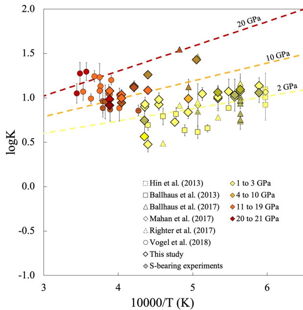
Figure 4. LogK determined experimentally as a function of reciprocal temperature for all experiments of this study and data compiled from literature (Ballhaus et al., 2013, 2017; Hin et al., 2013; Mahan et al., 2017; Righter et al., 2017; Vogel et al., 2018). Errors correspond to one standard deviation \sigma and were propagated from EPMA and LA-ICPMS measurements of this study and from literature. Experiments containing more than 1 mol% of S in the metal are represented with a horizontal lines pattern. All experiments are color-coded according to their pressure: 1–3 GPa in yellow, 4–10 GPa in orange, 11–19 GPa in light red, >19 GPa in dark red. Multilinear regression fits are also displayed at IW-2 in several conditions: 2, 10, and 20 GPa with no S in the metal. LogK being defined as a + b \frac{1}{T} + c \frac{P}{T} , this figure displays the effect of pressure and temperature alone on Sn partitioning between metal and silicate.
