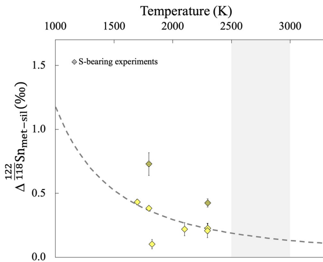
Figure 7. Sn isotope fractionation between metal and silicate from a selection of piston cylinder experiments at 2 GPa as a function of the equilibrium temperature of those experiments. This fractionation is a function of 1/T^2 (Urey, 1947) as represented by the gray dashed regression. A fractionation between 0.10 and 0.73‰ is observed. S-bearing experiments, represented with a horizontal lines pattern, seem to present a higher fractionation of Sn isotopes between metal and silicate. The gray zone corresponds to temperatures that are relevant to the conditions of core–mantle differentiation in a deep magma ocean on Earth. The interpolation of the regression based on experimental data at such temperatures shows that isotopic fractionation could be observed at Earth's differentiation conditions.
