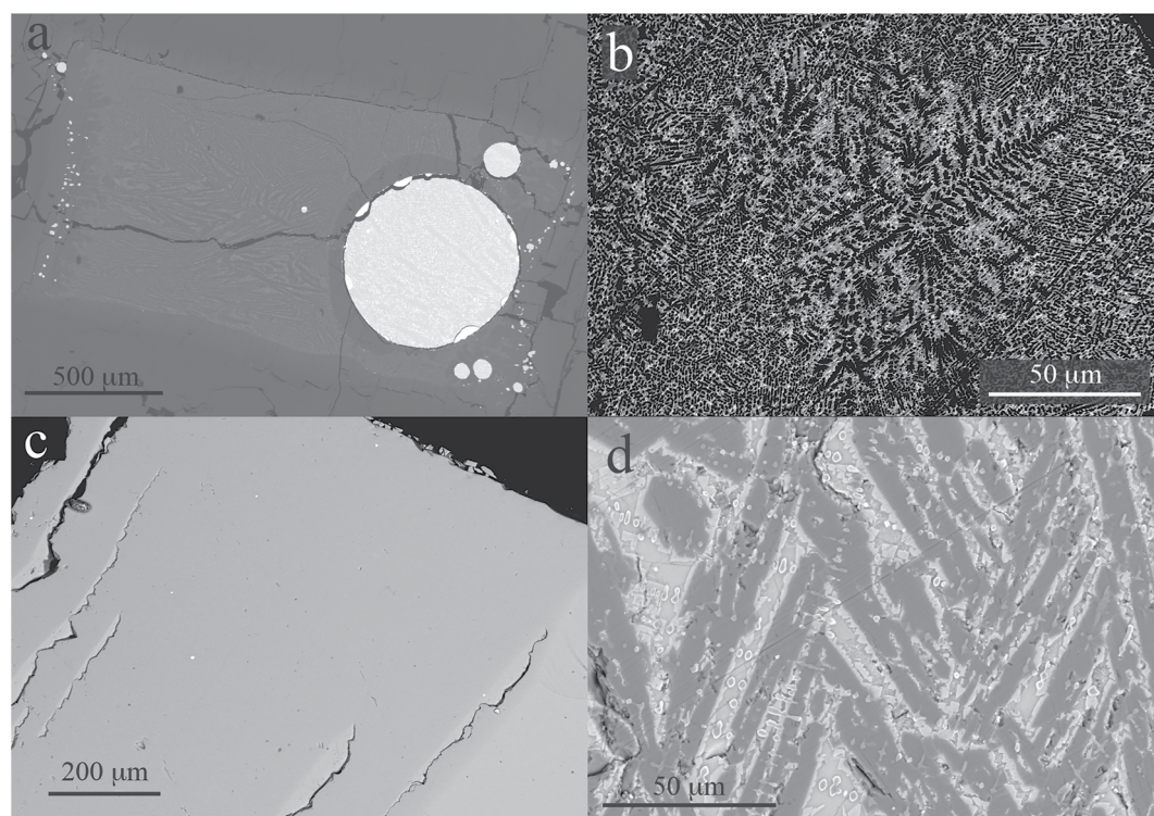
Figure 1. Back-scattered electron images from typical multianvil and piston cylinder run products. (a) Image of H4950 multianvil experiment (12 GPa, 2,273 K). The average composition of both phases are measured with 30 \mu\text{m} rasters on the electron microprobe, and a 90 \mu\text{m} beam size for laser ablation in order to homogenize quench textures in the metal and in the silicate that correspond to local chemical heterogeneities. (b) Image of metal phase (piston cylinder, 2 GPa, 1,797 K) showing dendritic quench texture. (c) Image of silicate phase of run 268 (piston cylinder, 2 GPa, 1,823 K) typical of low temperature, boron nitride encapsulated runs showing clean glass with a few \sim 1\ \mu\text{m} metal nuggets. (d) Image of silicate phase of run 272 (piston cylinder, 2 GPa, 2,296 K) showing typical quench textures for high temperature MgO-encapsulated experiments with dendritic olivine crystals and interstitial pyroxenite glass (brighter gray).
