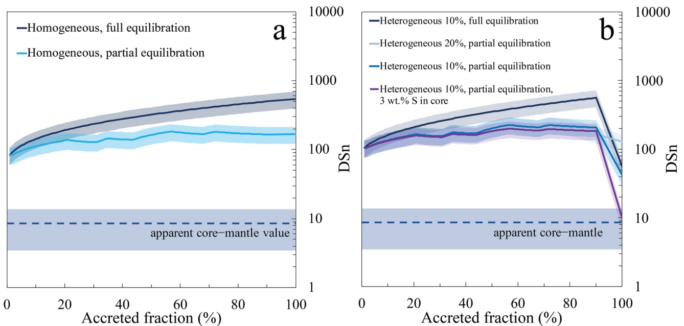
Figure 5. Evolution of D_{Sn} during Earth's accretion computed from core formation models with full and partial equilibration and 1.8 wt.% S in the core of the final Earth. (a) Tin partitioning with continuous and homogeneous core formation models with full and partial equilibration. For partial equilibration, \epsilon was computed with k = 0.5 . The final D_{Sn} displayed for Earth are respectively 544 \pm 145 and 167 \pm 45 . The use of an \epsilon is lowering significantly the partitioning of Sn, but the final values are too high to be compared to the observed Sn partitioning on Earth ( 8.56 \pm 5.07 ), shown as a dotted line on the figure. (b) Tin partitioning as a function of the percentage of accreted Earth computed from continuous heterogeneous core formation models in which all the Sn and S were brought in the last 20% or in the last 10% of Earth's accretion in order to simulate a late accretion stage. The obtained final D_{Sn} are lower than in the scenario presented in (a): 128 \pm 34 for the light blue curve which represents a 20% late accretion stage with partial equilibration, 55 \pm 15 for the dark blue curve corresponding to a 10% late accretion stage with full equilibration, 42 \pm 11 for the blue curve which shows a 10% late accretion stage with partial equilibration, using an \epsilon with k = 0.5 , and 9.9 \pm 2.6 for the purple curve representing a model identical to the previous one with 3 wt.% of S in the core. The partitioning is still distinct from the observed value shown in dotted line ( 8.56 \pm 5.07 ) except when more S is brought into the core. In those models we used a succession of planetesimals of different sizes to be accreted at each steps: 0.1, 1, 10, and 20 wt.% of the Earth's total mass. In calculations considering a partial equilibration, the partitioning coefficients are sensitive to the size of the accreted embryos which is why we observe variations on the curve at stages where there is a change of size of accreted bodies.
