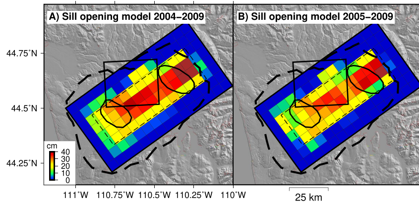
Figure 5. Distributed sill opening models for 2004–2009 (a) and 2005–2009 (b). The thin and dashed rectangles are the NGB and the caldera sources with uniform opening. The thick dashed line is the caldera border and the elliptical lines show the Sour Creek (SCD) and Mallard Lake (MLD) domes.
