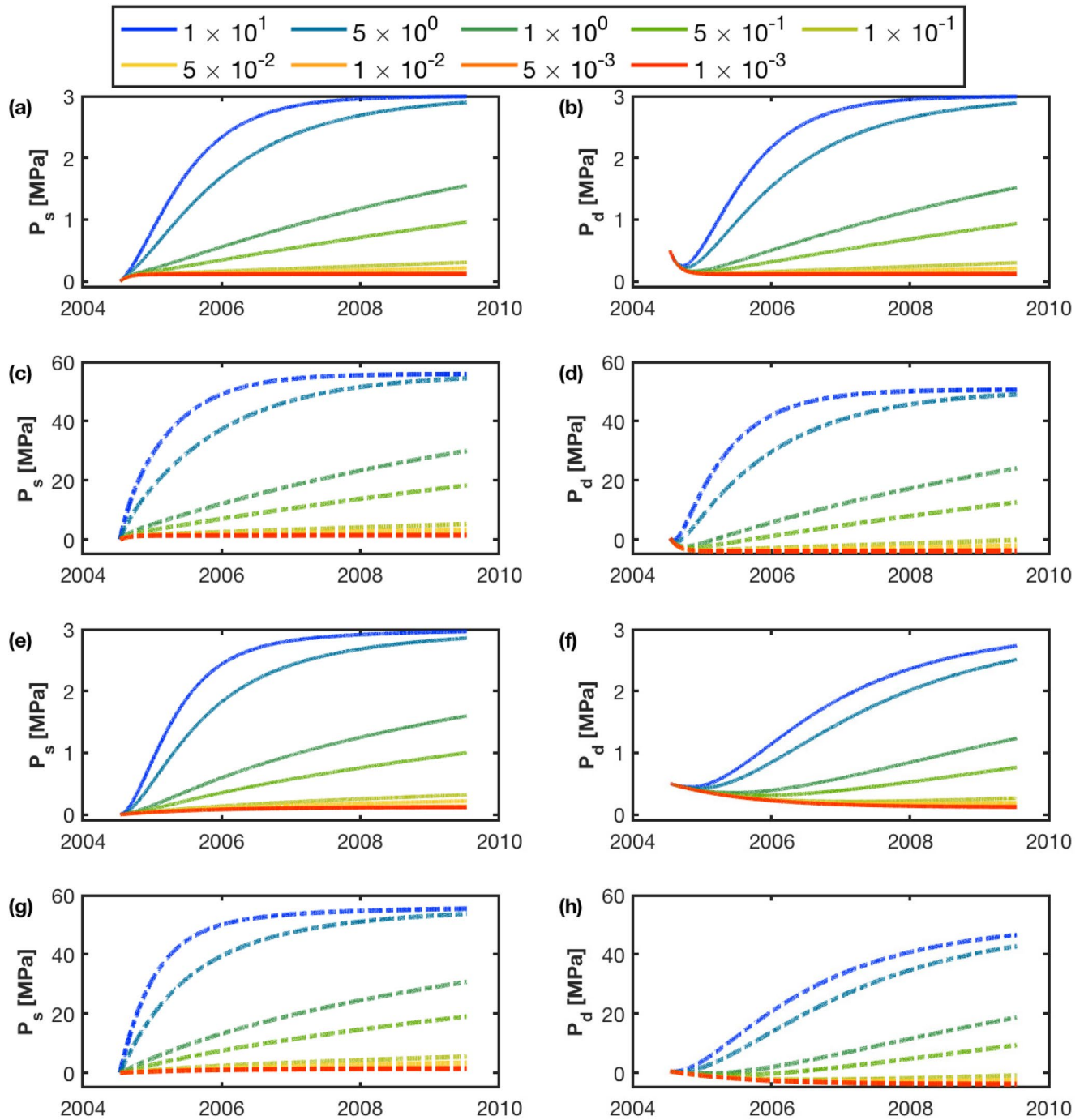
Figure 11. Same as Figure 10 but with P_{d0} = 0.5 MPa for the NGB sill. This simulation shows that magma extraction from NGB to the caldera can produce subsidence at NGB with a similar amplitude to that of the caldera uplift only if the NGB sill overpressure is unrealistically higher than the overpressure in the caldera sill.
