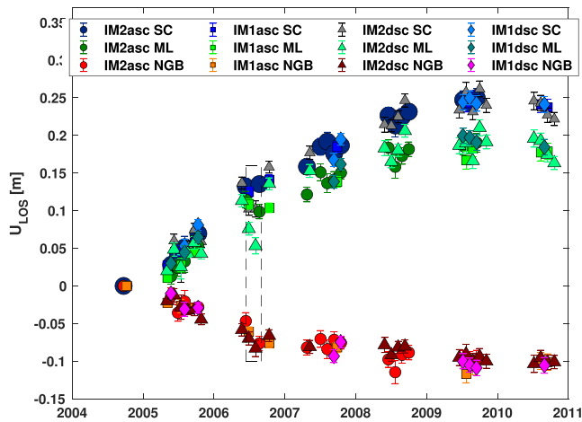
Figure 3. ENVISAT time series of line-of-sight deformation ( U_{LoS} ) for selected pixels of maximum displacement at SCD, MLD and NGB (Figure 2). The IM2dsc data show larger dispersion in the displacement because the interferograms used in the time series contain far more turbulent signals than any of the other three tracks (Supporting Information S1). The dashed box shows jumps in the IM2 descending time series not observed in other data sets. Using pairwise logic, these are not indicative of any ground deformation signal.
