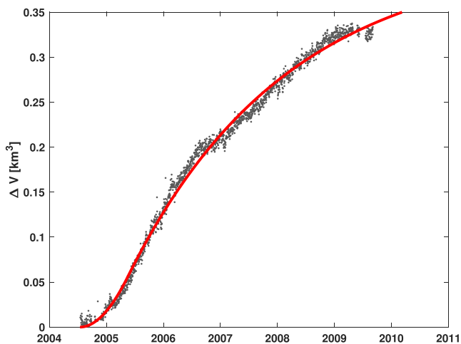
Figure 6. Time series of volume change ( \Delta V ) for the caldera source with uniform opening, and inverted from the vertical component ( U_z ) of all the GPS stations. The red line is the best-fit to Equation 1, but with P scaled to represent the source volume change.
