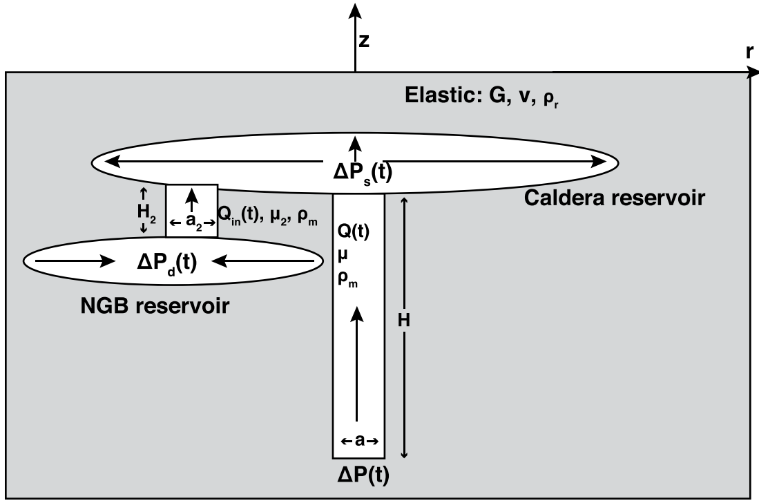
Figure 9. Sketch that shows the main physical parameters involved in the dynamic model of magma injection (Figure 10 and Equation 11). The model is made up of two reservoirs that are penny-shaped cracks, but vertically exaggerated in the figure. Here P_s and P_d represent the pressure in the caldera floor and NGB reservoirs which are hydraulically connected. Magma ascends from a mantle source to the caldera source, which is also filled by magma flowing from the NGB source. The model does not consider large areas of partial melt inferred from V_P tomography (Farrell et al., 2014; Huang et al., 2015) and how the melt can either bypass or interact with these areas.
