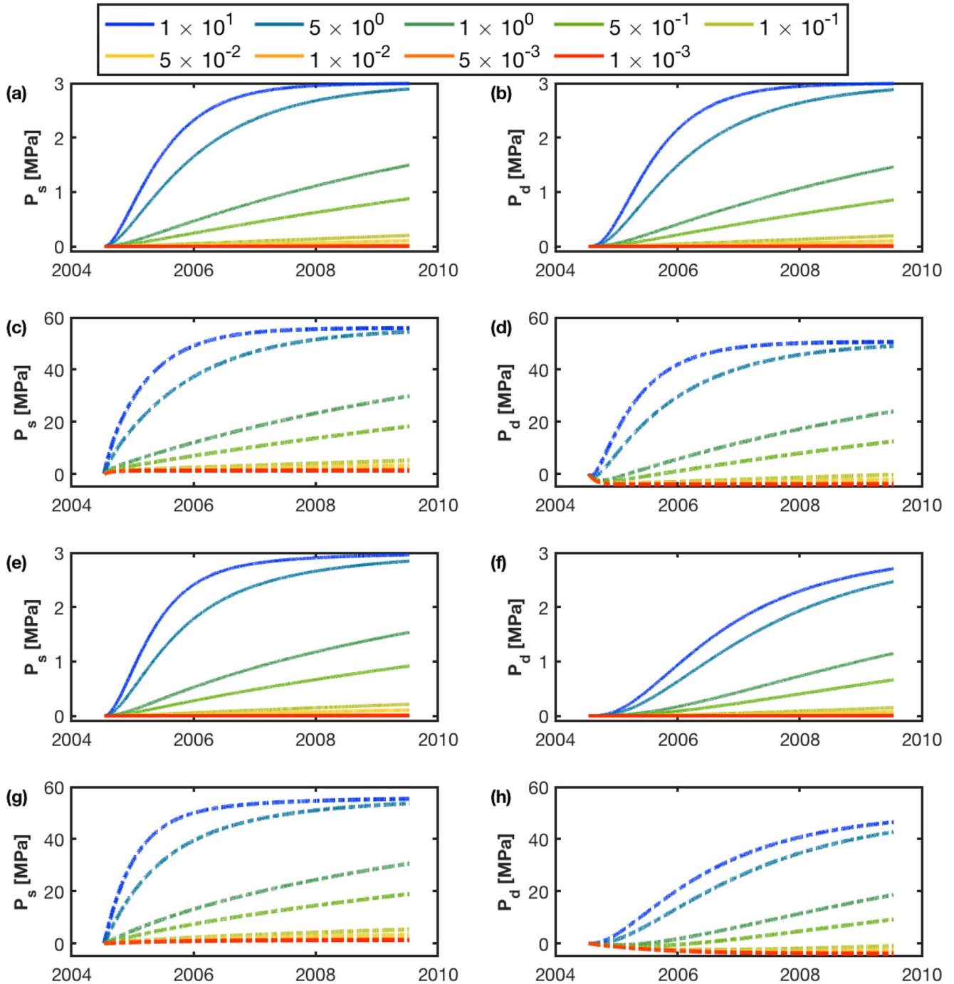
Figure 10. Simulation of the pressure change in the caldera source ( P_s , (a, c, e, and g)) and NGB ( P_d , (b, d, f, and h)) reservoirs based on the analytic model of magma transfer between the caldera floor and NGB (Equation 11) for the 2004–2009 time period, and with P_d^0 = 0.05 MPa for the NGB sill. Panels (a)–(b) show simulations with conduit flow due to magma overpressure while panels (c)–(d) show models with flow due to both magma overpressure and buoyancy. The colored lines show simulations for different conduit conductivities between the caldera sources and a deep mantle source. (a)–(d) and (e)–(h) show simulations for conduit conductivities of 1 and 0.1 between the caldera sill and the deeper NGB sill. Deformation due to magma injection is proportional to the source pressure change in a linear elastic half-space, so the ground deformation follows functions with the same shape as the source pressure function. The models show that magma extraction from NGB to the caldera floor cannot explain both the deformation trends observed in the GPS (Figure 1) and InSAR (Figure 3) data.
