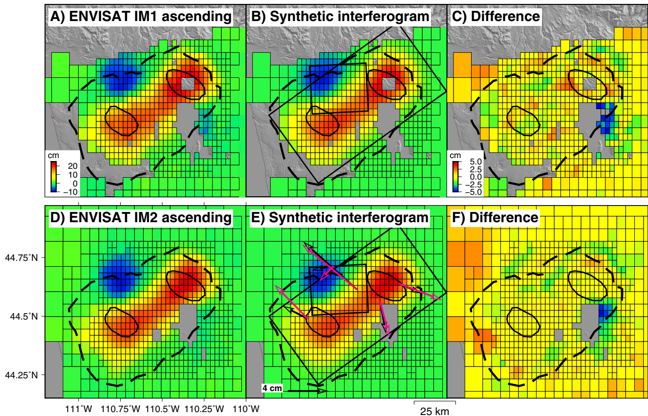
Figure 4. Downsampled (a), (d), synthetic (b), (e) and residual interferograms (c), (f) produced by a distributed opening sill below the caldera and by a closing sill below NG spanning 2004–2009. The black and pink arrows are the GPS data and synthetic data from the best-fit joint inversion. The rectangles are the modeled sills (Figure 5).
