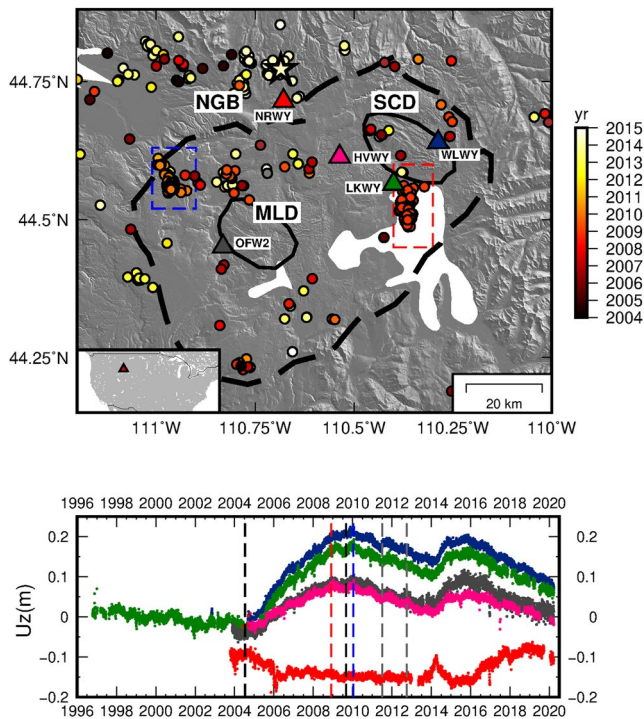
Figure 1. Top. Yellowstone caldera (thick dashed line), Mallard Lake (MLD) and Sour Creek (SCD) resurgent domes (black lines) draped over the 10 m shaded NED DEM. Triangles are GPS stations that recorded data during the complete episode of unrest in 2004–2009. The dots show earthquakes from the USGS Earthquake Catalog shallower than 15 km with M_L > 2.5 . The red and blue dashed rectangles show the December 2008 (Farrell et al., 2010) and January 2010 Madison Plateau (Shelly et al., 2013) seismic swarms. The star is the M_W 4.8 earthquake of March 30 2014 at NGB. Inset shows location of Yellowstone caldera (red triangle) within the United States. Bottom. GPS time series of vertical deformation (colored triangles on top). The dashed black and gray lines show the 2004–2009 episode of unrest, and the caldera subsidence covered by the TSX data during 2011–2012 respectively (Figure 2). The vertical red and blue lines show the December 2008 and January 2010 seismic swarms.
