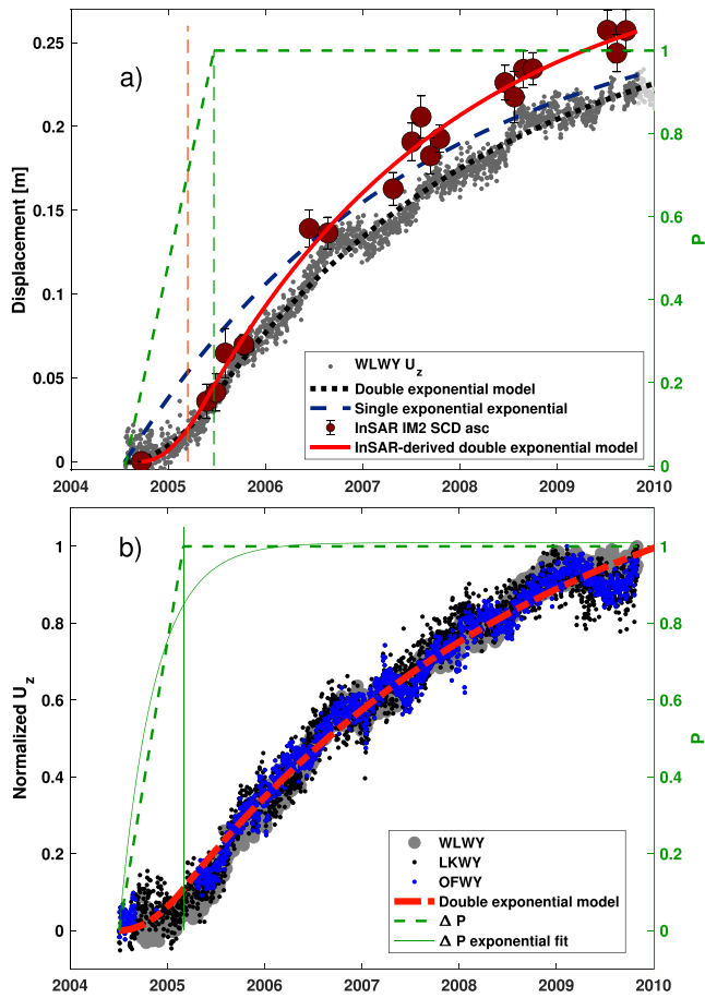
Figure 7. (a) Magma injection model fits to GPS (gray dots) and Interferometric Synthetic Aperture Radar (InSAR) (red circles) data. Displacement refers to either vertical displacement for GPS data or line-of-sight displacement for InSAR data. The red and black lines are the best-fit models to the InSAR IM2 for Sour Creek (SCD) and the vertical component of the WLWY station. The blue dashed line is the best-fit function U = U_f(1 - e^{-t/\tau}) with U_f the maximum displacement and \tau a time constant. The right axis shows the pressure P in the deep magma source. The vertical lines show the change in the deep magma pressure P between a linearly increasing pressure to a constant pressure (green line for GPS and orange line for InSAR). (b) Best-fit magma injection model (red line) to the normalized vertical displacements of the WLWY, LKWY and OFW2 stations. The dashed green line is the adimensional mantle pressure function ( P_s ), and the green continuous line is the best-fit exponential fit of the form P_s = P(1 - e^{-t/\tau_m}) . The latter function is used to simulate the magma flow between the caldera and NGB (Figure 10 and Figure 11). The vertical green lines in panels A and B do not agree with each other because in panel A the model is applied only to a single GPS station while in B it is applied to the normalized displacements of the three stations.
